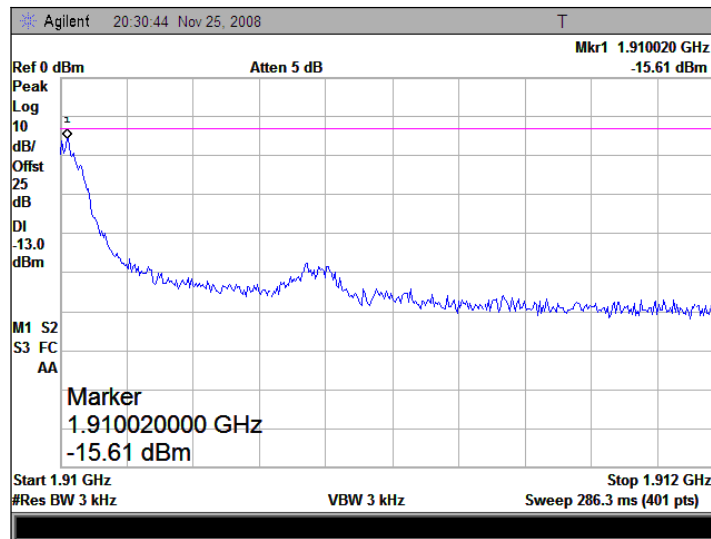
(Plot D: Channel = 810)
