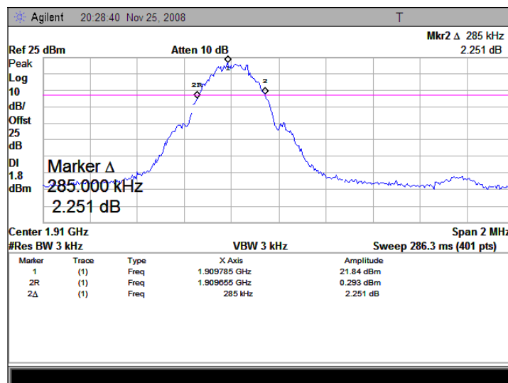
(Plot F: GSM 1900MHz Channel = 810)
