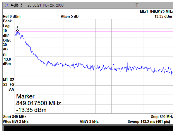
(Plot B: Channel = 251)
