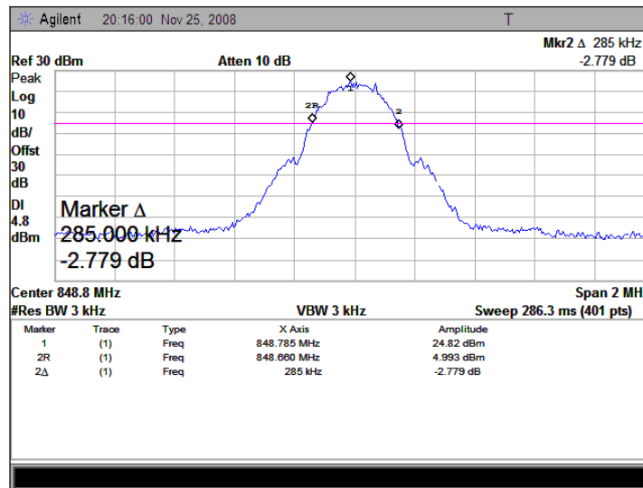
(Plot C: GSM 850MHz Channel = 251)
