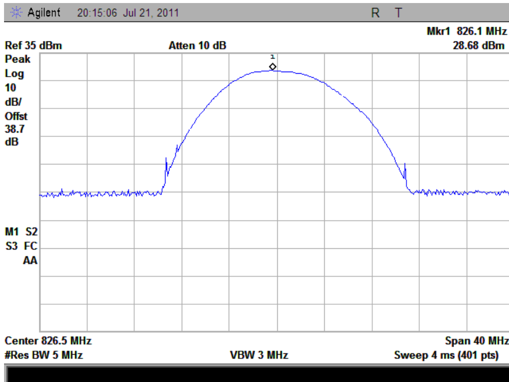
(WCDMA 850MHz Channel = 4132)
