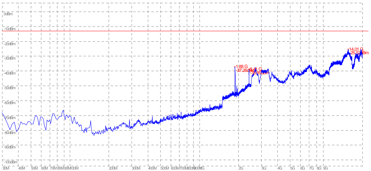
(Plot B.4: GSM 1900MHz Channel = 661, Test Antenna Vertical)
