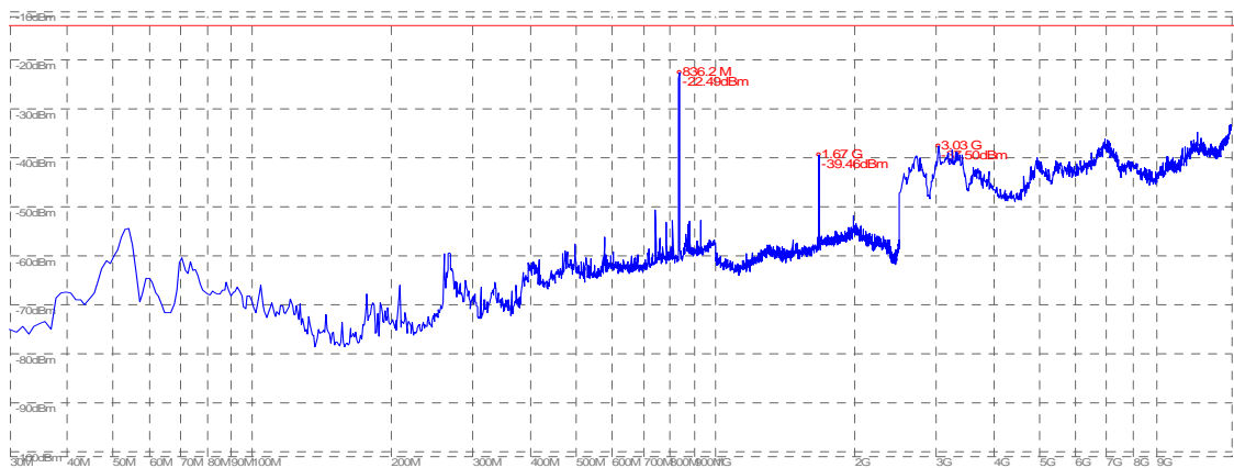
(Plot B.1: GSM 850MHz Channel = 190, Test Antenna Horizontal)
