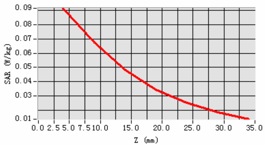
SAR, Z Axis Scan (X = -46, Y = -22)
