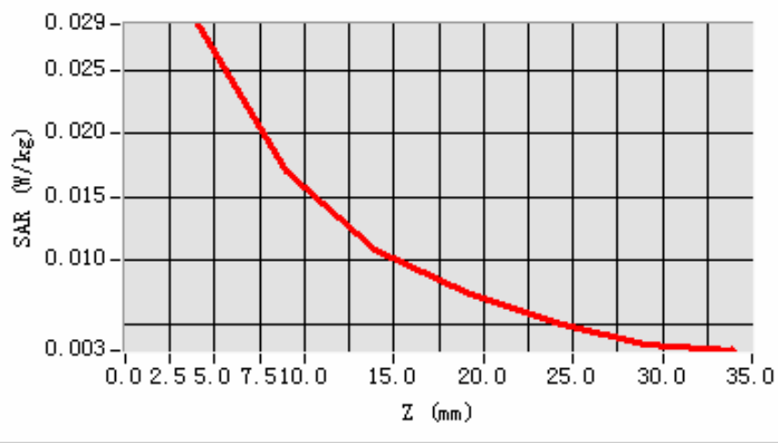
SAR, Z Axis Scan (X = 9, Y = 49)
