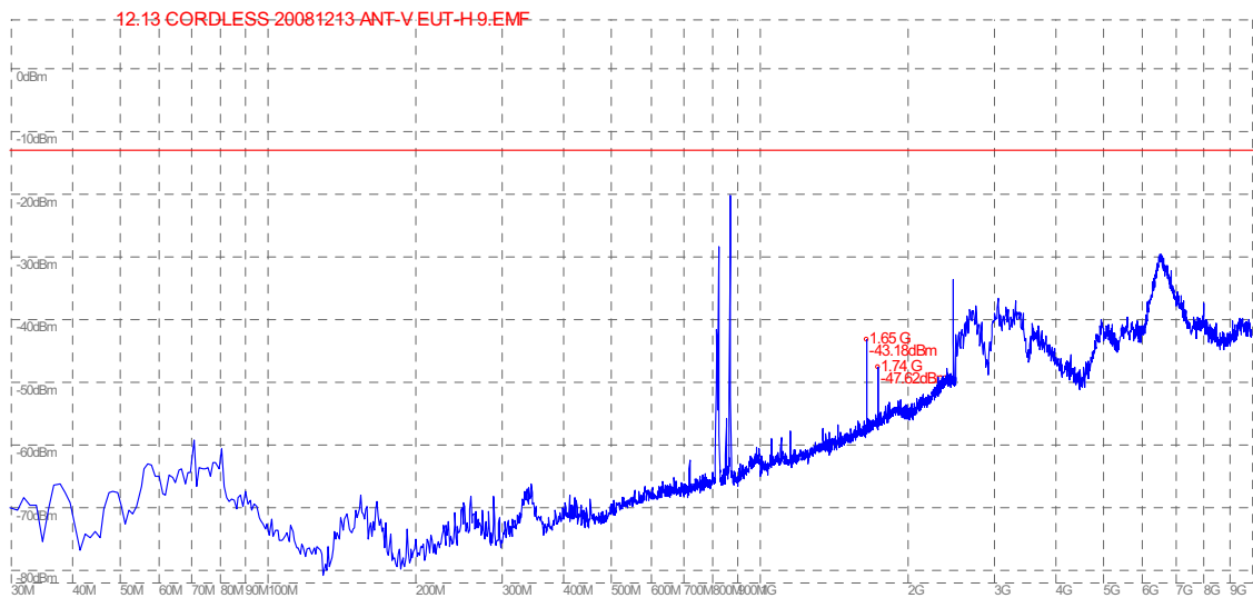
(Plot B: Test Antenna Vertical)
