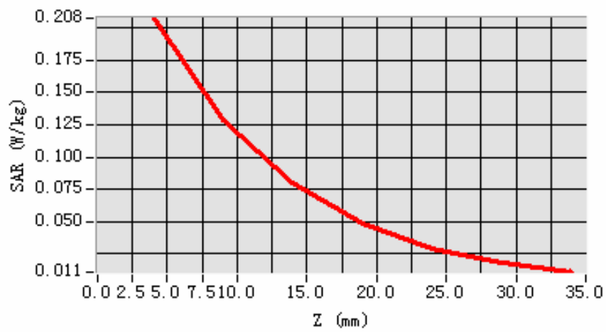
SAR, Z Axis Scan (X = -39, Y = -31)
