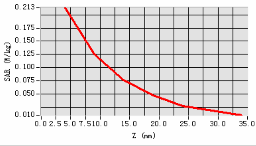
SAR, Z Axis Scan (X = -40, Y = -33)
