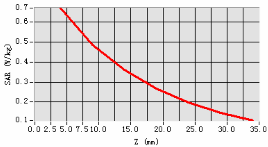
SAR, Z Axis Scan (X = -37, Y = -22)
