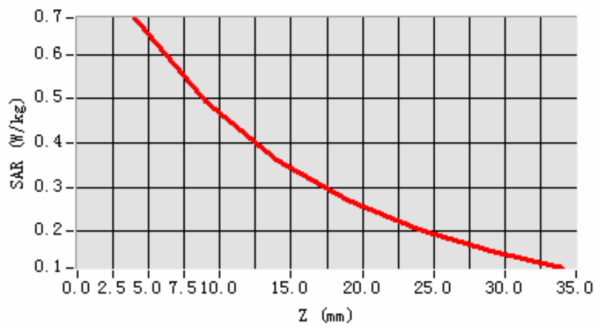
SAR, Z Axis Scan (X = -37, Y = -23)
