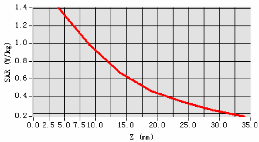
SAR, Z Axis Scan (X = -47, Y = -31)
