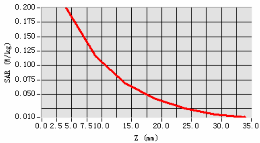
SAR, Z Axis Scan (X = -41, Y = -40)
