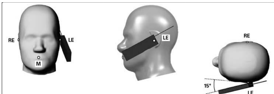
Fig 9.3 Illustration for Tilted Position
