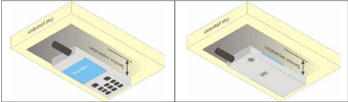
Fig 9.4 Illustration for Body Worn Position
