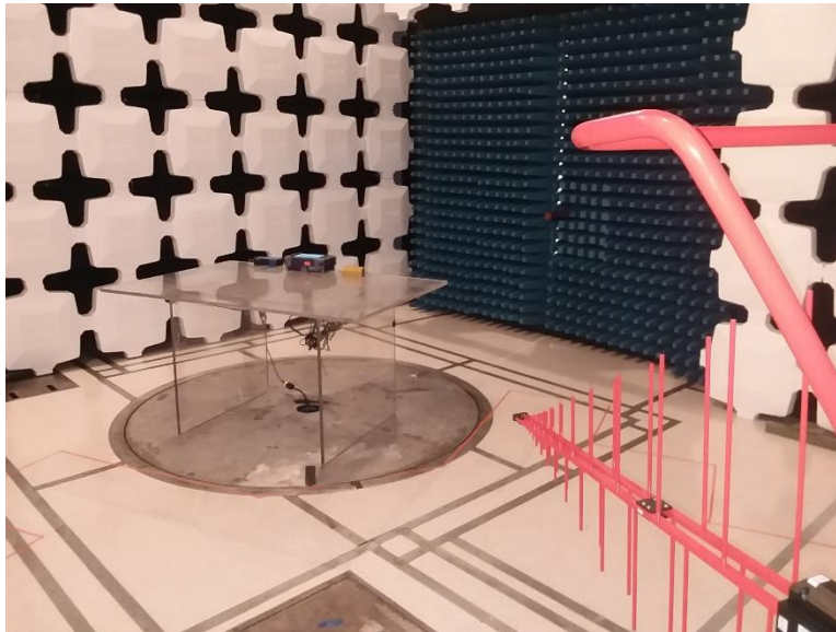
Figure 1: §15.407(b)(1) & (6 – 7) Undesirable Emissions, below 1GHz test setup
