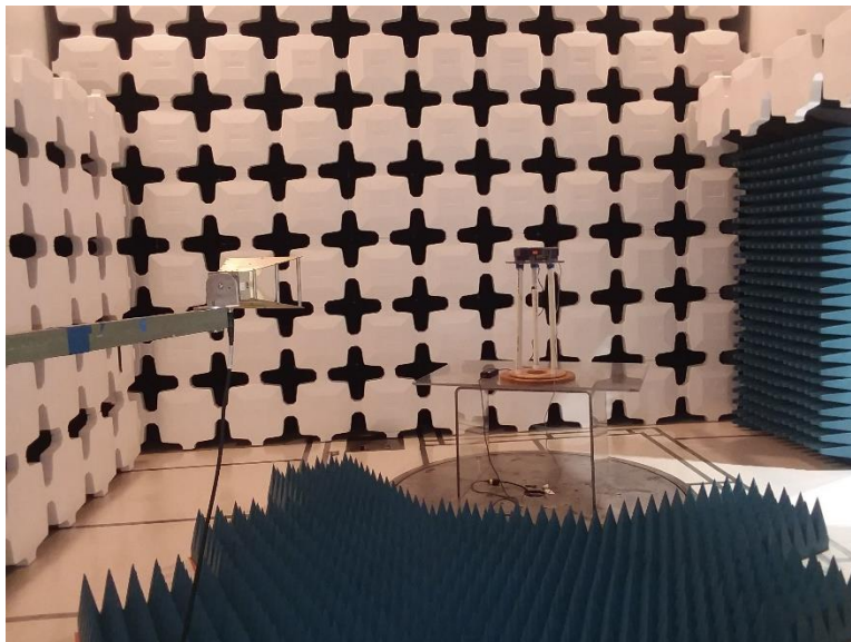
Figure 2: §15.407(b)(1) & (6 – 7) Undesirable Emissions, above 1GHz test setup
