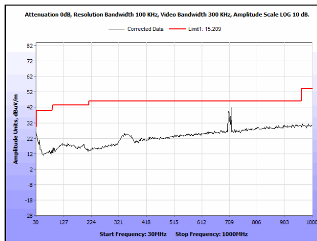
Plot 669. Radiated Spurious Emissions, 802.11ac 40 MHz, Channel 142, 1SS, 30 MHz – 1 GHz
