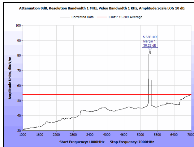
Plot 745. Radiated Spurious Emissions, 802.11ac 80 MH, Channel 106, 2SS, 1 GHz – 7 GHz, Average
