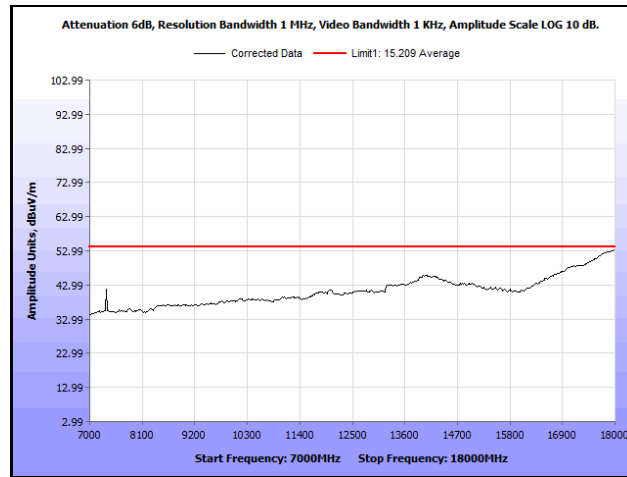
Plot 902. Radiated Spurious Emissions, 802.11n 40 MHz, Channel 110, 2SS, 7 GHz – 18 GHz, Average
