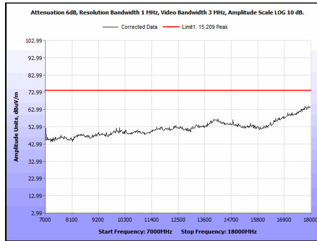
Plot 868. Radiated Spurious Emissions, 802.11n 40 MHz, Channel 62, 1SS, 7 GHz – 18 GHz, Peak
