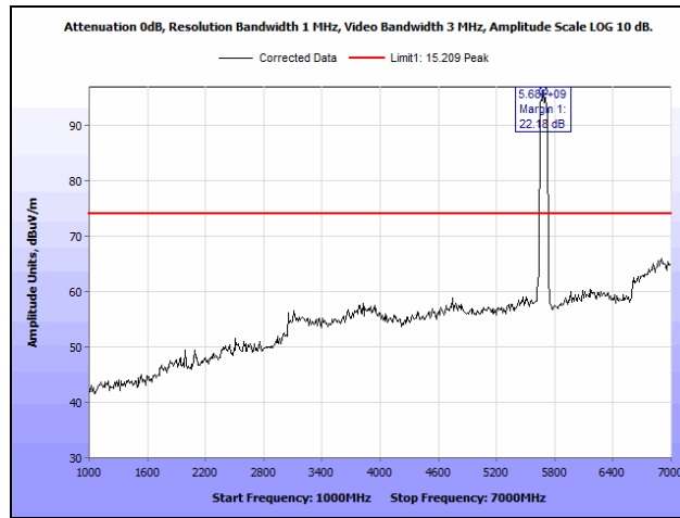
Plot 736. Radiated Spurious Emissions, 802.11ac 80 MHz, Channel 138, 1SS, 1 GHz – 7 GHz, Peak
