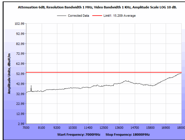
Plot 607. Radiated Spurious Emissions, 802.11ac 20 MH, Channel 100, 2SS, 7 GHz – 18 GHz, Average
