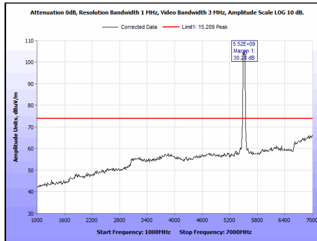
Plot 896. Radiated Spurious Emissions, 802.11n 40 MH, Channel 102, 2SS, 1 GHz – 7 GHz, Peak
