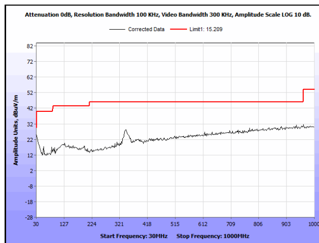
Plot 834. Radiated Spurious Emissions, 802.11n 20 MH, Channel 60, 3SS, 30 MHz – 1 GHz
