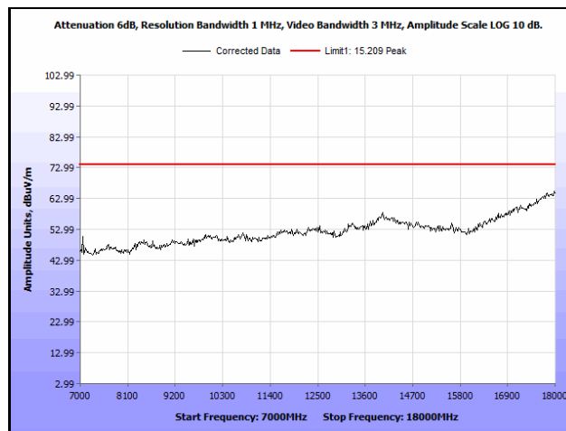
Plot 768. Radiated Spurious Emissions, 802.11ac 80 MH, Channel 138, 3SS, 7 GHz – 18 GHz, Peak
