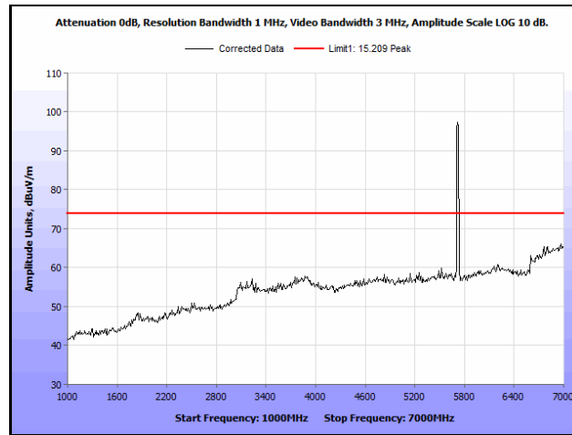
Plot 556. Radiated Spurious Emissions, 802.11a 20 MHz, Channel 144, 1 GHz – 7 GHz, Peak
