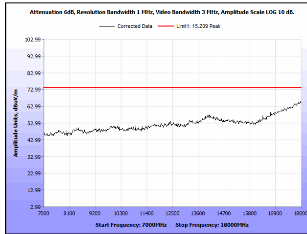
Plot 553. Radiated Spurious Emissions, 802.11a 20 MHz, Channel 116, 7 GHz – 18 GHz, Peak
