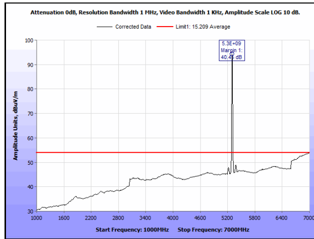
Plot 835. Radiated Spurious Emissions, 802.11n 20 MH, Channel 60, 3SS, 1 GHz – 7 GHz, Average
