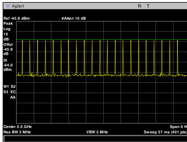
Plot 1025. Radar Waveform Calibration, Type 1, 5500 MHz
