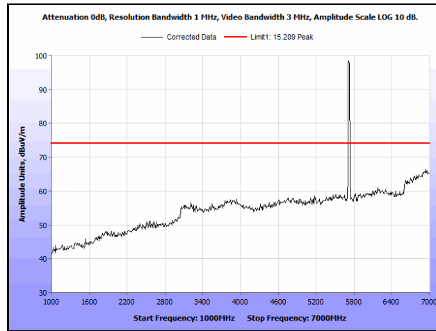
Plot 796. Radiated Spurious Emissions, 802.11n 20 MHz, Channel 144, 1SS, 1 GHz – 7 GHz, Peak
