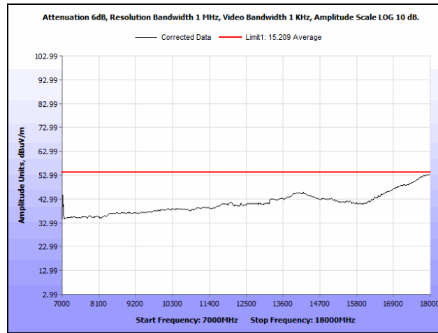
Plot 817. Radiated Spurious Emissions, 802.11n 20 MH, Channel 100, 2SS, 7 GHz – 18 GHz, Average
