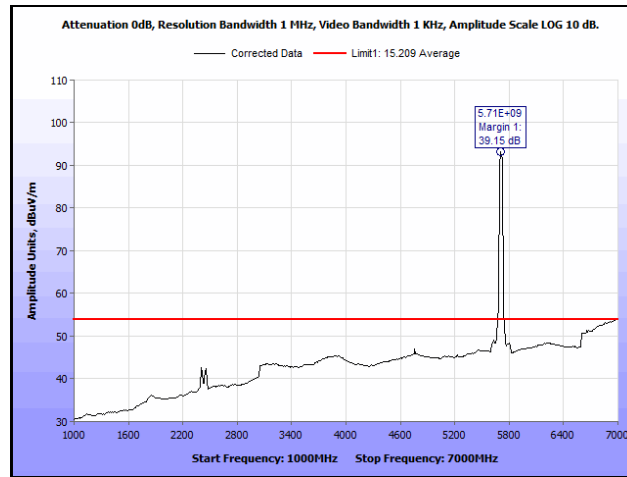
Plot 695. Radiated Spurious Emissions, 802.11ac 40 MHz, Channel 142, 2SS, 1 GHz – 7 GHz, Average
