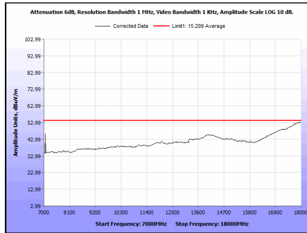
Plot 742. Radiated Spurious Emissions, 802.11ac 80 MHz, Channel 58, 2SS, 7 GHz – 18 GHz, Average
