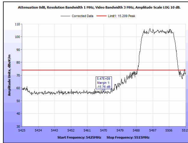
Plot 955. Radiated Band Edge, 802.11ac 20 MHz, 3SS, 5470 MHz, Peak
