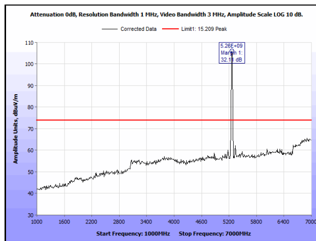
Plot 831. Radiated Spurious Emissions, 802.11n 20 MHz, Channel 52, 3SS, 1 GHz – 7 GHz, Peak
