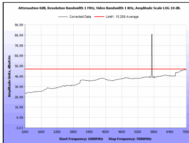
Plot 795. Radiated Spurious Emissions, 802.11n 20 MH, Channel 144, 1SS, 1 GHz – 7 GHz, Average
