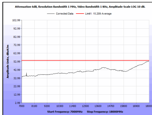
Plot 647. Radiated Spurious Emissions, 802.11ac 20 MH, Channel 144, 3SS, 7 GHz – 18 GHz, Average
