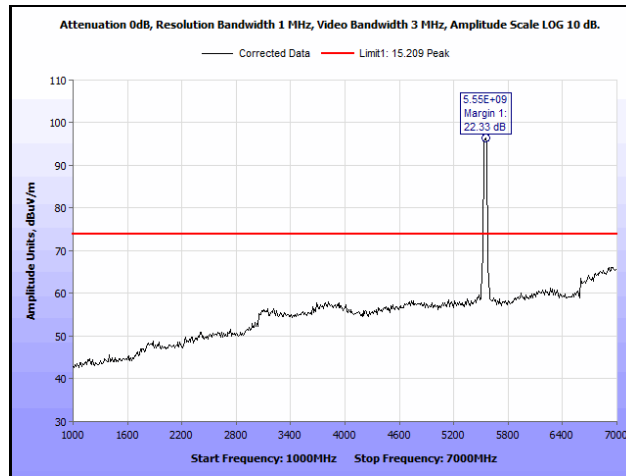
Plot 871. Radiated Spurious Emissions, 802.11n 40 MH, Channel 102, 1SS, 1 GHz – 7 GHz, Peak
