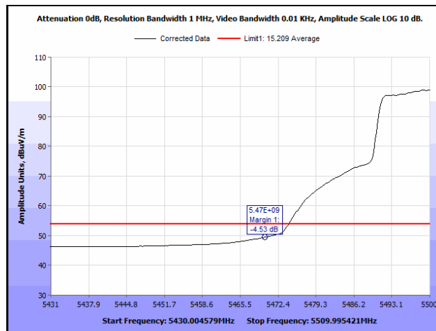
Plot 1002. Radiated Band Edge, 802.11n 20 MHz, 3SS, 5470 MHz, Average
