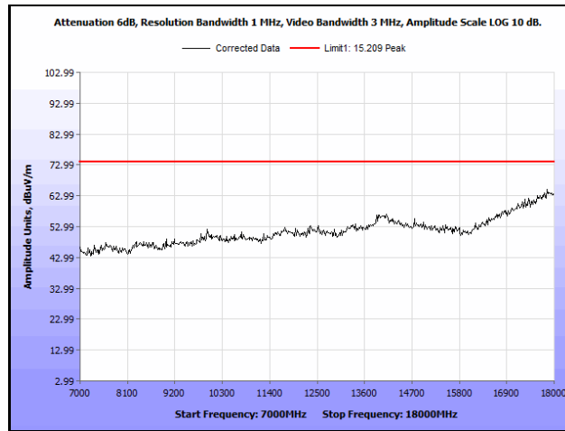
Plot 838. Radiated Spurious Emissions, 802.11n 20 MHz, Channel 60, 3SS, 7 GHz – 18 GHz, Peak
