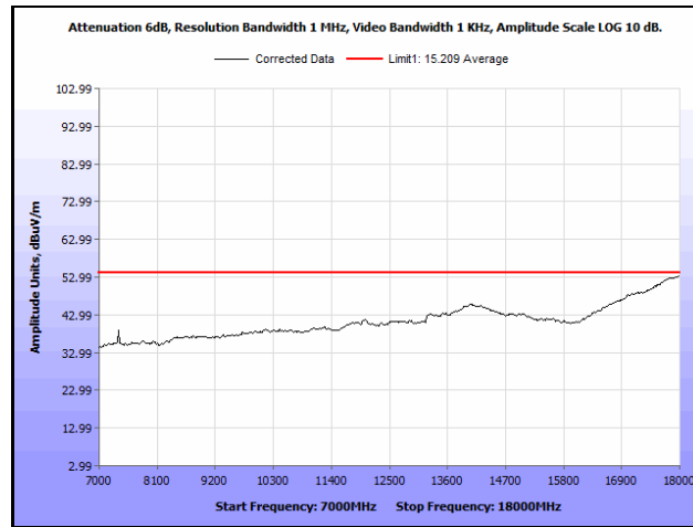
Plot 637. Radiated Spurious Emissions, 802.11ac 20 MH, Channel 100, 3SS, 7 GHz – 18 GHz, Average
