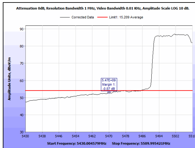
Plot 982. Radiated Band Edge, 802.11ac 80 MHz, 2SS, 5470 MHz, Average
