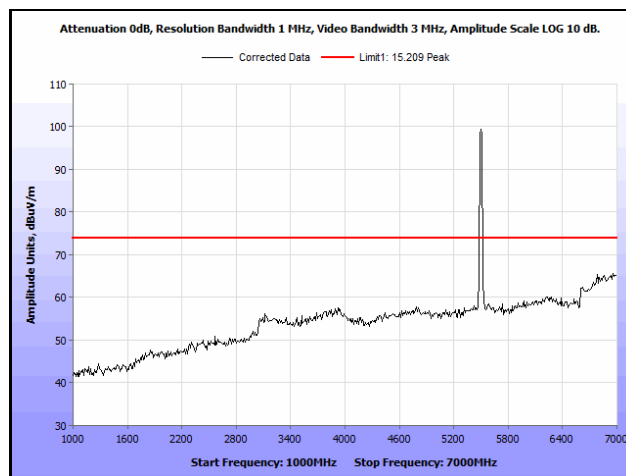
Plot 786. Radiated Spurious Emissions, 802.11n 20 MHz, Channel 100, 1SS, 1 GHz – 7 GHz, Peak
