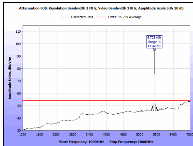
Plot 825. Radiated Spurious Emissions, 802.11n 20 MH, Channel 144, 2SS, 1 GHz – 7 GHz, Average
