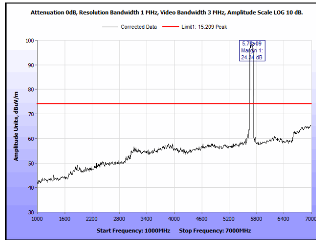
Plot 751. Radiated Spurious Emissions, 802.11ac 80 MH, Channel 138, 2SS, 1 GHz – 7 GHz, Peak
