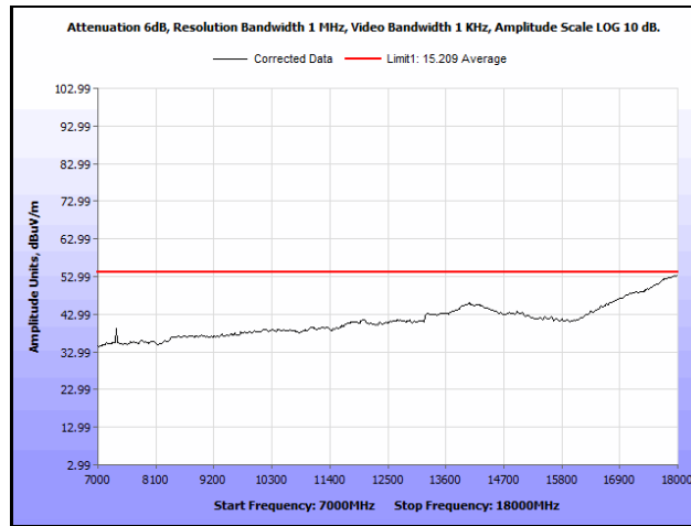
Plot 887. Radiated Spurious Emissions, 802.11n 40 MH, Channel 54, 2SS, 7 GHz – 18 GHz, Average
