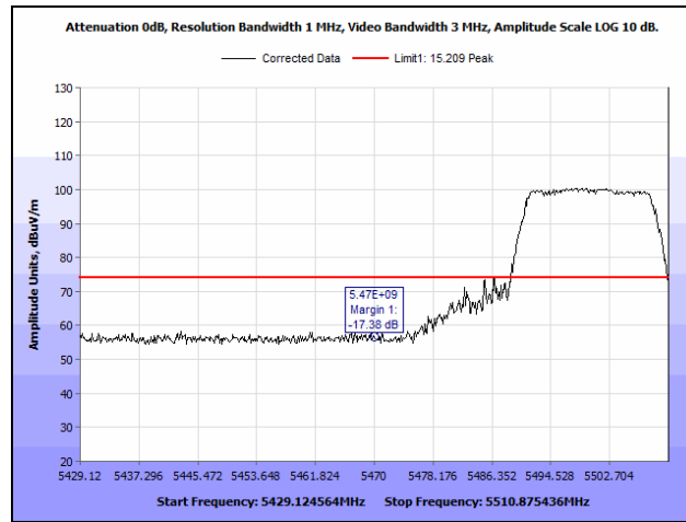
Plot 991. Radiated Band Edge, 802.11n 20 MHz, 1SS, 5470 MHz, Peak
