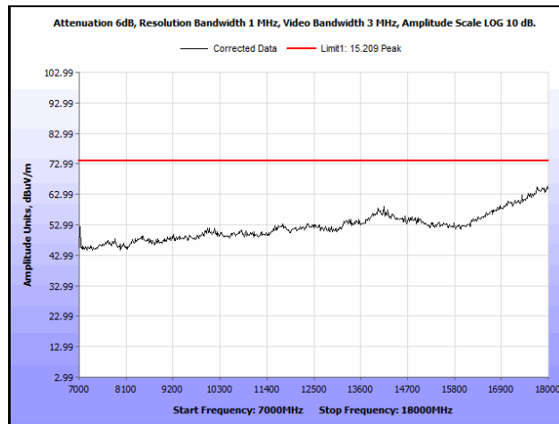
Plot 668. Radiated Spurious Emissions, 802.11ac 40 MHz, Channel 110, 1SS, 7 GHz – 18 GHz, Peak
