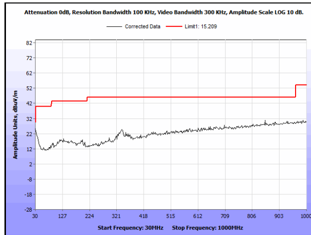
Plot 794. Radiated Spurious Emissions, 802.11n 20 MH, Channel 144, 1SS, 30 MHz – 1 GHz
