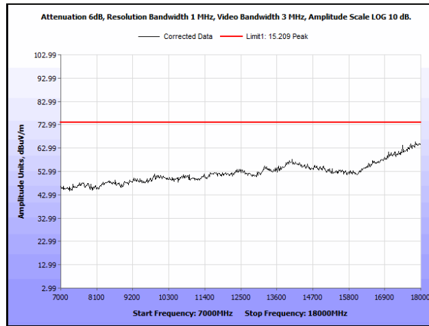
Plot 793. Radiated Spurious Emissions, 802.11n 20 MH, Channel 116, 1SS, 7 GHz – 18 GHz, Peak
