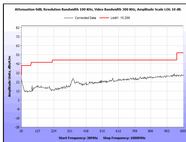
Plot 564. Radiated Spurious Emissions, 802.11ac 20 MH, Channel 60, 1SS, 30 MHz – 1 GHz
