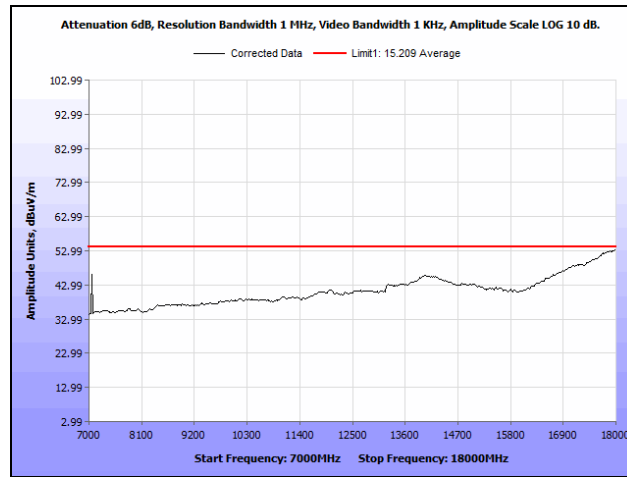
Plot 727. Radiated Spurious Emissions, 802.11ac 80 MHz, Channel 58, 1SS, 7 GHz – 18 GHz, Average
