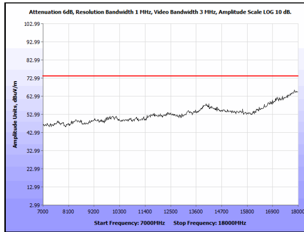
Plot 538. Radiated Spurious Emissions, 802.11a 20 MHz, Channel 60, 7 GHz – 18 GHz, Peak
