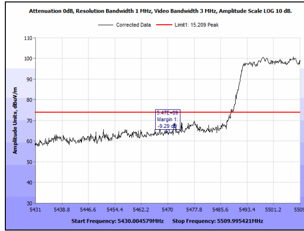
Plot 987. Radiated Band Edge, 802.11ac 80 MHz, 3SS, 5470 MHz, Peak
