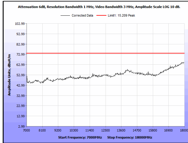
Plot 673. Radiated Spurious Emissions, 802.11ac 40 MH, Channel 142, 1SS, 7 GHz – 18 GHz, Peak
