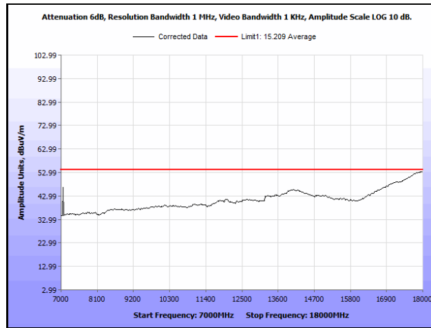
Plot 757. Radiated Spurious Emissions, 802.11ac 80 MHz, Channel 58, 3SS, 7 GHz – 18 GHz, Average
