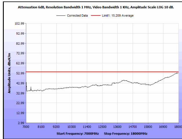
Plot 877. Radiated Spurious Emissions, 802.11n 40 MHz, Channel 110, 1SS, 7 GHz – 18 GHz, Average
