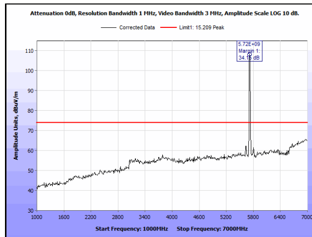
Plot 646. Radiated Spurious Emissions, 802.11ac 20 MH, Channel 144, 3SS, 1 GHz – 7 GHz, Peak
