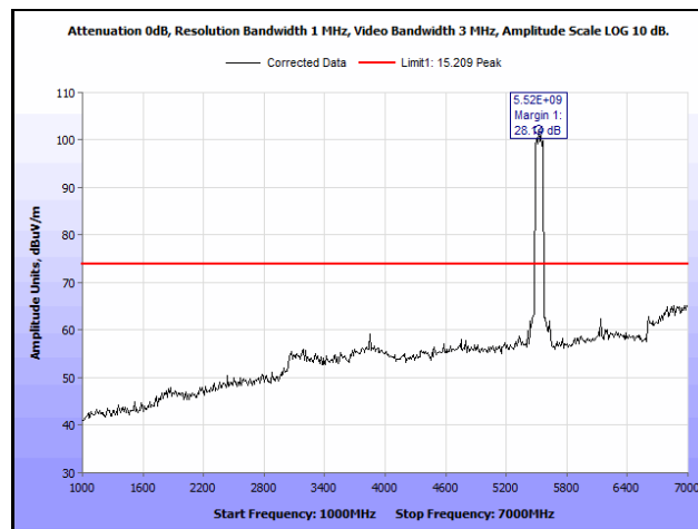
Plot 746. Radiated Spurious Emissions, 802.11ac 80 MH, Channel 106, 2SS, 1 GHz – 7 GHz, Peak
