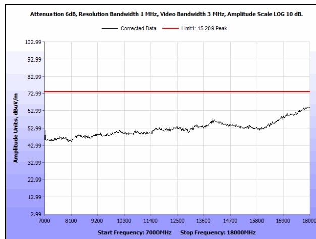
Plot 898. Radiated Spurious Emissions, 802.11n 40 MH, Channel 102, 2SS, 7 GHz – 18 GHz, Peak
