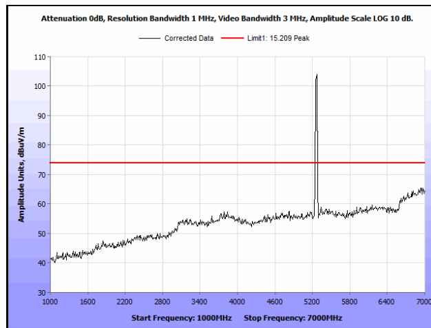
Plot 591. Radiated Spurious Emissions, 802.11ac 20 MHz, Channel 52, 2SS, 1 GHz – 7 GHz, Peak
