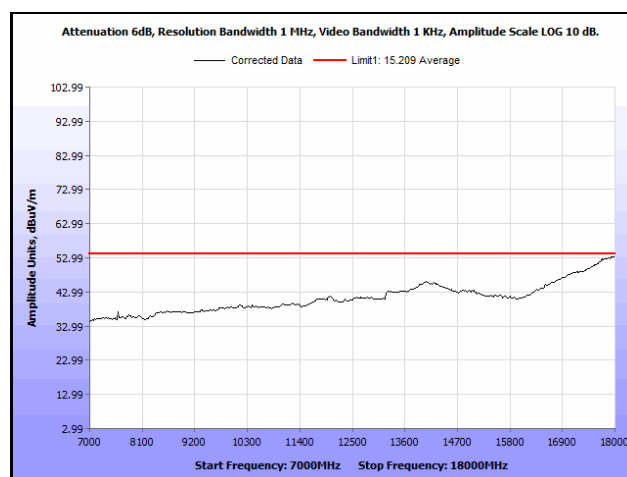
Plot 747. Radiated Spurious Emissions, 802.11ac 80 MH, Channel 106, 2SS, 7 GHz – 18 GHz, Average
