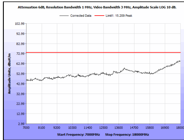
Plot 628. Radiated Spurious Emissions, 802.11ac 20 MHz, Channel 60, 3SS, 7 GHz – 18 GHz, Peak
