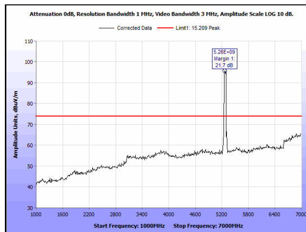
Plot 886. Radiated Spurious Emissions, 802.11n 40 MHz, Channel 54, 2SS, 1 GHz – 7 GHz, Peak
