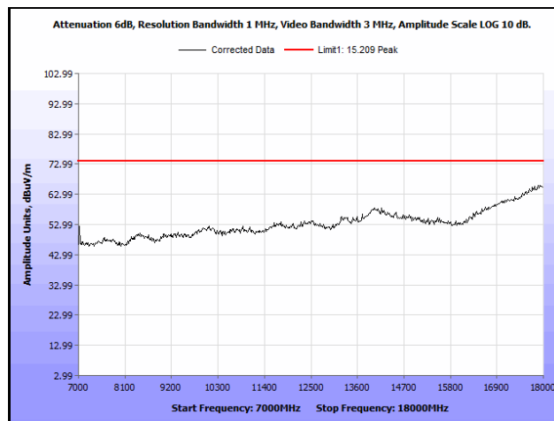
Plot 663. Radiated Spurious Emissions, 802.11ac 40 MHz, Channel 102, 1SS, 7 GHz – 18 GHz, Peak
