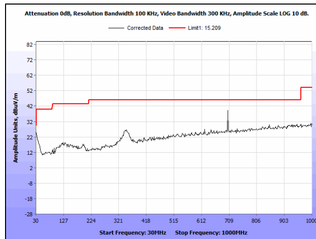
Plot 734. Radiated Spurious Emissions, 802.11ac 80 MH, Channel 138, 1SS, 30 MHz – 1 GHz
