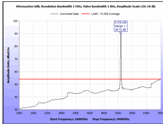
Plot 655. Radiated Spurious Emissions, 802.11ac 40 MHz, Channel 62, 1SS, 1 GHz – 7 GHz, Average
