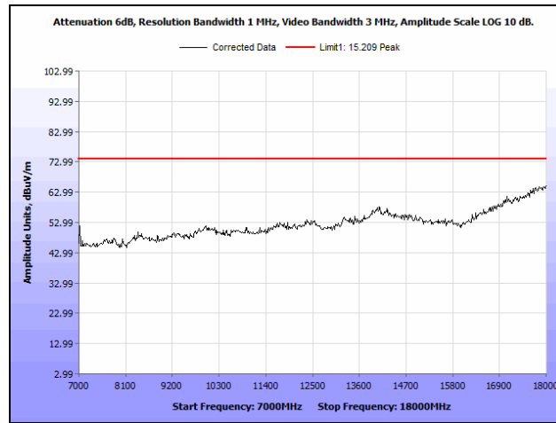
Plot 933. Radiated Spurious Emissions, 802.11n 40 MH, Channel 142, 3SS, 7 GHz – 18 GHz, Peak
