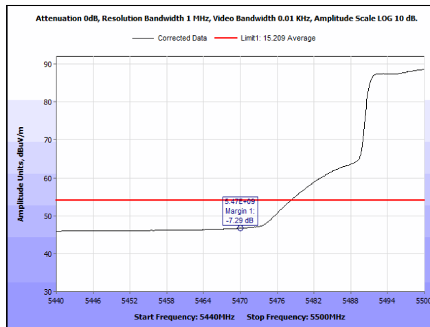
Plot 990. Radiated Band Edge, 802.11n 20 MHz, 1SS, 5470 MHz, Average
