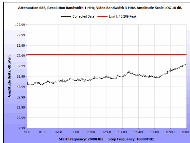
Plot 873. Radiated Spurious Emissions, 802.11n 40 MH, Channel 102, 1SS, 7 GHz – 18 GHz, Peak
