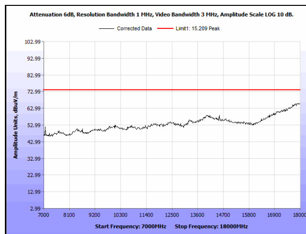
Plot 753. Radiated Spurious Emissions, 802.11ac 80 MH, Channel 138, 2SS, 7 GHz – 18 GHz, Peak
