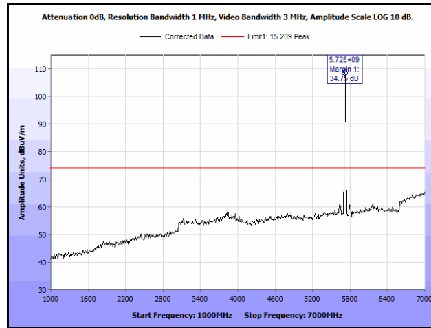
Plot 616. Radiated Spurious Emissions, 802.11ac 20 MHz, Channel 144, 2SS, 1 GHz – 7 GHz, Peak
