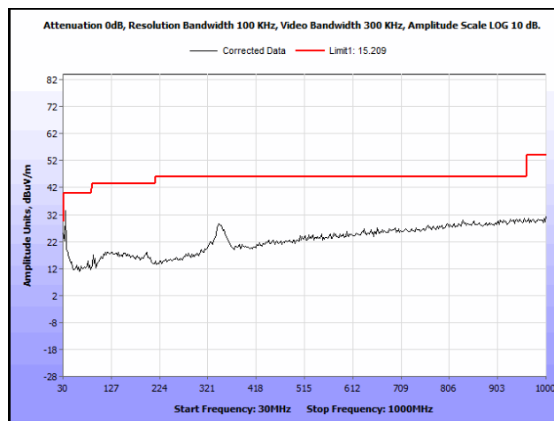
Plot 759. Radiated Spurious Emissions, 802.11ac 80 MHz, Channel 106, 3SS, 30 MHz – 1 GHz
