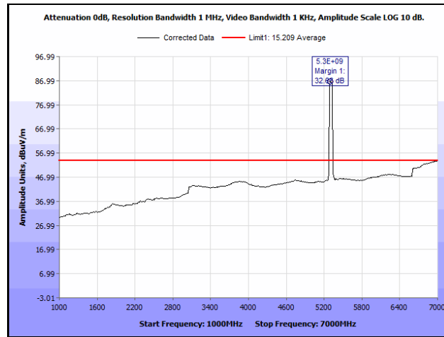
Plot 865. Radiated Spurious Emissions, 802.11n 40 MH, Channel 62, 1SS, 1 GHz – 7 GHz, Average
