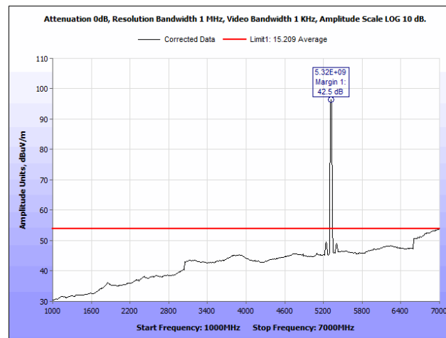
Plot 630. Radiated Spurious Emissions, 802.11ac 20 MHz, Channel 64, 3SS, 1 GHz – 7 GHz, Average
