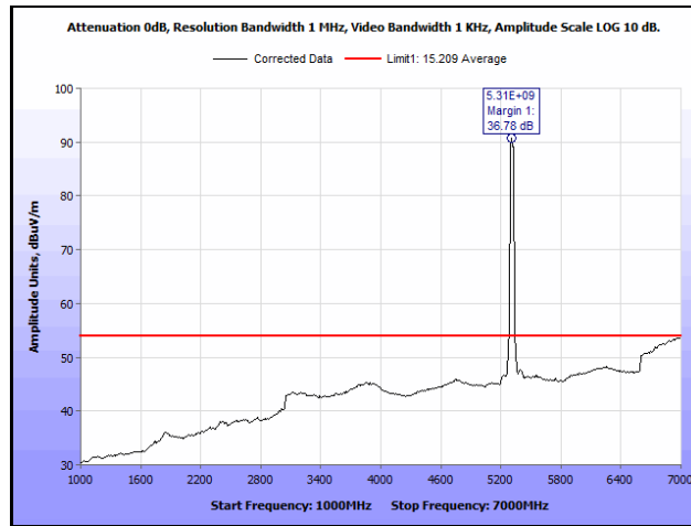
Plot 705. Radiated Spurious Emissions, 802.11ac 40 MHz, Channel 62, 3SS, 1 GHz – 7 GHz, Average
