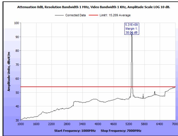
Plot 890. Radiated Spurious Emissions, 802.11n 40 MH, Channel 62, 2SS, 1 GHz – 7 GHz, Average
