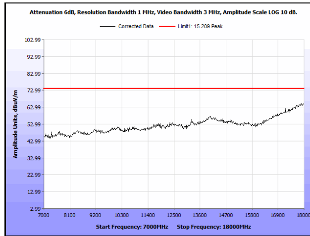
Plot 643. Radiated Spurious Emissions, 802.11ac 20 MHz, Channel 116, 3SS, 7 GHz – 18 GHz, Peak
