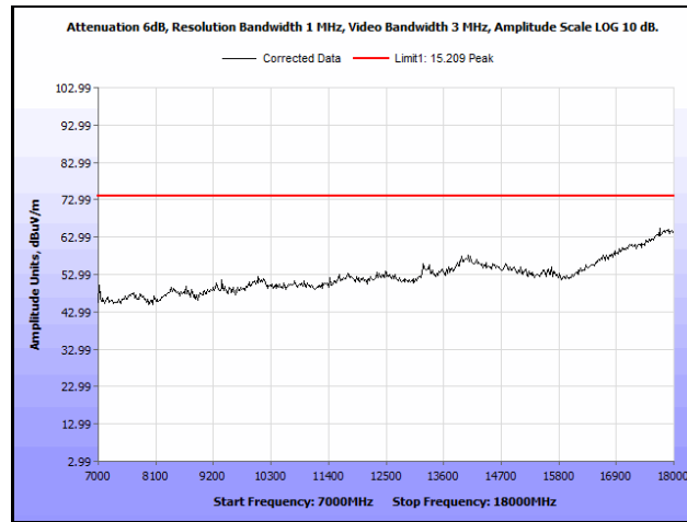
Plot 658. Radiated Spurious Emissions, 802.11ac 40 MHz, Channel 62, 1SS, 7 GHz – 18 GHz, Peak
