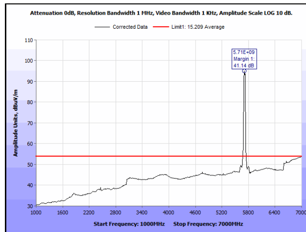
Plot 905. Radiated Spurious Emissions, 802.11n 40 MH, Channel 142, 2SS, 1 GHz – 7 GHz, Average
