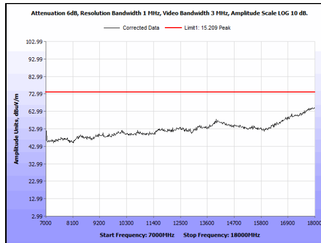
Plot 903. Radiated Spurious Emissions, 802.11n 40 MHz, Channel 110, 2SS, 7 GHz – 18 GHz, Peak
