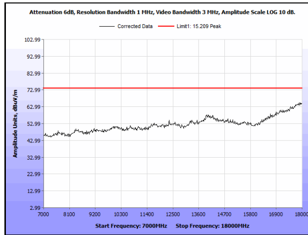
Plot 778. Radiated Spurious Emissions, 802.11n 20 MH, Channel 60, 1SS, 7 GHz – 18 GHz, Peak
