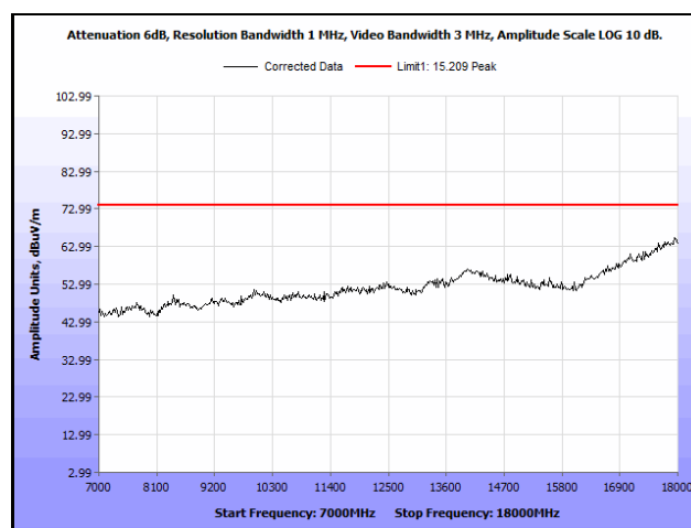
Plot 648. Radiated Spurious Emissions, 802.11ac 20 MH, Channel 144, 3SS, 7 GHz – 18 GHz, Peak
