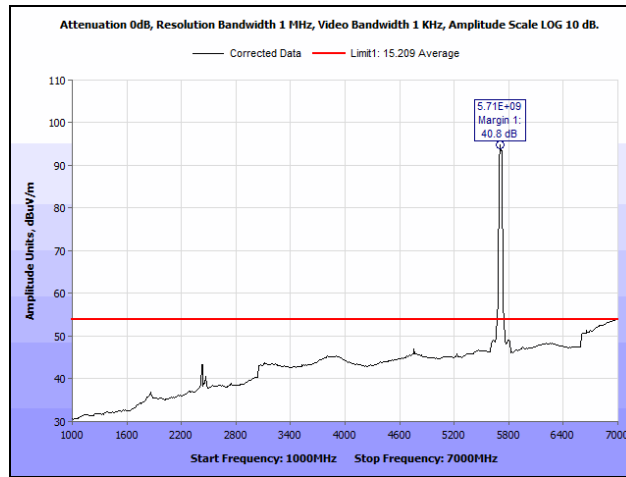
Plot 930. Radiated Spurious Emissions, 802.11n 40 MH, Channel 142, 3SS, 1 GHz – 7 GHz, Average
