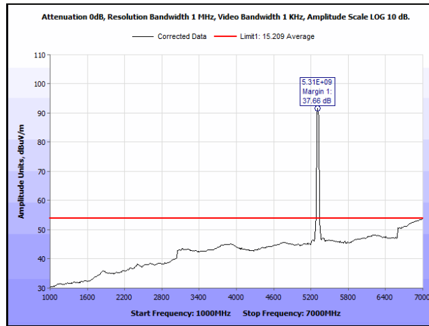
Plot 915. Radiated Spurious Emissions, 802.11n 40 MH, Channel 62, 3SS, 1 GHz – 7 GHz, Average
