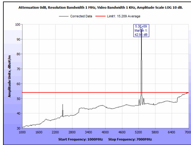
Plot 805. Radiated Spurious Emissions, 802.11n 20 MH, Channel 60, 2SS, 1 GHz – 7 GHz, Average
