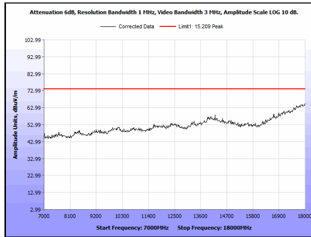
Plot 568. Radiated Spurious Emissions, 802.11ac 20 MHz, Channel 60, 1SS, 7 GHz – 18 GHz, Peak
