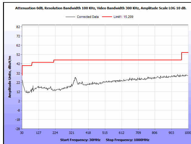
Plot 879. Radiated Spurious Emissions, 802.11n 40 MHz, Channel 142, 1SS, 30 MHz – 1 GHz
