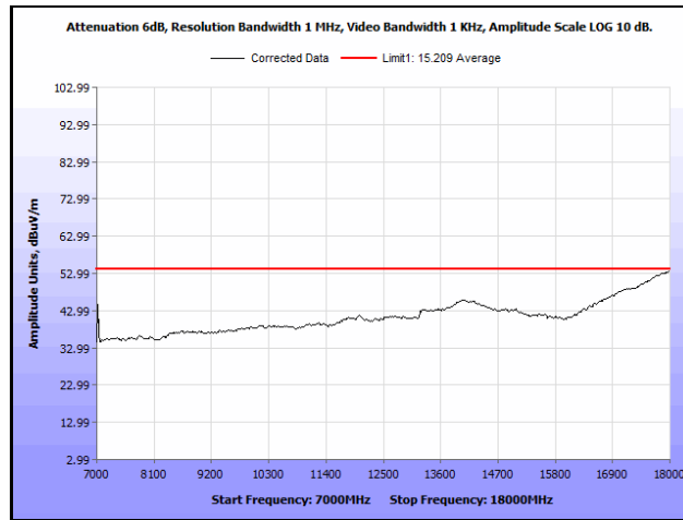
Plot 677. Radiated Spurious Emissions, 802.11ac 40 MHz, Channel 54, 2SS, 7 GHz – 18 GHz, Average
