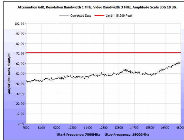
Plot 823. Radiated Spurious Emissions, 802.11n 20 MH, Channel 116, 2SS, 7 GHz – 18 GHz, Peak
