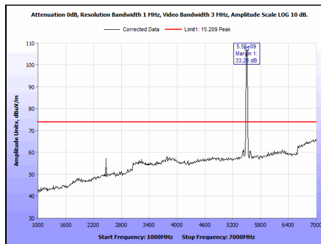
Plot 576. Radiated Spurious Emissions, 802.11ac 20 MHz, Channel 100, 1SS, 1 GHz – 7 GHz, Peak
