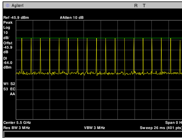
Plot 1024. Radar Waveform Calibration, Type 0, 5500 MHz
