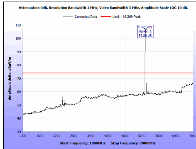
Plot 631. Radiated Spurious Emissions, 802.11ac 20 MHz, Channel 64, 3SS, 1 GHz – 7 GHz, Peak
