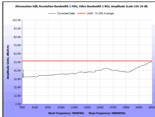
Plot 842. Radiated Spurious Emissions, 802.11n 20 MHz, Channel 64, 3SS, 7 GHz – 18 GHz, Average
