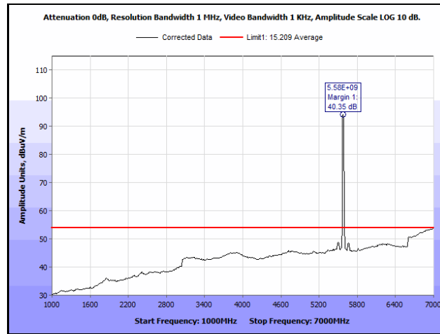
Plot 640. Radiated Spurious Emissions, 802.11ac 20 MHz, Channel 116, 3SS, 1 GHz – 7 GHz, Average
