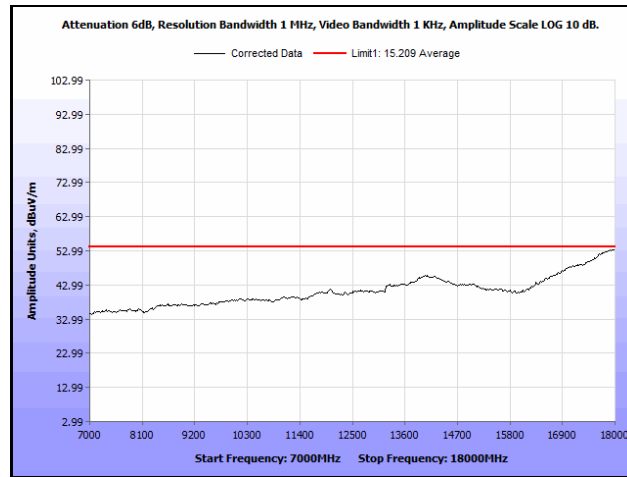
Plot 692. Radiated Spurious Emissions, 802.11ac 40 MH, Channel 110, 2SS, 7 GHz – 18 GHz, Average
