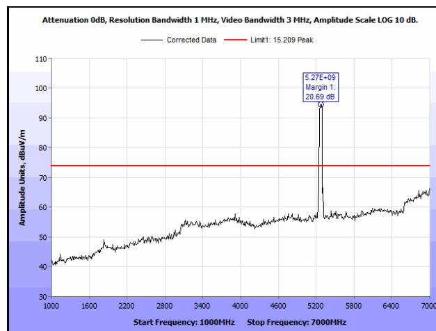
Plot 861. Radiated Spurious Emissions, 802.11n 40 MHz, Channel 54, 1SS, 1 GHz – 7 GHz, Peak
