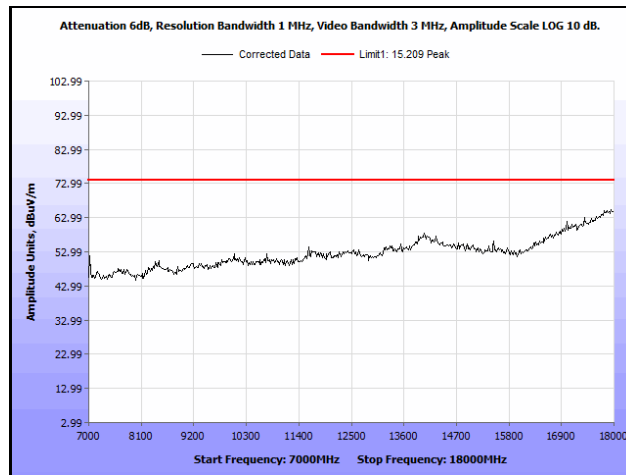
Plot 678. Radiated Spurious Emissions, 802.11ac 40 MHz, Channel 54, 2SS, 7 GHz – 18 GHz, Peak
