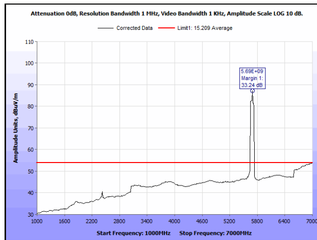
Plot 765. Radiated Spurious Emissions, 802.11ac 80 MH, Channel 138, 3SS, 1 GHz – 7 GHz, Average
