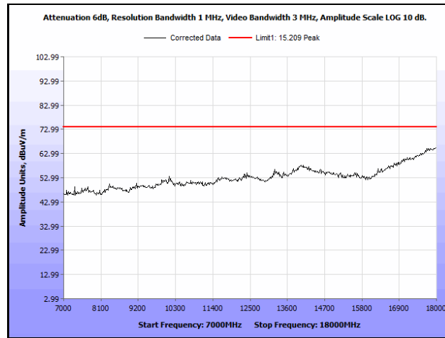
Plot 853. Radiated Spurious Emissions, 802.11n 20 MHz, Channel 116, 3SS, 7 GHz – 18 GHz, Peak
