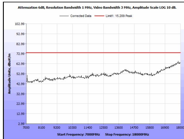
Plot 743. Radiated Spurious Emissions, 802.11ac 80 MHz, Channel 58, 2SS, 7 GHz – 18 GHz, Peak
