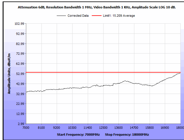
Plot 667. Radiated Spurious Emissions, 802.11ac 40 MHz, Channel 110, 1SS, 7 GHz – 18 GHz, Average
