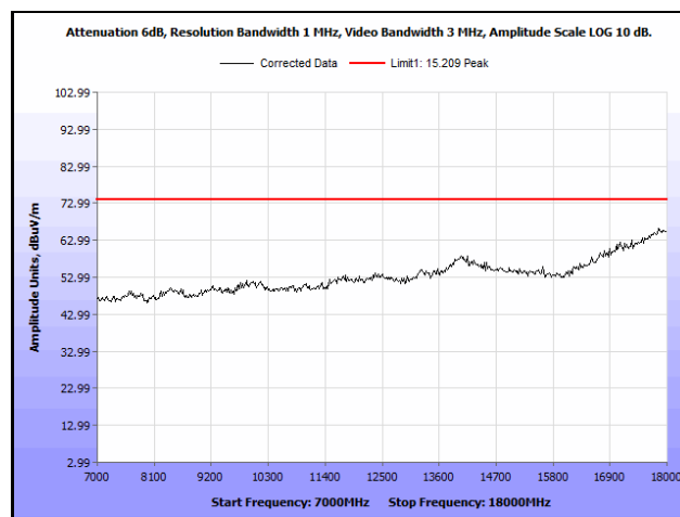
Plot 543. Radiated Spurious Emissions, 802.11a 20 MHz, Channel 64, 7 GHz – 18 GHz, Peak
