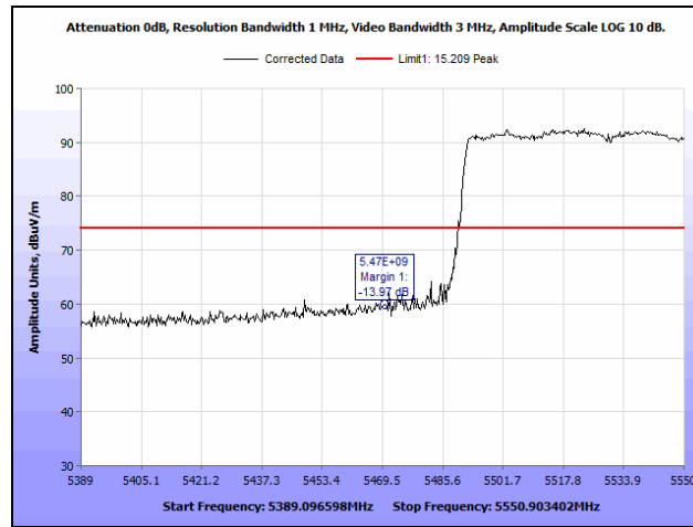
Plot 979. Radiated Band Edge, 802.11ac 80 MHz, 1SS, 5470 MHz, Peak
