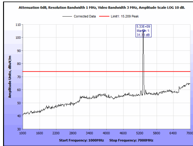
Plot 571. Radiated Spurious Emissions, 802.11ac 20 MH, Channel 64, 1SS, 1 GHz – 7 GHz, Peak
