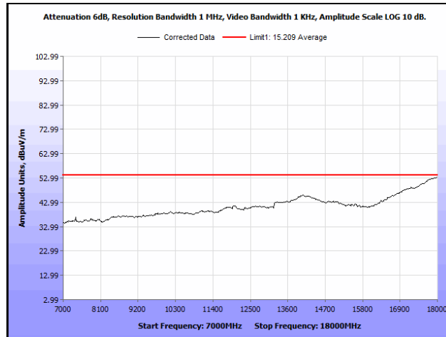
Plot 767. Radiated Spurious Emissions, 802.11ac 80 MH, Channel 138, 3SS, 7 GHz – 18 GHz, Average
