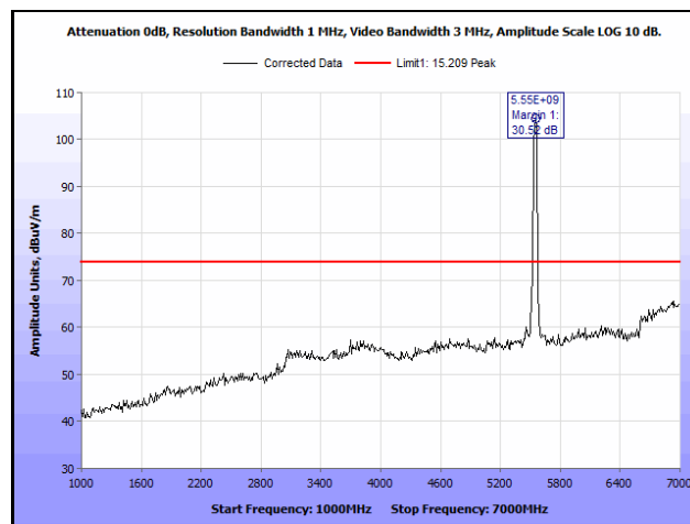
Plot 926. Radiated Spurious Emissions, 802.11n 40 MHz, Channel 110, 3SS, 1 GHz – 7 GHz, Peak
