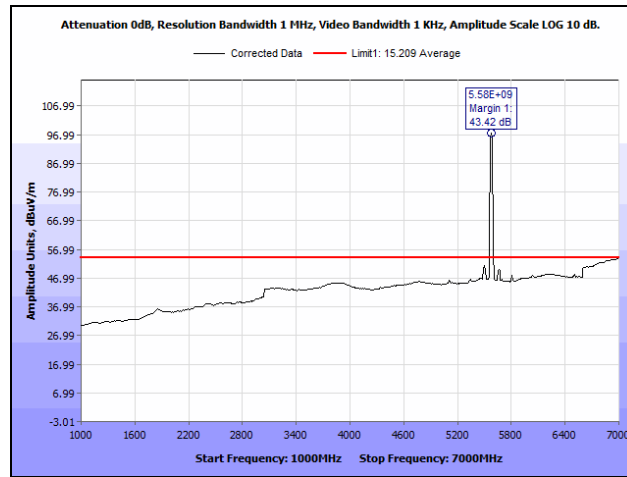
Plot 820. Radiated Spurious Emissions, 802.11n 20 MH, Channel 116, 2SS, 1 GHz – 7 GHz, Average
