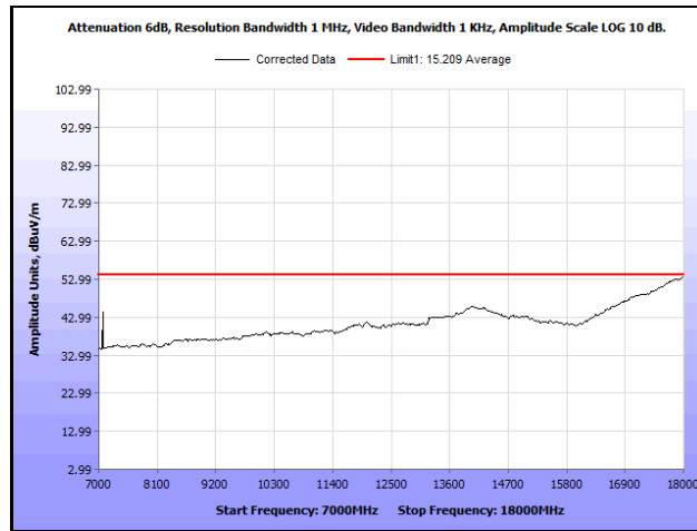
Plot 592. Radiated Spurious Emissions, 802.11ac 20 MH, Channel 52, 2SS, 7 GHz – 18 GHz, Average
