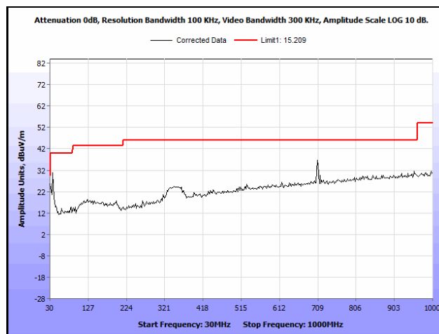
Plot 679. Radiated Spurious Emissions, 802.11ac 40 MHz, Channel 62, 2SS, 30 MHz – 1 GHz
