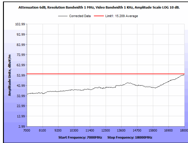
Plot 862. Radiated Spurious Emissions, 802.11n 40 MH, Channel 54, 1SS, 7 GHz – 18 GHz, Average
