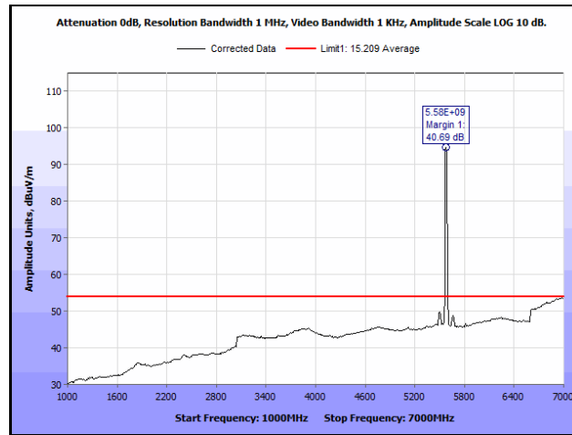
Plot 580. Radiated Spurious Emissions, 802.11ac 20 MH, Channel 116, 1SS, 1 GHz – 7 GHz, Average
