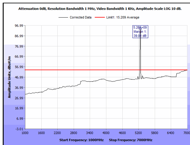
Plot 830. Radiated Spurious Emissions, 802.11n 20 MHz, Channel 52, 3SS, 1 GHz – 7 GHz, Average
