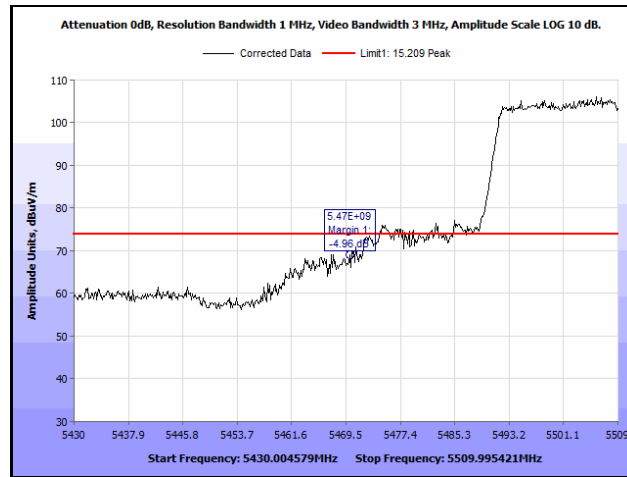
Plot 1015. Radiated Band Edge, 802.11n 40 MHz, 2SS, 5470 MHz, Peak
