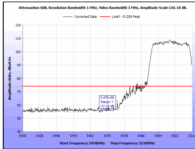
Plot 1003. Radiated Band Edge, 802.11n 20 MHz, 3SS, 5470 MHz, Peak
