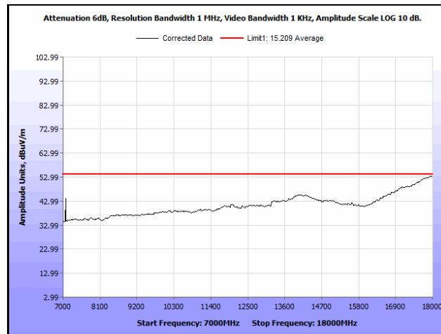
Plot 572. Radiated Spurious Emissions, 802.11ac 20 MH, Channel 64, 1SS, 7 GHz – 18 GHz, Average
