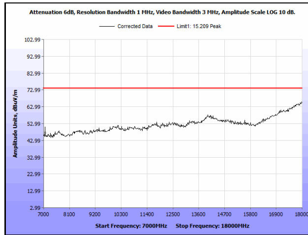
Plot 763. Radiated Spurious Emissions, 802.11ac 80 MH, Channel 106, 3SS, 7 GHz – 18 GHz, Peak
