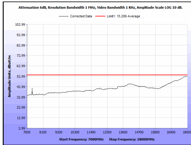
Plot 912. Radiated Spurious Emissions, 802.11n 40 MH, Channel 54, 3SS, 7 GHz – 18 GHz, Average
