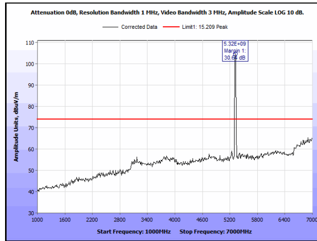
Plot 841. Radiated Spurious Emissions, 802.11n 20 MHz, Channel 64, 3SS, 1 GHz – 7 GHz, Peak
