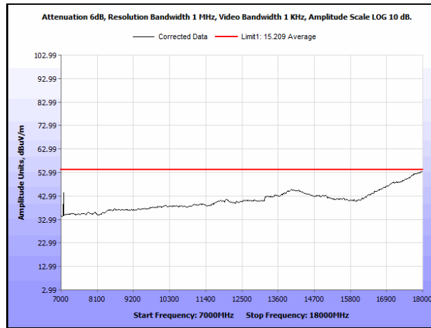
Plot 832. Radiated Spurious Emissions, 802.11n 20 MH, Channel 52, 3SS, 7 GHz – 18 GHz, Average
