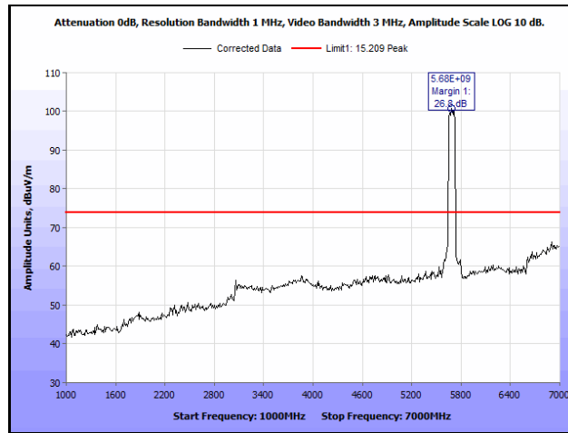
Plot 766. Radiated Spurious Emissions, 802.11ac 80 MH, Channel 138, 3SS, 1 GHz – 7 GHz, Peak
