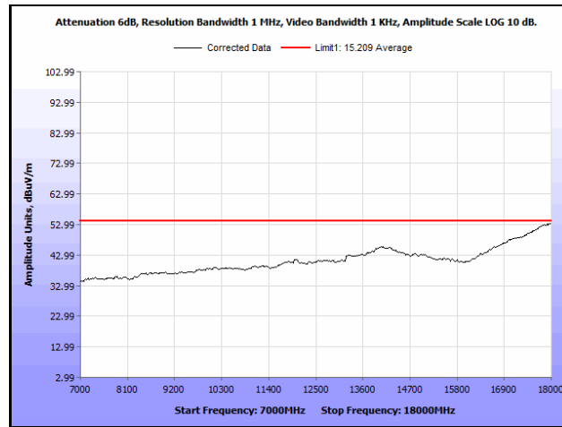
Plot 787. Radiated Spurious Emissions, 802.11n 20 MH, Channel 100, 1SS, 7 GHz – 18 GHz, Average
