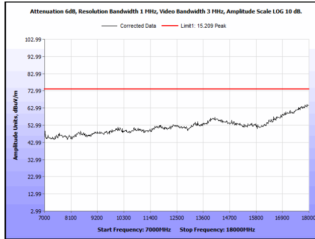
Plot 883. Radiated Spurious Emissions, 802.11n 40 MH, Channel 142, 1SS, 7 GHz – 18 GHz, Peak
