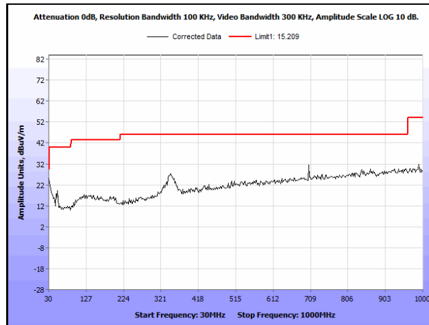
Plot 764. Radiated Spurious Emissions, 802.11ac 80 MH, Channel 138, 3SS, 30 MHz – 1 GHz
