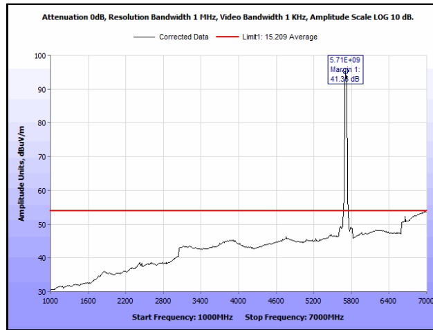
Plot 670. Radiated Spurious Emissions, 802.11ac 40 MHz, Channel 142, 1SS, 1 GHz – 7 GHz, Average
