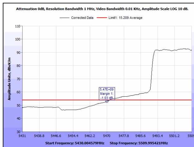
Plot 966. Radiated Band Edge, 802.11ac 40 MHz, 2SS, 5470 MHz, Average
