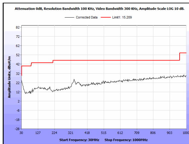
Plot 609. Radiated Spurious Emissions, 802.11ac 20 MH, Channel 116, 2SS, 30 MHz – 1 GHz
