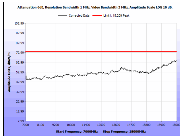
Plot 693. Radiated Spurious Emissions, 802.11ac 40 MH, Channel 110, 2SS, 7 GHz – 18 GHz, Peak
