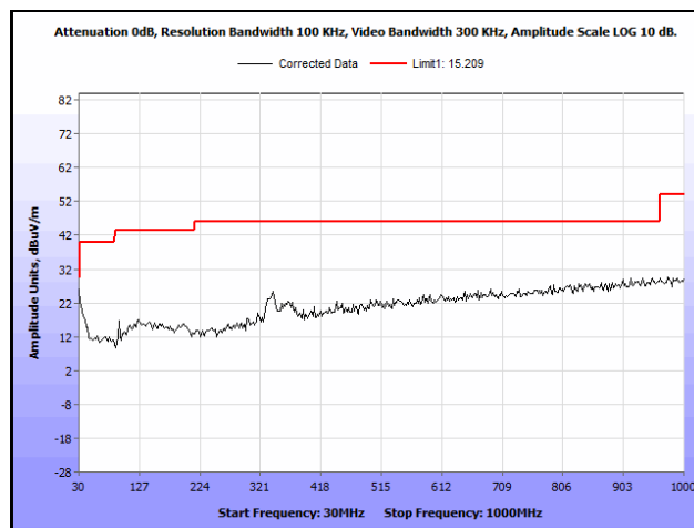
Plot 594. Radiated Spurious Emissions, 802.11ac 20 MH, Channel 60, 2SS, 30 MHz – 1 GHz
