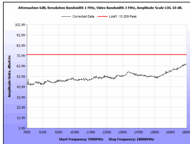
Plot 728. Radiated Spurious Emissions, 802.11ac 80 MHz, Channel 58, 1SS, 7 GHz – 18 GHz, Peak
