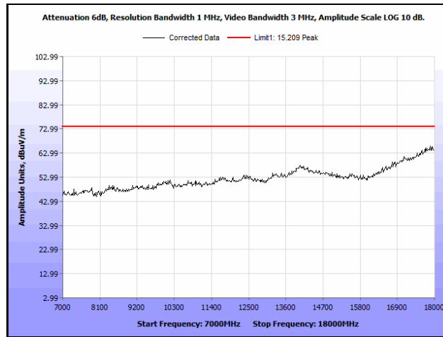
Plot 598. Radiated Spurious Emissions, 802.11ac 20 MHz, Channel 60, 2SS, 7 GHz – 18 GHz, Peak
