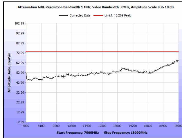
Plot 683. Radiated Spurious Emissions, 802.11ac 40 MHz, Channel 62, 2SS, 7 GHz – 18 GHz, Peak
