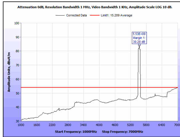
Plot 730. Radiated Spurious Emissions, 802.11ac 80 MH, Channel 106, 1SS, 1 GHz – 7 GHz, Average
