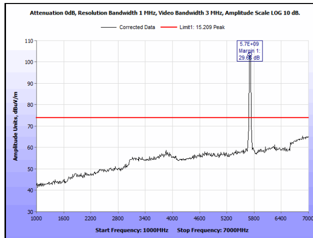
Plot 671. Radiated Spurious Emissions, 802.11ac 40 MHz, Channel 142, 1SS, 1 GHz – 7 GHz, Peak
