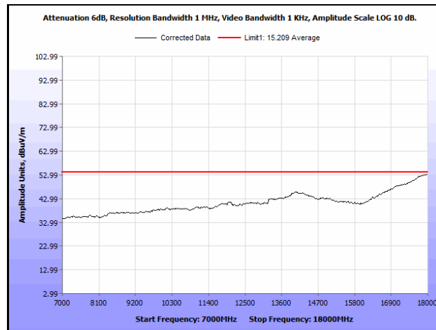
Plot 542. Radiated Spurious Emissions, 802.11a 20 MHz, Channel 64, 7 GHz – 18 GHz, Average
