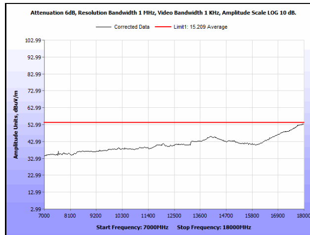
Plot 752. Radiated Spurious Emissions, 802.11ac 80 MH, Channel 138, 2SS, 7 GHz – 18 GHz, Average
