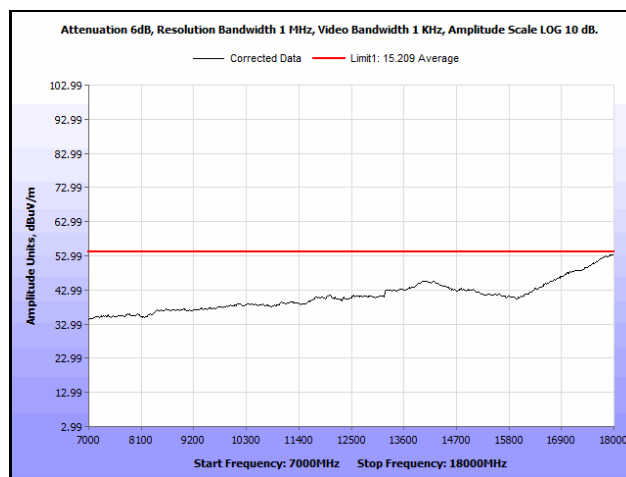
Plot 672. Radiated Spurious Emissions, 802.11ac 40 MHz, Channel 142, 1SS, 7 GHz – 18 GHz, Average
