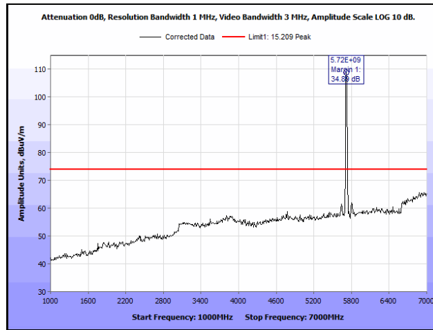
Plot 856. Radiated Spurious Emissions, 802.11n 20 MHz, Channel 144, 3SS, 1 GHz – 7 GHz, Peak
