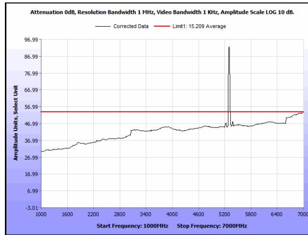
Plot 535. Radiated Spurious Emissions, 802.11a 20 MHz, Channel 60, 1 GHz – 7 GHz, Average
