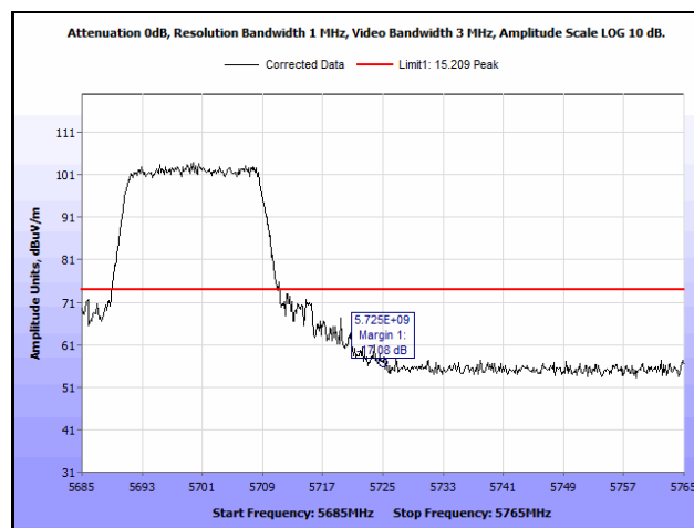
Plot 999. Radiated Band Edge, 802.11n 20 MHz, 2SS, 5725 MHz, Peak
