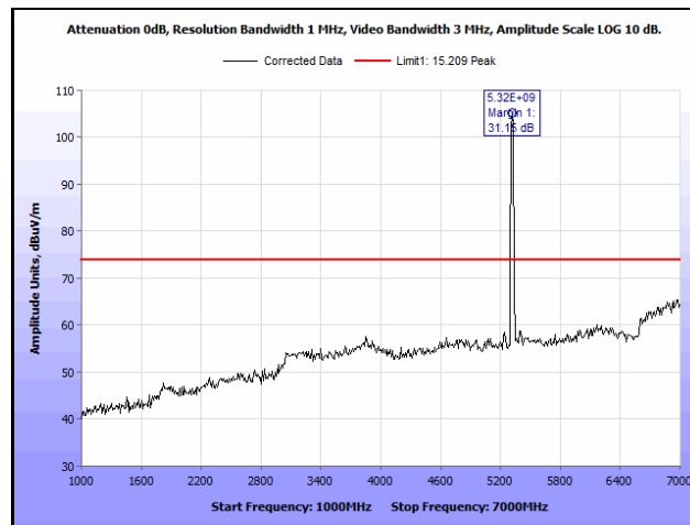
Plot 601. Radiated Spurious Emissions, 802.11ac 20 MHz, Channel 64, 2SS, 1 GHz – 7 GHz, Peak
