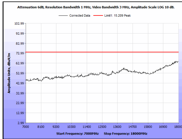
Plot 613. Radiated Spurious Emissions, 802.11ac 20 MH, Channel 116, 2SS, 7 GHz – 18 GHz, Peak
