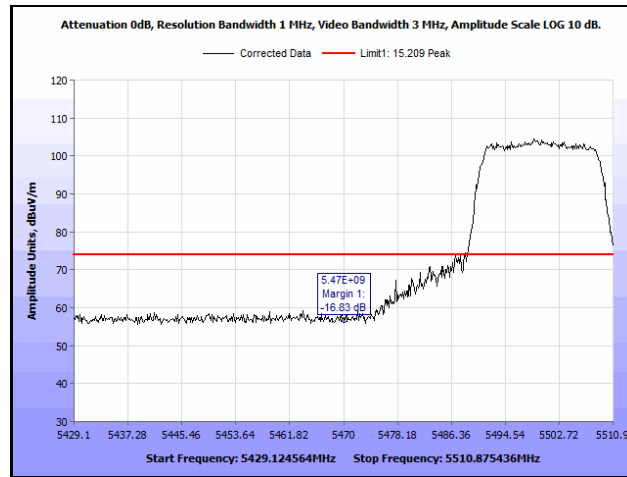
Plot 997. Radiated Band Edge, 802.11n 20 MHz, 2SS, 5470 MHz, Peak
