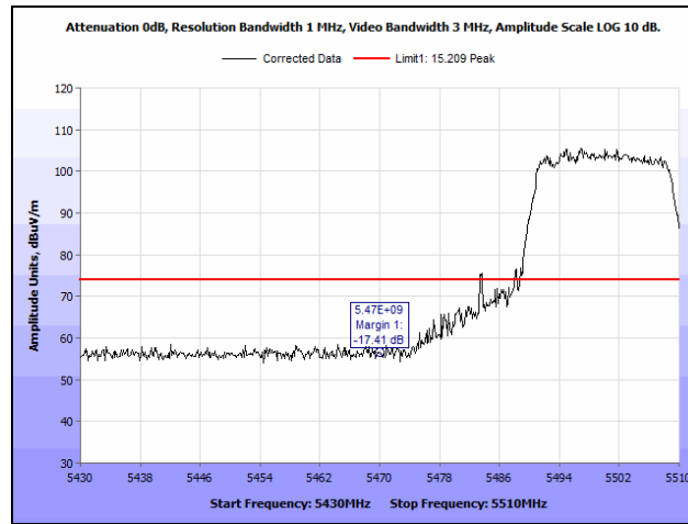
Plot 949. Radiated Band Edge, 802.11ac 20 MHz, 2SS, 5470 MHz, Peak
