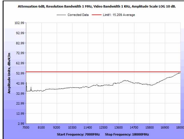
Plot 872. Radiated Spurious Emissions, 802.11n 40 MH, Channel 102, 1SS, 7 GHz – 18 GHz, Average
