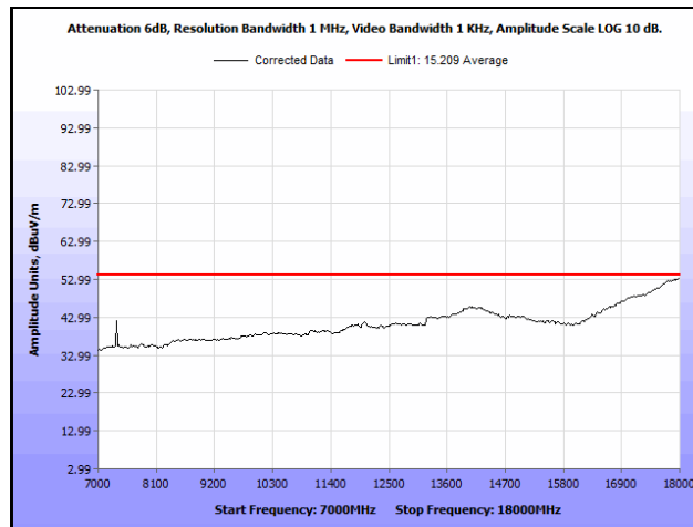
Plot 897. Radiated Spurious Emissions, 802.11n 40 MH, Channel 102, 2SS, 7 GHz – 18 GHz, Average
