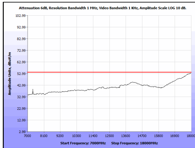
Plot 662. Radiated Spurious Emissions, 802.11ac 40 MHz, Channel 102, 1SS, 7 GHz – 18 GHz, Average
