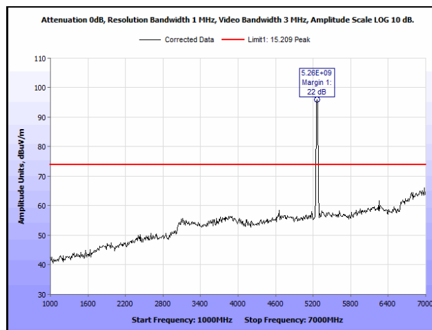
Plot 771. Radiated Spurious Emissions, 802.11n 20 MHz, Channel 52, 1SS, 1 GHz – 7 GHz, Peak
