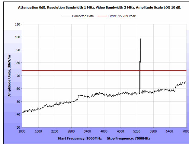
Plot 781. Radiated Spurious Emissions, 802.11n 20 MH, Channel 64, 1SS, 1 GHz – 7 GHz, Peak
