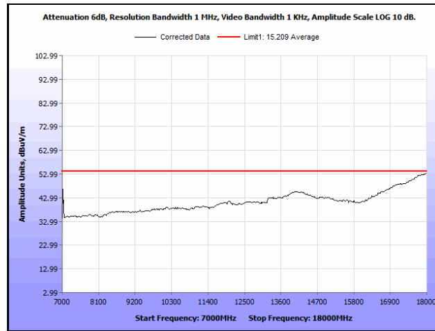
Plot 702. Radiated Spurious Emissions, 802.11ac 40 MH, Channel 54, 3SS, 7 GHz – 18 GHz, Average
