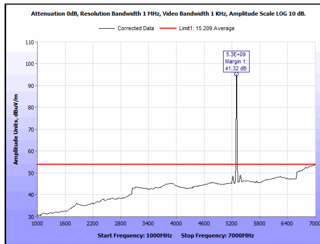
Plot 595. Radiated Spurious Emissions, 802.11ac 20 MHz, Channel 60, 2SS, 1 GHz – 7 GHz, Average
