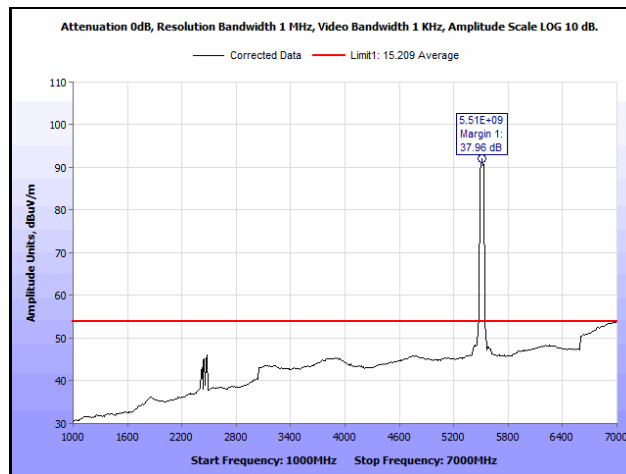
Plot 710. Radiated Spurious Emissions, 802.11ac 40 MHz, Channel 102, 3SS, 1 GHz – 7 GHz, Average
