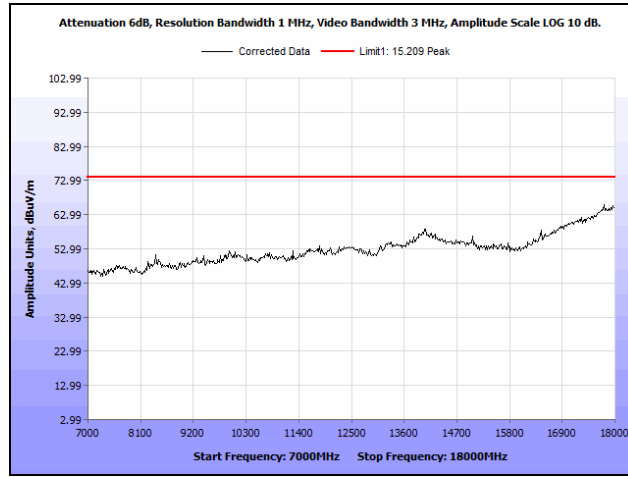
Plot 723. Radiated Spurious Emissions, 802.11ac 40 MH, Channel 142, 3SS, 7 GHz – 18 GHz, Peak
