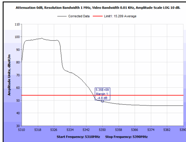
Plot 1000. Radiated Band Edge, 802.11n 20 MHz, 3SS, 5350 MHz, Average
