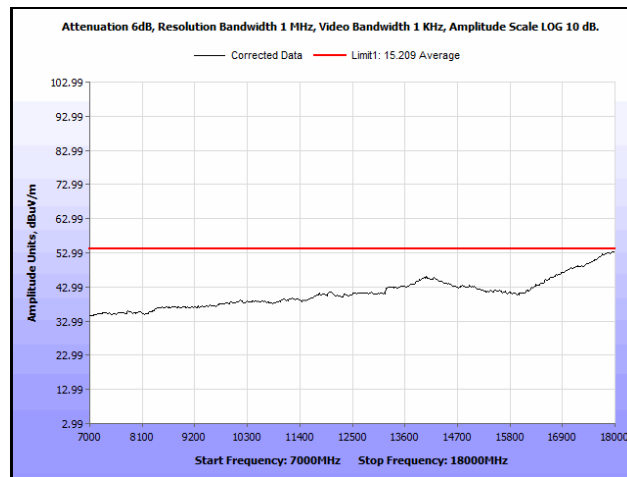
Plot 562. Radiated Spurious Emissions, 802.11ac 20 MH, Channel 52, 1SS, 7 GHz – 18 GHz, Average
