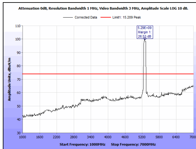
Plot 726. Radiated Spurious Emissions, 802.11ac 80 MHz, Channel 58, 1SS, 1 GHz – 7 GHz, Peak
