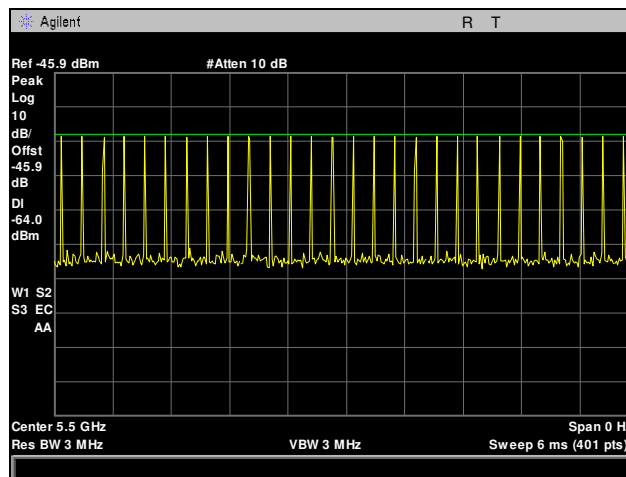
Plot 1026. Radar Waveform Calibration, Type 2, 5500 MHz
