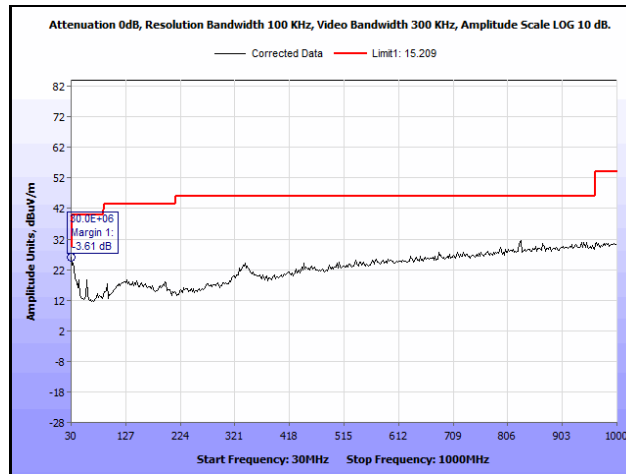
Plot 779. Radiated Spurious Emissions, 802.11n 20 MH, Channel 64, 1SS, 30 MHz – 1 GHz
