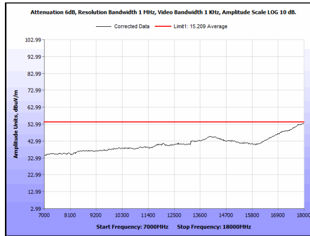
Plot 622. Radiated Spurious Emissions, 802.11ac 20 MH, Channel 52, 3SS, 7 GHz – 18 GHz, Average
