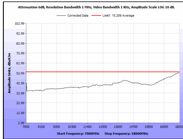
Plot 652. Radiated Spurious Emissions, 802.11ac 40 MHz, Channel 54, 1SS, 7 GHz – 18 GHz, Average
