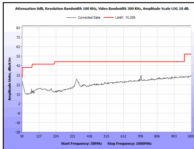
Plot 829. Radiated Spurious Emissions, 802.11n 20 MHz, Channel 52, 3SS, 30 MHz – 1 GHz
