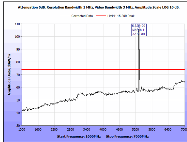
Plot 811. Radiated Spurious Emissions, 802.11n 20 MH, Channel 64, 2SS, 1 GHz – 7 GHz, Peak
