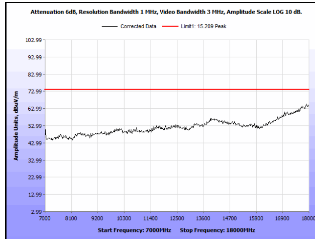
Plot 878. Radiated Spurious Emissions, 802.11n 40 MHz, Channel 110, 1SS, 7 GHz – 18 GHz, Peak
