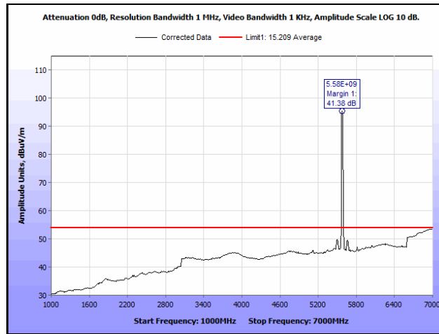
Plot 850. Radiated Spurious Emissions, 802.11n 20 MH, Channel 116, 3SS, 1 GHz – 7 GHz, Average
