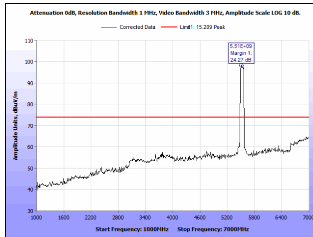
Plot 731. Radiated Spurious Emissions, 802.11ac 80 MH, Channel 106, 1SS, 1 GHz – 7 GHz, Peak
