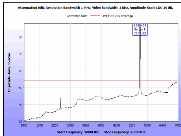
Plot 920. Radiated Spurious Emissions, 802.11n 40 MHz, Channel 102, 3SS, 1 GHz – 7 GHz, Average
