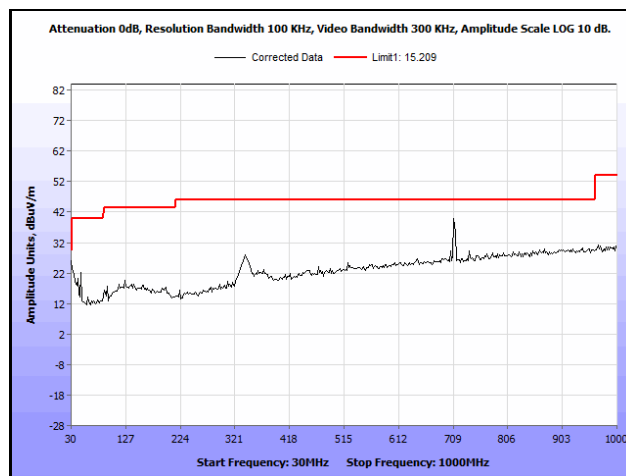
Plot 914. Radiated Spurious Emissions, 802.11n 40 MH, Channel 62, 3SS, 30 MHz – 1 GHz
