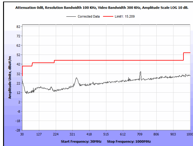
Plot 824. Radiated Spurious Emissions, 802.11n 20 MH, Channel 144, 2SS, 30 MHz – 1 GHz
