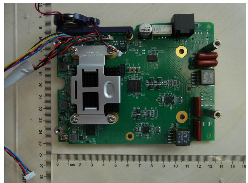
Figure 28: PCB with DSL connector SCTPS-AB-CU, SCTPS-AB
