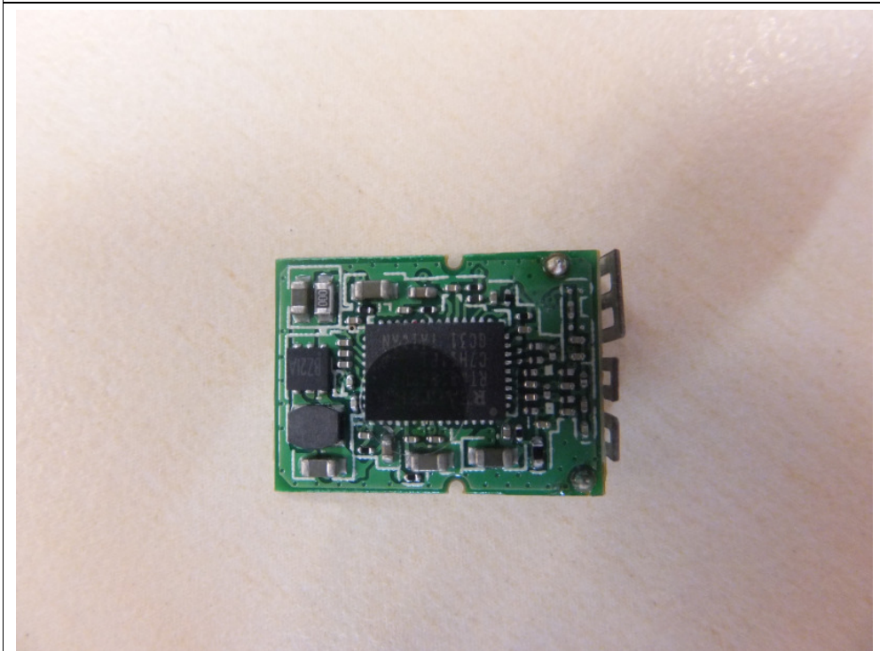
Figure 37: Wi-Fi USB dongle PCB view 1
