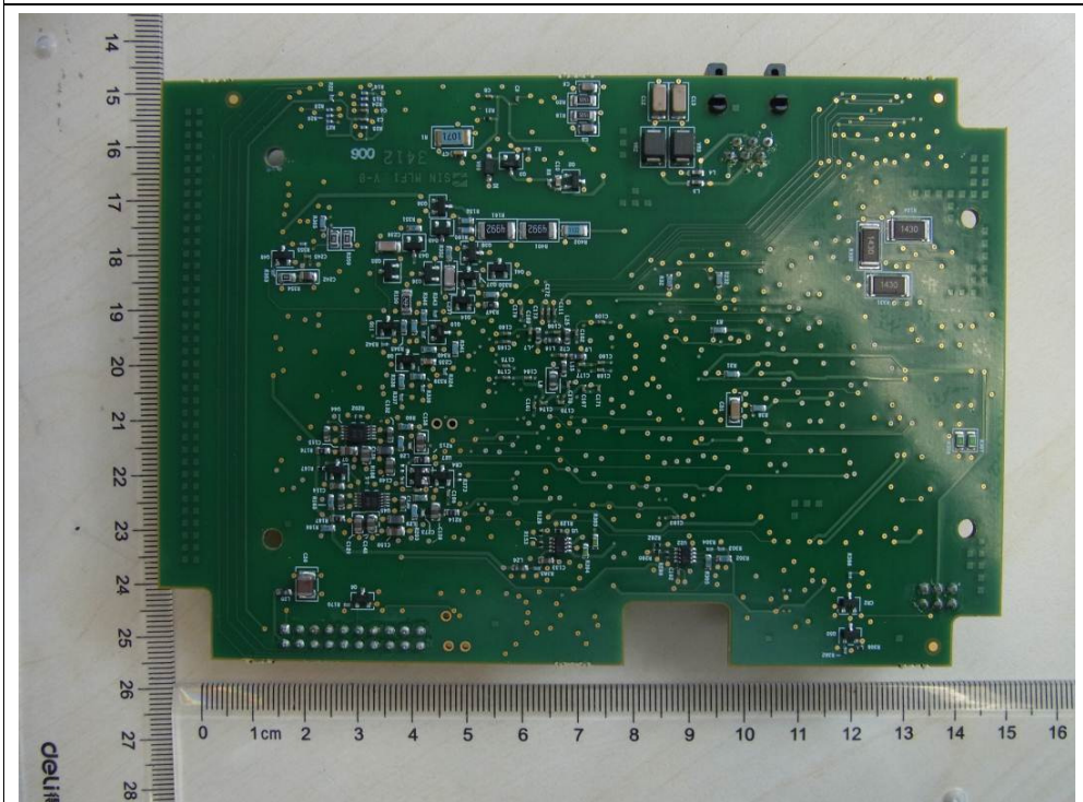
Figure 23 PCB with POTS connector CSC-TPSVW-CU, SCTPS-AB-CU
