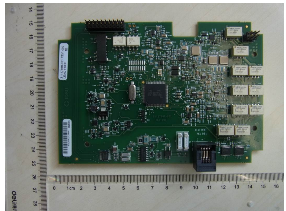
Figure 22: PCB with POTS connector CSC-TPSVW-CU, SCTPS-AB-CU
