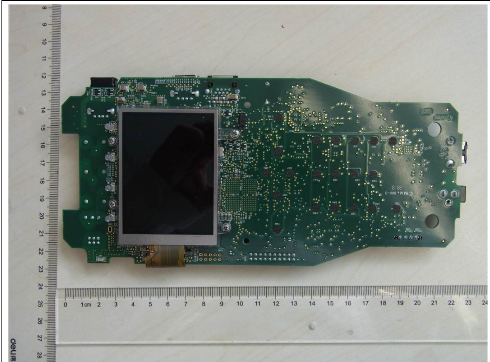
Figure 21: Main PCB
