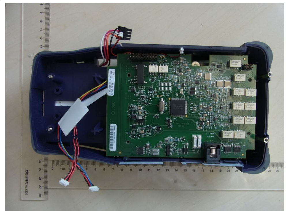
Figure 18: Internal view bottom enclosure CSC-TPSVW-CU, SCTPS-AB-CU
