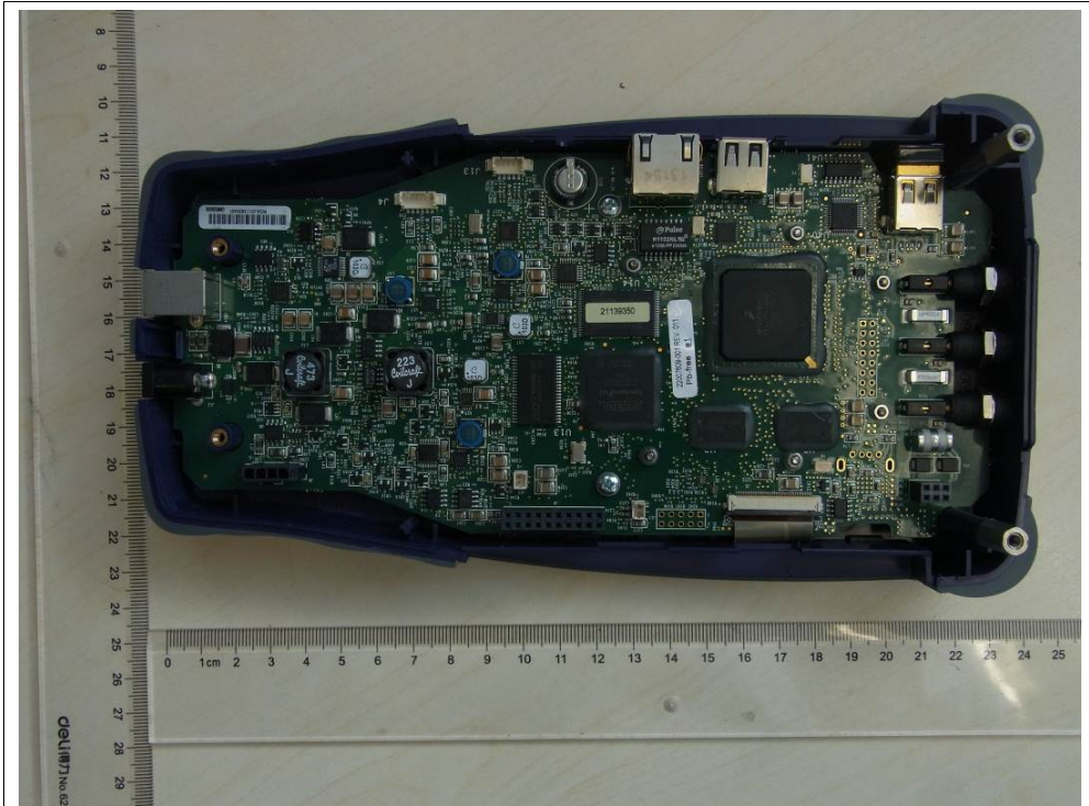
Figure 16: Internal view
