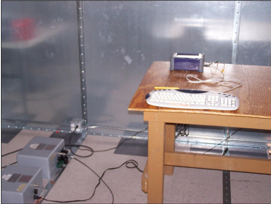
Photograph 5. Conducted Emissions, 15.207(a), Test Setup
