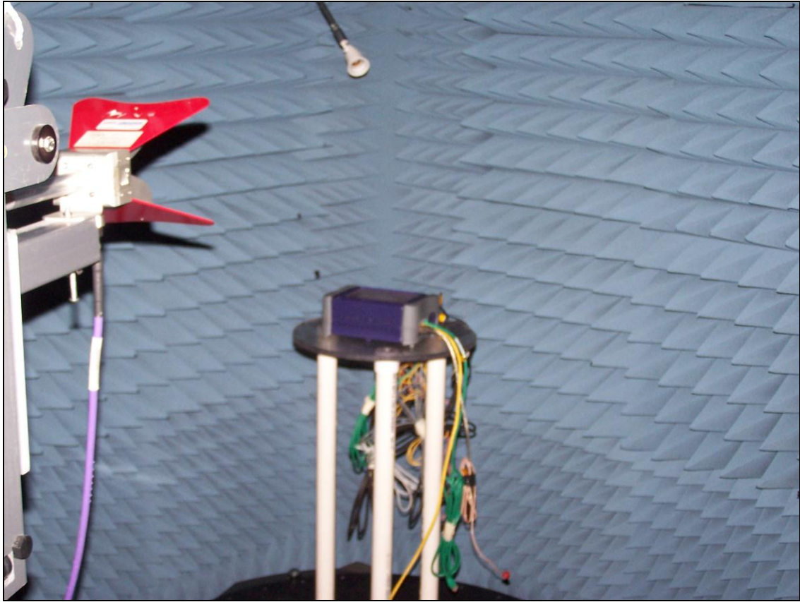
Photograph 8. Radiated Spurious Emissions, Test Setup
