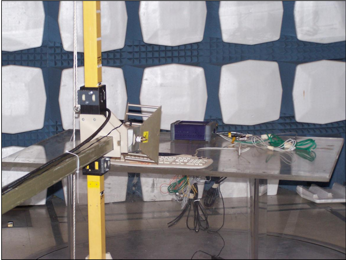
Photograph 3. Radiated Emission, Test Setup, 1 GHz to 5 GHz
