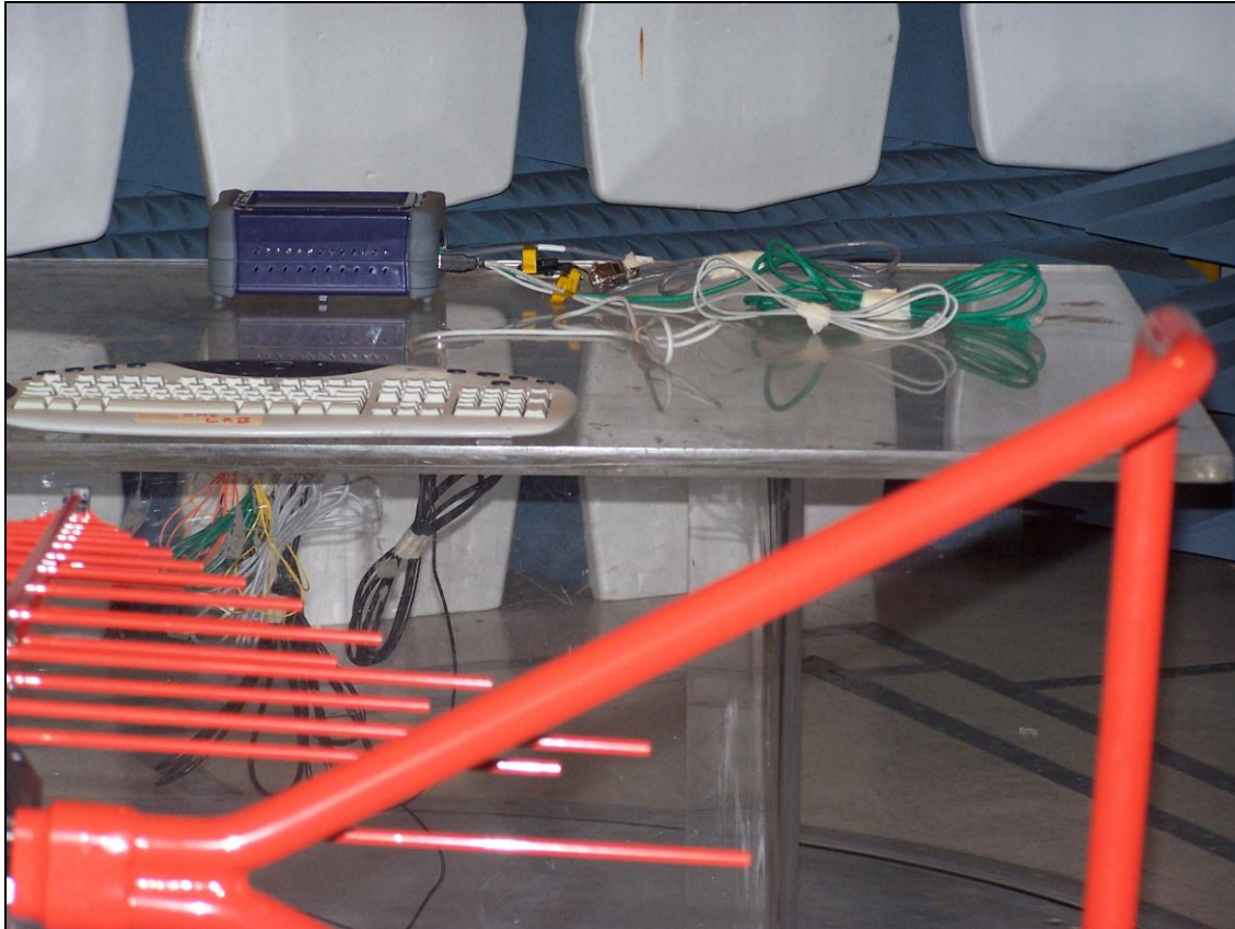
Photograph 6. Radiated Spurious Emissions, Test Setup, Low Frequency
