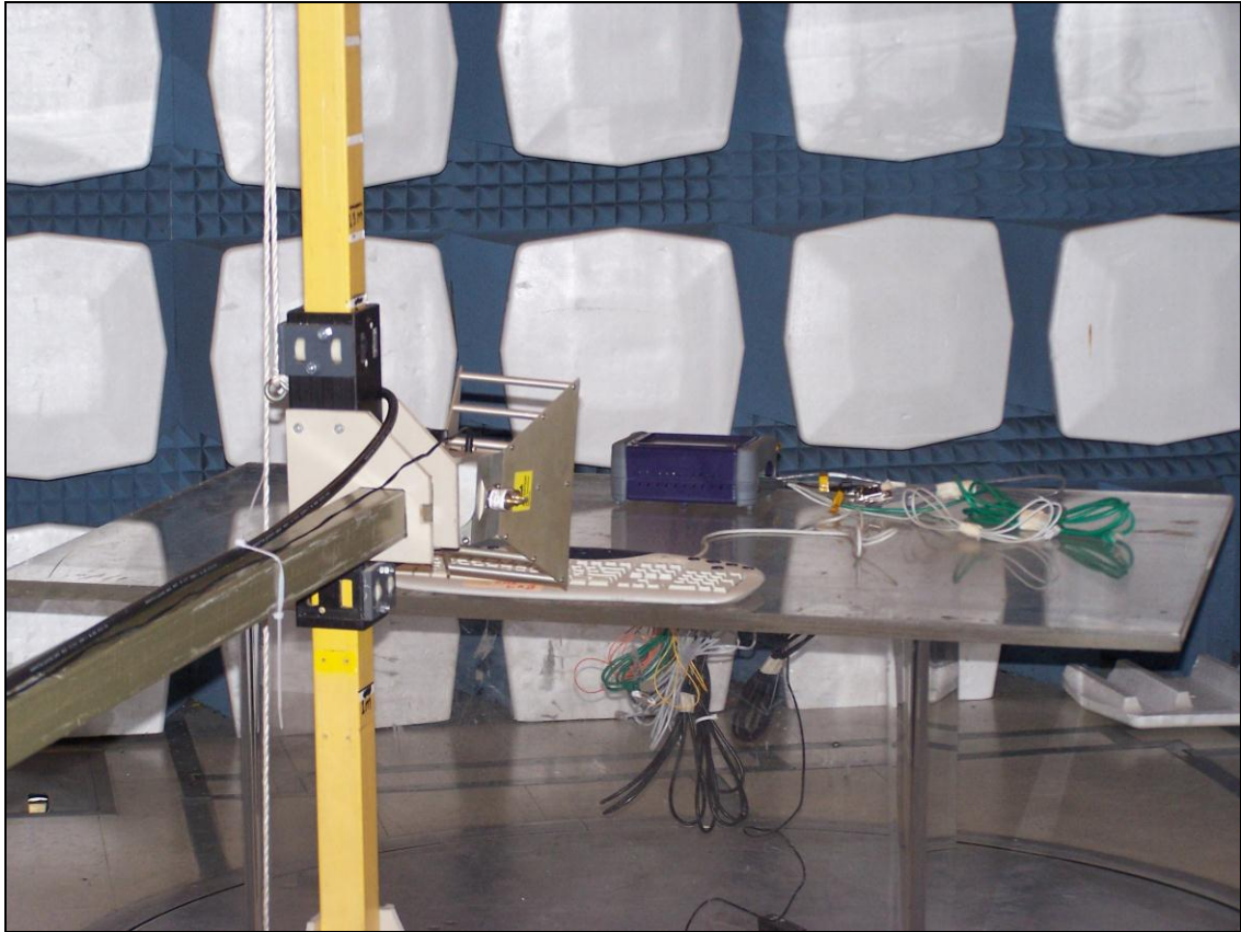
Photograph 7. Radiated Spurious Emissions, Test Setup, High Frequency
