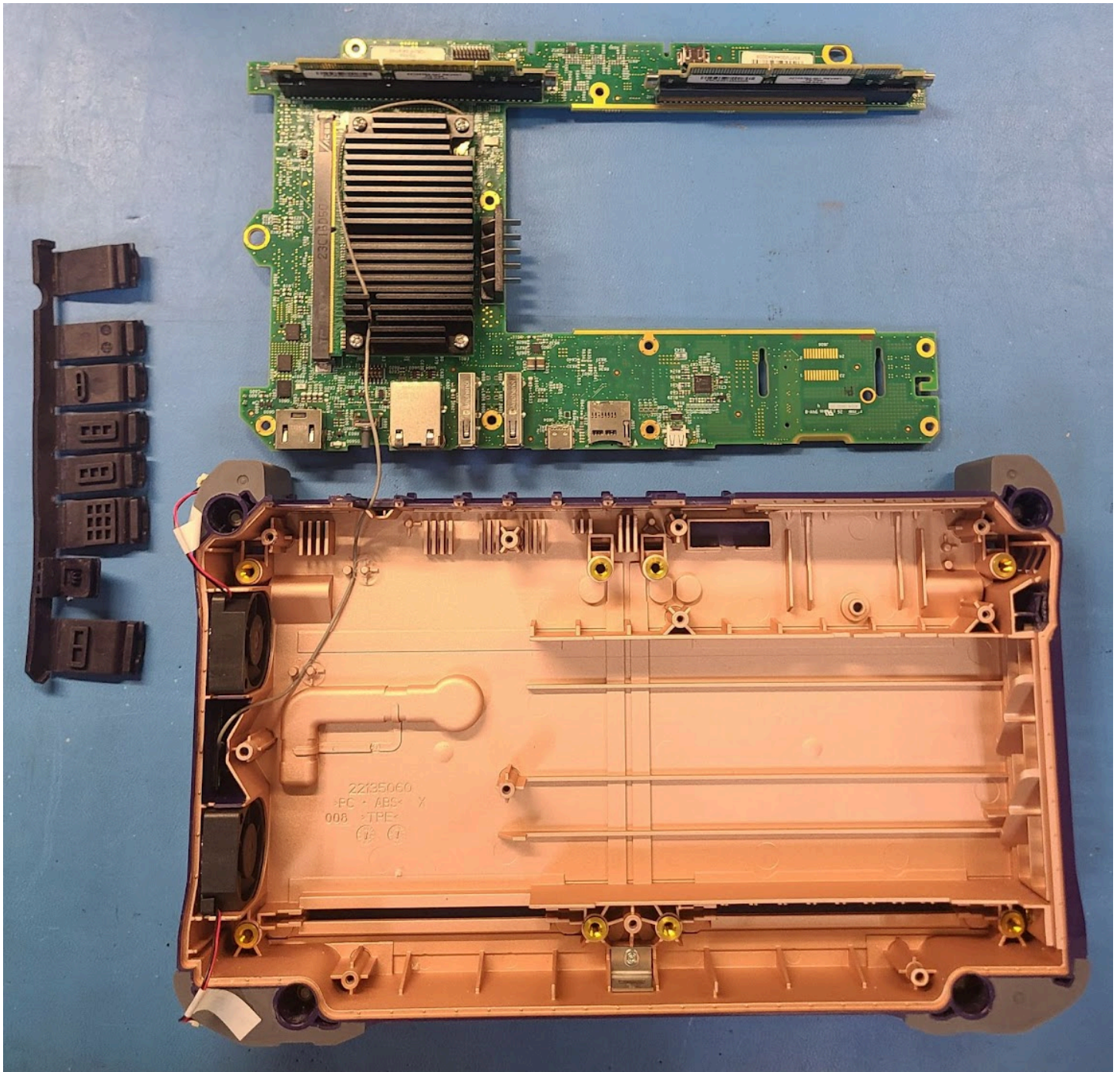
Disassembled
