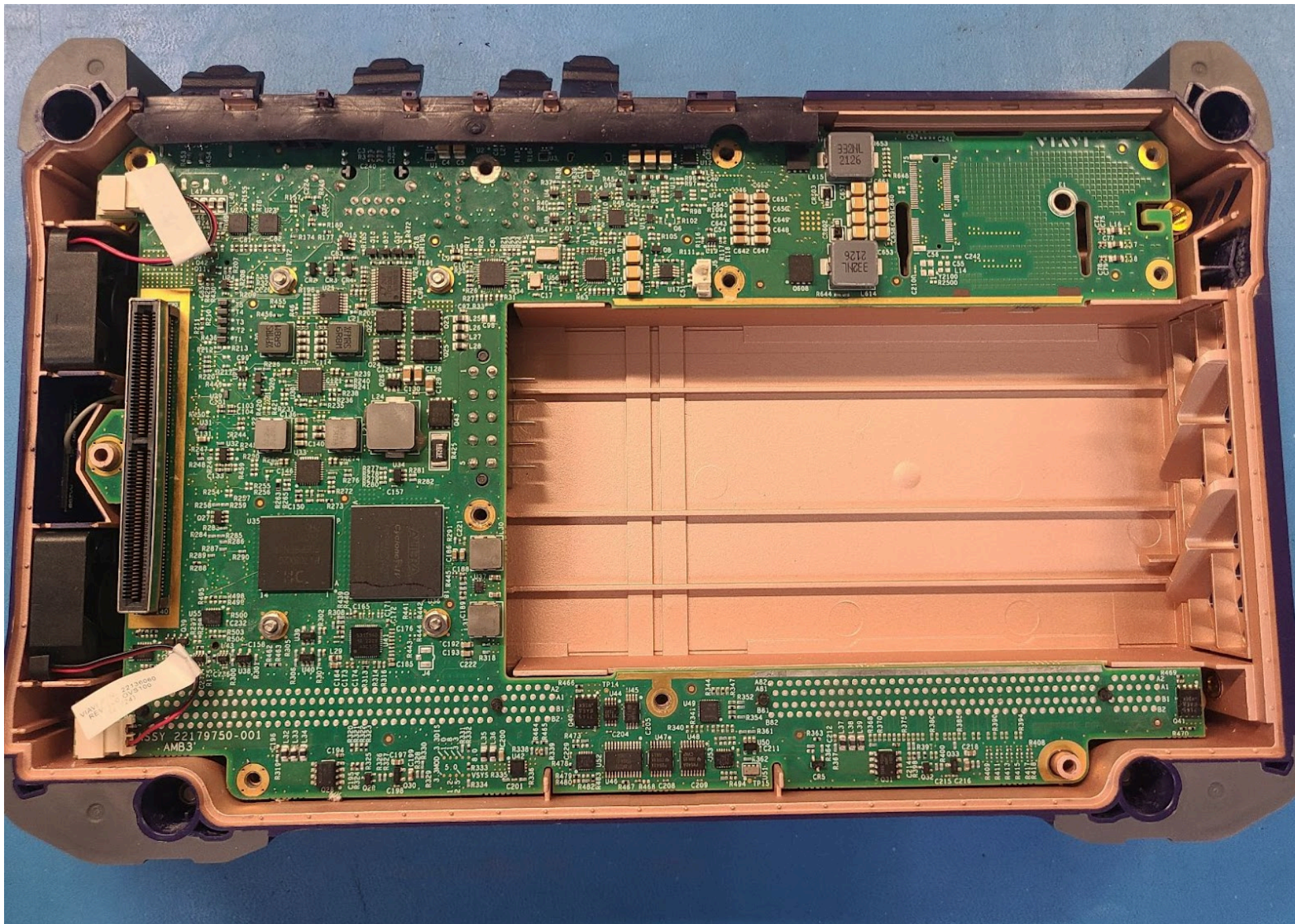
Cover Removed
