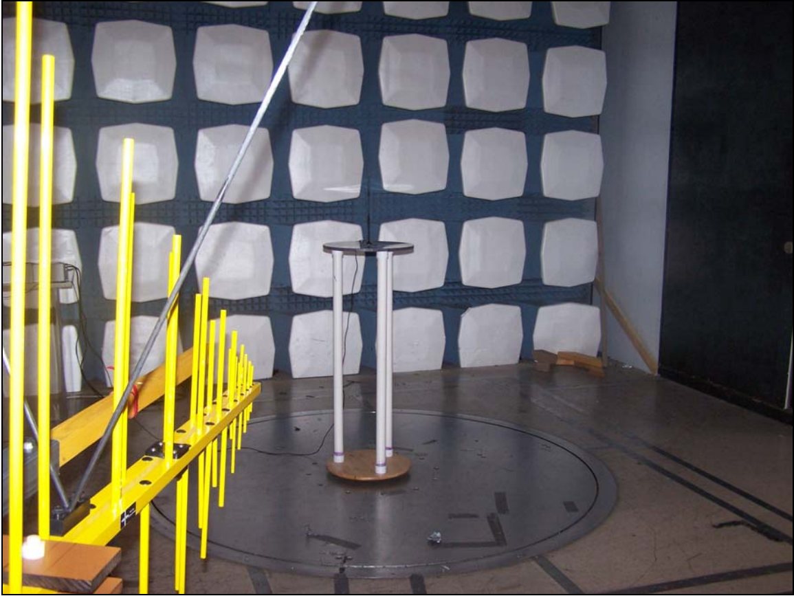
Photograph 2. 850 MHz, Test Setup
