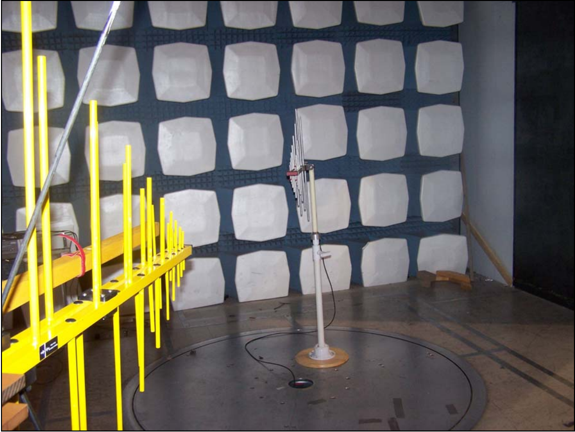
Photograph 1. 850 MHz, Antenna Substitution
