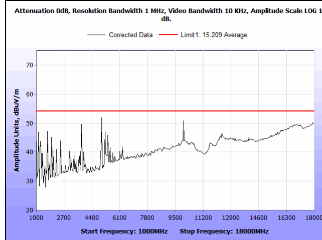
Plot 12. Radiated Emissions, 1 – 18 GHz, BT, 15 High Average
