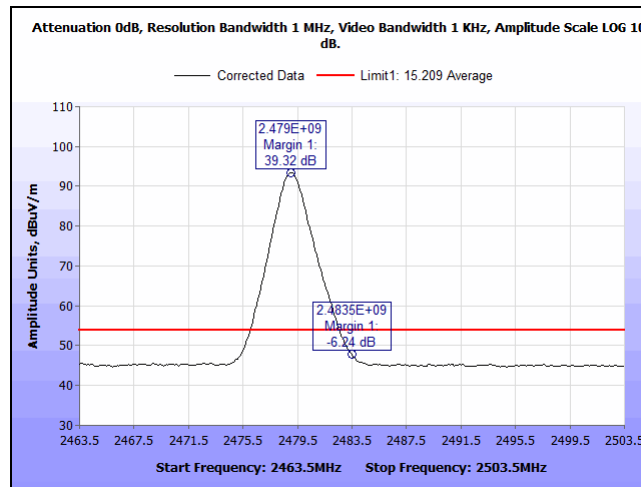
Plot 14. Radiated Restricted Band Edge, BT, 15 High Average
