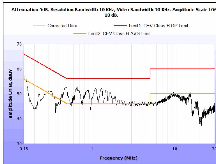
Plot 1. Conducted Emissions, 15.207(a), Phase Line Transmitter OFF
