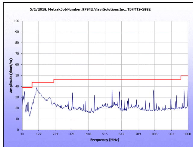
Plot 6. Radiated Spurious Emissions, 30 MHz – 1 GHz, BT, 15 Mid
