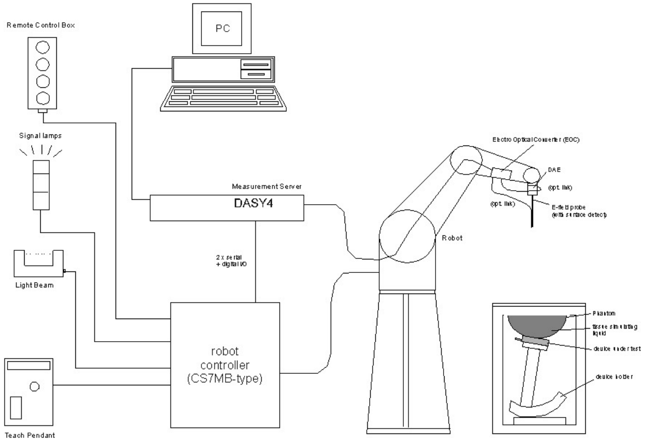
Figure 7: SAR Measurement System
