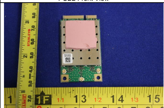
Module Front View
