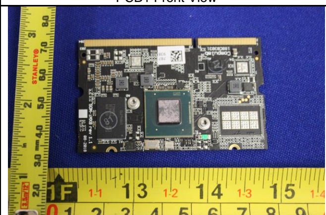
PCB2 Front View
