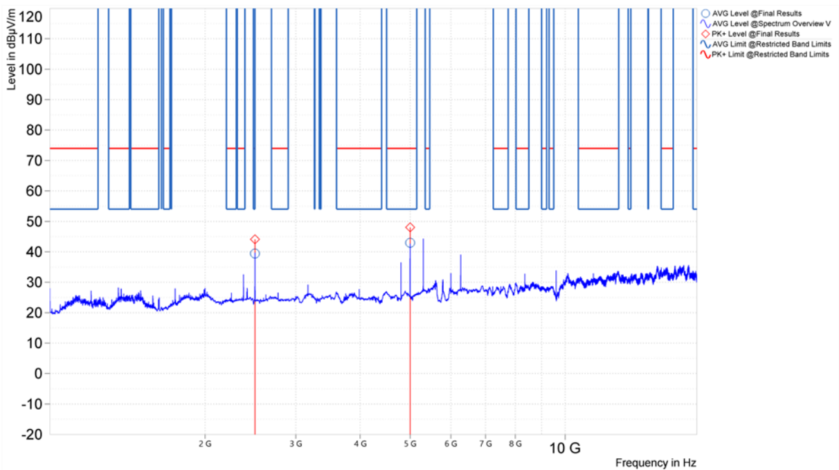
Figure 59. Worst Case Spurious Emissions, 1GHz – 18GHz, 802.11a, Vertical (U-NII-3, Middle Channel)
