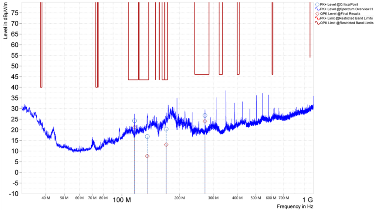
Figure 40. Worst Case Spurious Emissions, 30MHz – 1GHz, 802.11a, Horizontal (U-NII-2C, Middle Channel)
