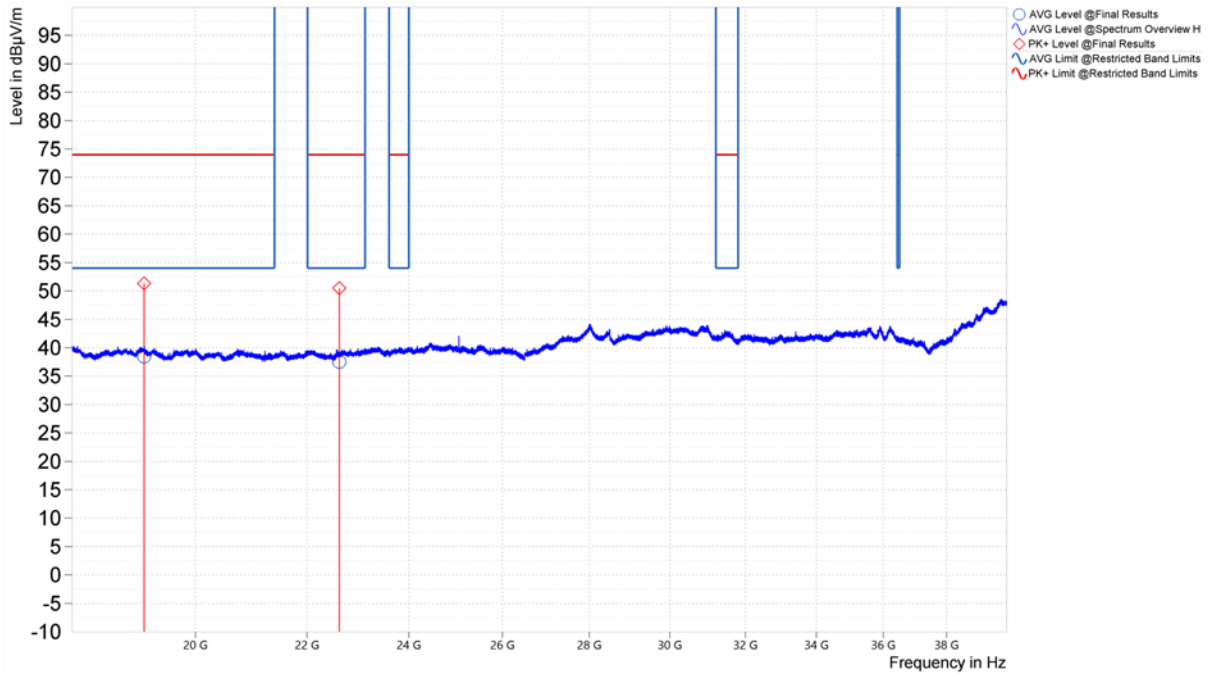
Figure 60. Worst Case Spurious Emissions, 18GHz – 40GHz, 802.11a, Horizontal (U-NII-3, Middle Channel)
