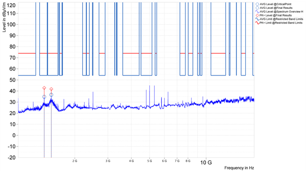
Figure 58. Worst Case Spurious Emissions, 1GHz – 18GHz, 802.11a, Horizontal (U-NII-3, Middle Channel)
