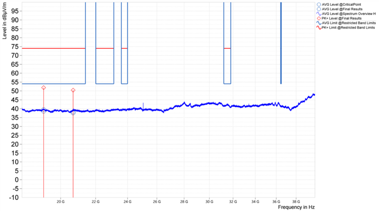
Figure 44. Worst Case Spurious Emissions, 18GHz – 40GHz, 802.11a, Horizontal (U-NII-2C, Middle Channel)
