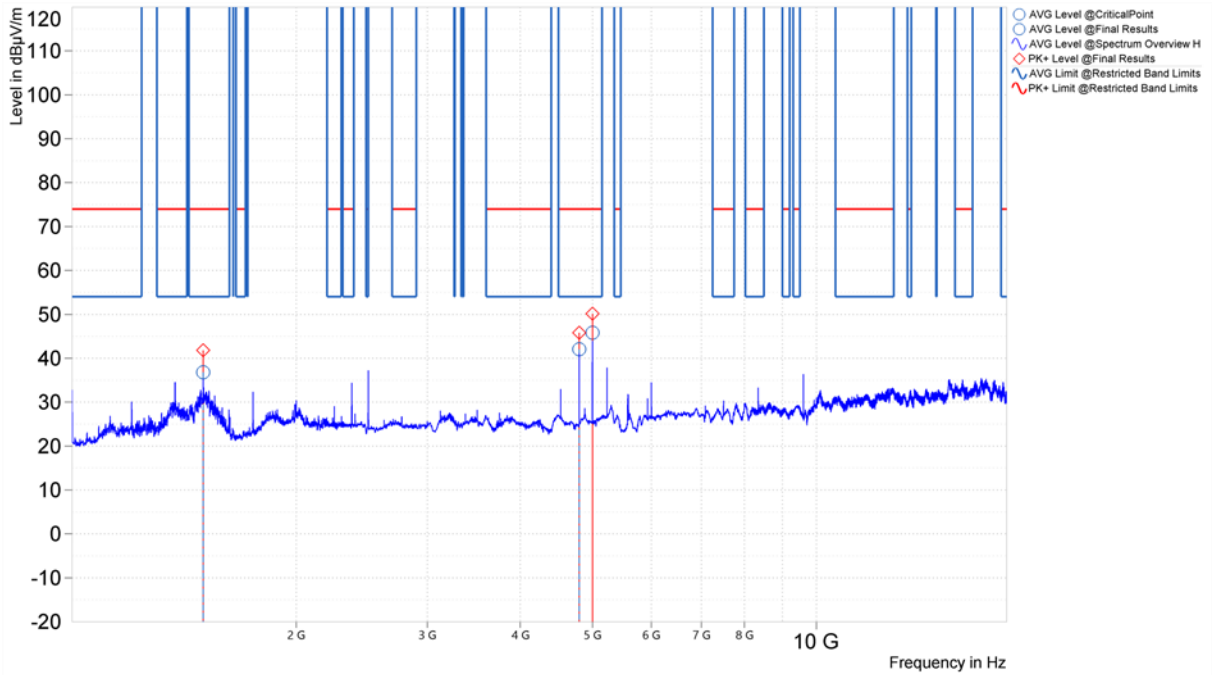
Figure 50. Worst Case Spurious Emissions, 1GHz – 18GHz, 802.11n, Horizontal (U-NII-2C, Middle Channel)
