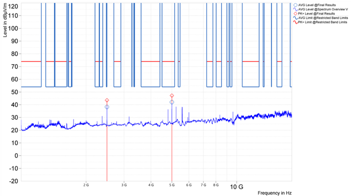
Figure 43. Worst Case Spurious Emissions, 1GHz – 18GHz, 802.11a, Vertical (U-NII-2C, Middle Channel)
