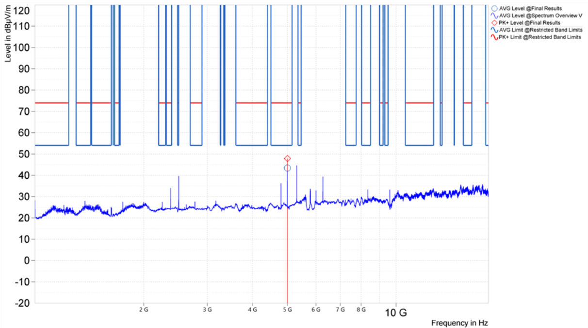
Figure 67. Worst Case Spurious Emissions, 1GHz – 18GHz, 802.11n, Vertical (U-NII-3, Middle Channel)
