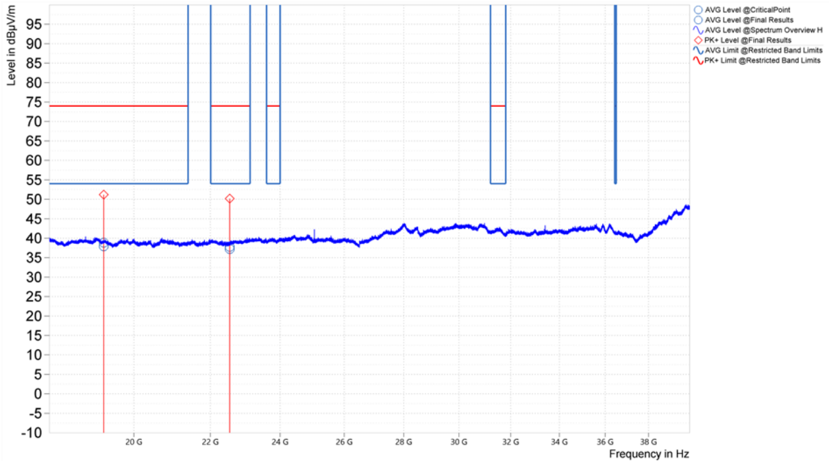
Figure 52. Worst Case Spurious Emissions, 18GHz – 40GHz, 802.11n, Horizontal (U-NII-2C, Middle Channel)
