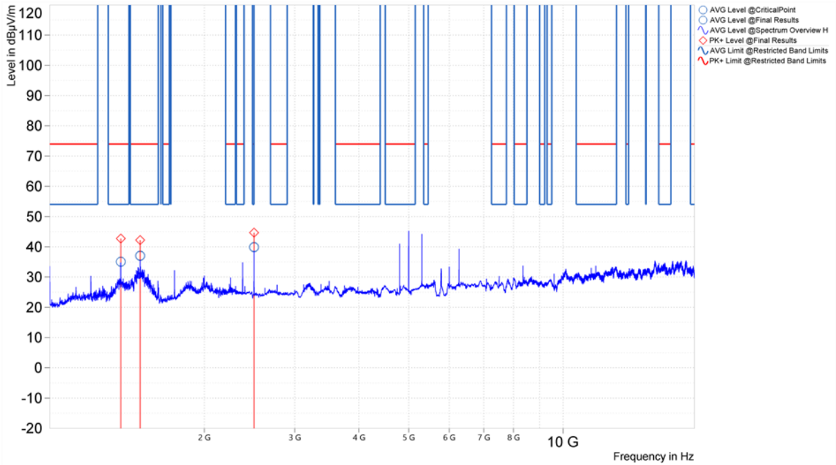
Figure 66. Worst Case Spurious Emissions, 1GHz – 18GHz, 802.11n, Horizontal (U-NII-3 Middle Channel)
