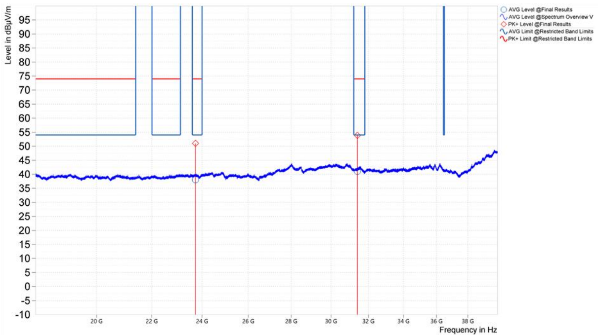
Figure 69. Worst Case Spurious Emissions, 18GHz – 40GHz, 802.11n, Vertical (U-NII-3, Middle Channel)
