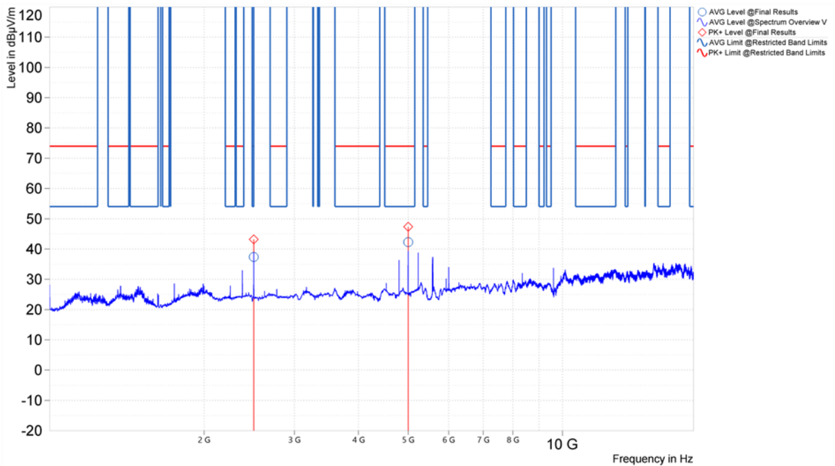
Figure 51. Worst Case Spurious Emissions, 1GHz – 18GHz, 802.11n, Vertical (U-NII-2C, Middle Channel)
