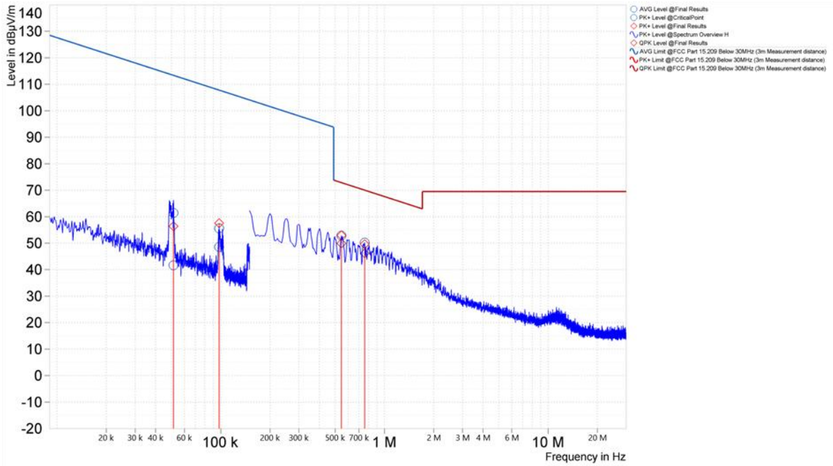
Figure 62. Worst Case Spurious Emissions, 9kHz – 30MHz, 802.11n, Coplanar Loop (U-NII-3, Middle Channel)
