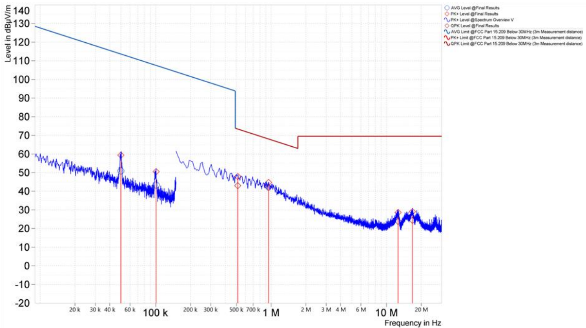
Figure 47. Worst Case Spurious Emissions, 9kHz – 30MHz, 802.11n, Coaxial Loop (U-NII-2C, Middle Channel)
