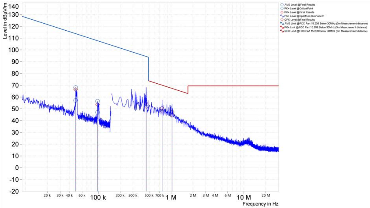
Figure 54. Worst Case Spurious Emissions, 9kHz – 30MHz, 802.11a, Coplanar Loop (U-NII-3, Middle Channel)
