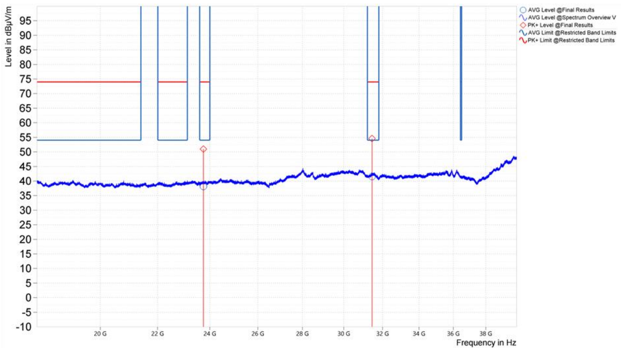
Figure 61. Worst Case Spurious Emissions, 18GHz – 40GHz, 802.11a, Vertical (U-NII-3, Middle Channel)
