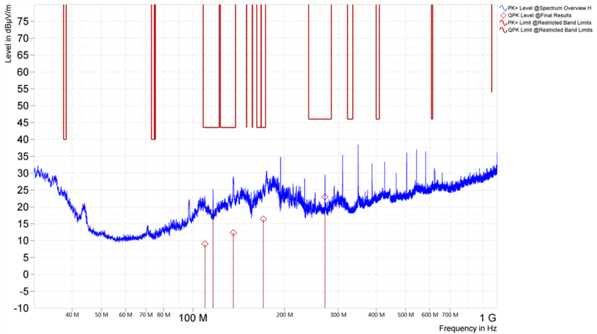
Figure 64. Worst Case Spurious Emissions, 30MHz – 1GHz, 802.11n, Horizontal (U-NII-3, Middle Channel)
