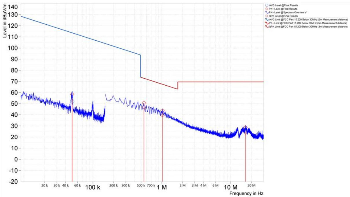
Figure 55. Worst Case Spurious Emissions, 9kHz – 30MHz, 802.11a, Coaxial Loop (U-NII-3, Middle Channel)
