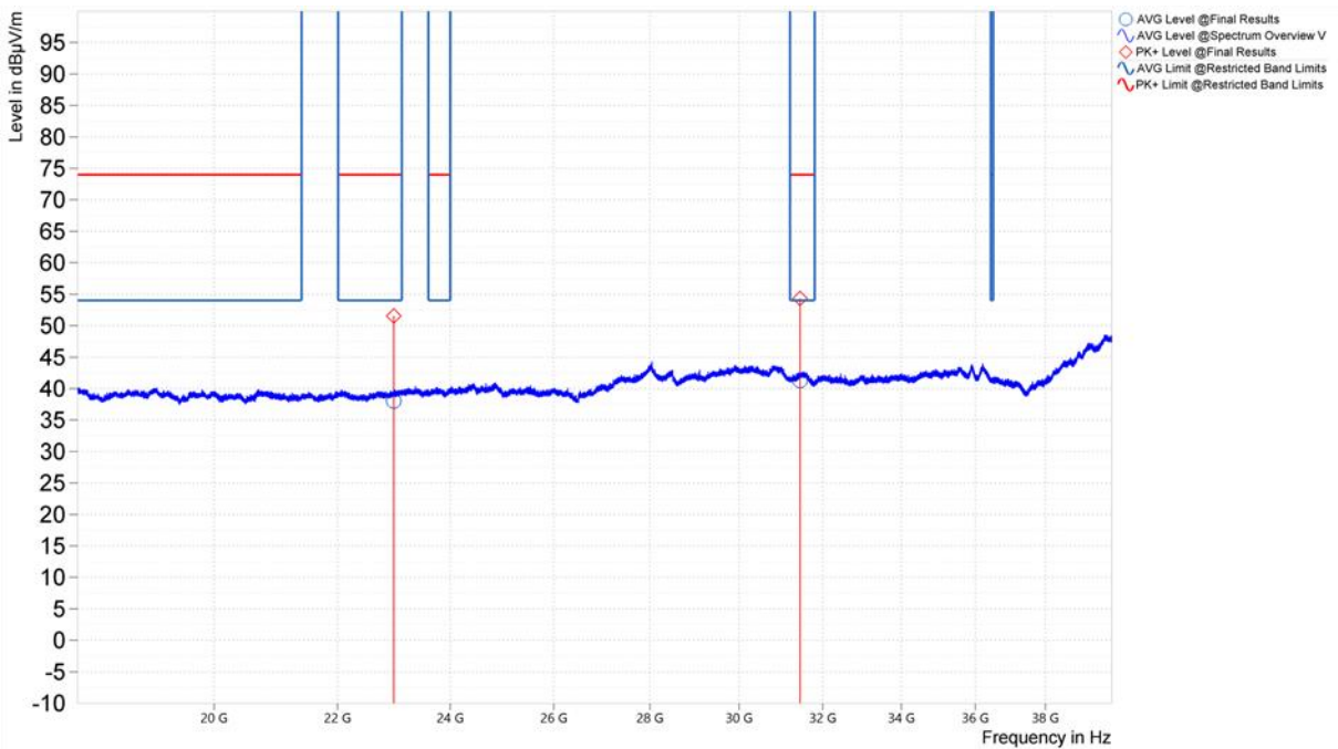
Figure 45. Worst Case Spurious Emissions, 18GHz – 40GHz, 802.11a, Vertical (U-NII-2C, Middle Channel)
