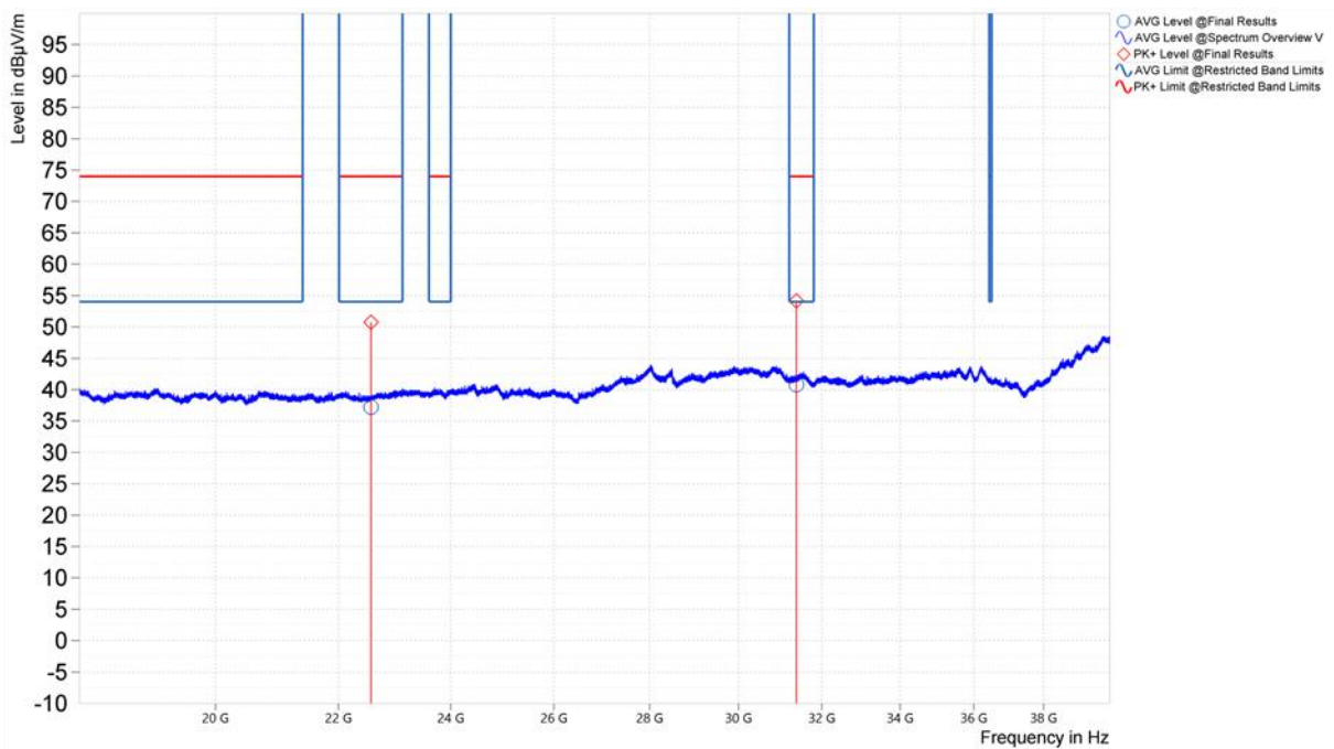
Figure 53. Worst Case Spurious Emissions, 18GHz – 40GHz, 802.11n, Vertical (U-NII-2C, Middle Channel)
