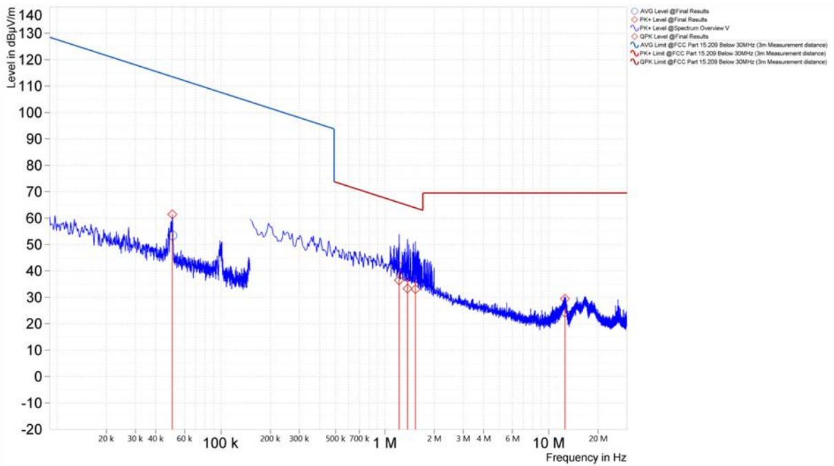
Figure 63. Worst Case Spurious Emissions, 9kHz – 30MHz, 802.11n, Coaxial Loop (U-NII-3, Middle Channel)
