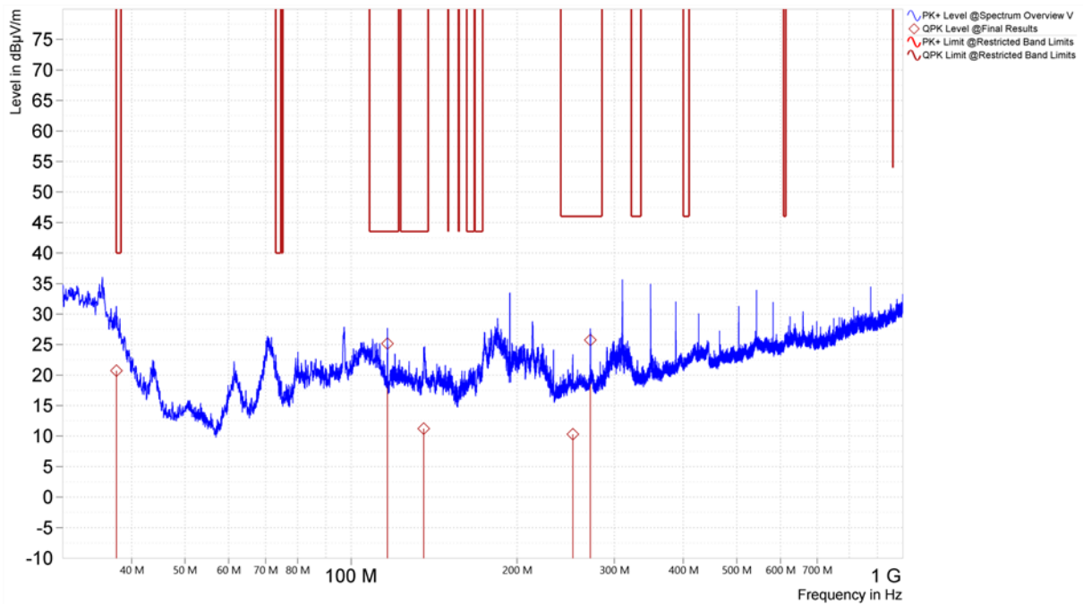
Figure 41. Worst Case Spurious Emissions, 30MHz – 1GHz, 802.11a, Vertical (U-NII-2C, Middle Channel)
