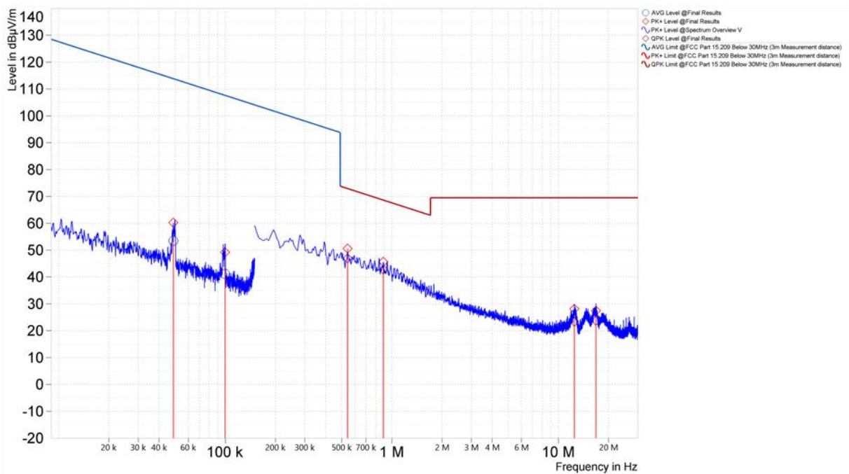
Figure 31. Worst Case Spurious Emissions, 9kHz – 30MHz, 802.11n, Coaxial Loop (U-NII-2A, Middle Channel)
