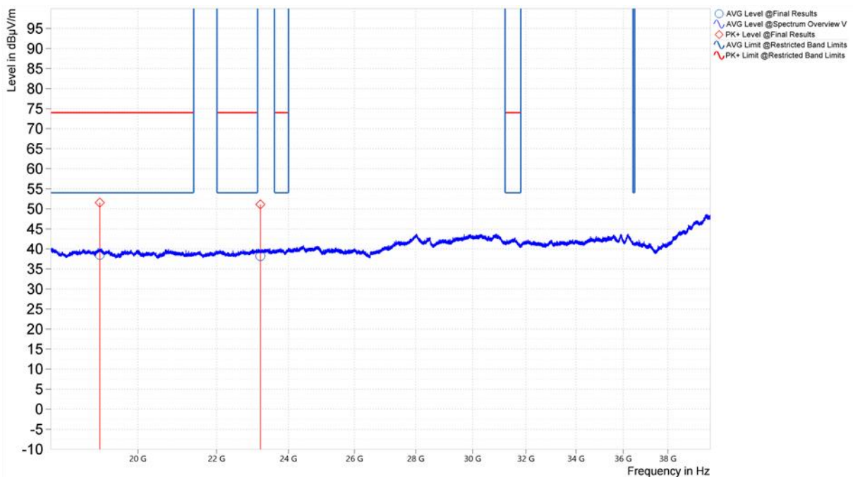
Figure 29. Worst Case Spurious Emissions, 18GHz – 40GHz, 802.11a, Vertical (U-NII-2A, Middle Channel)
