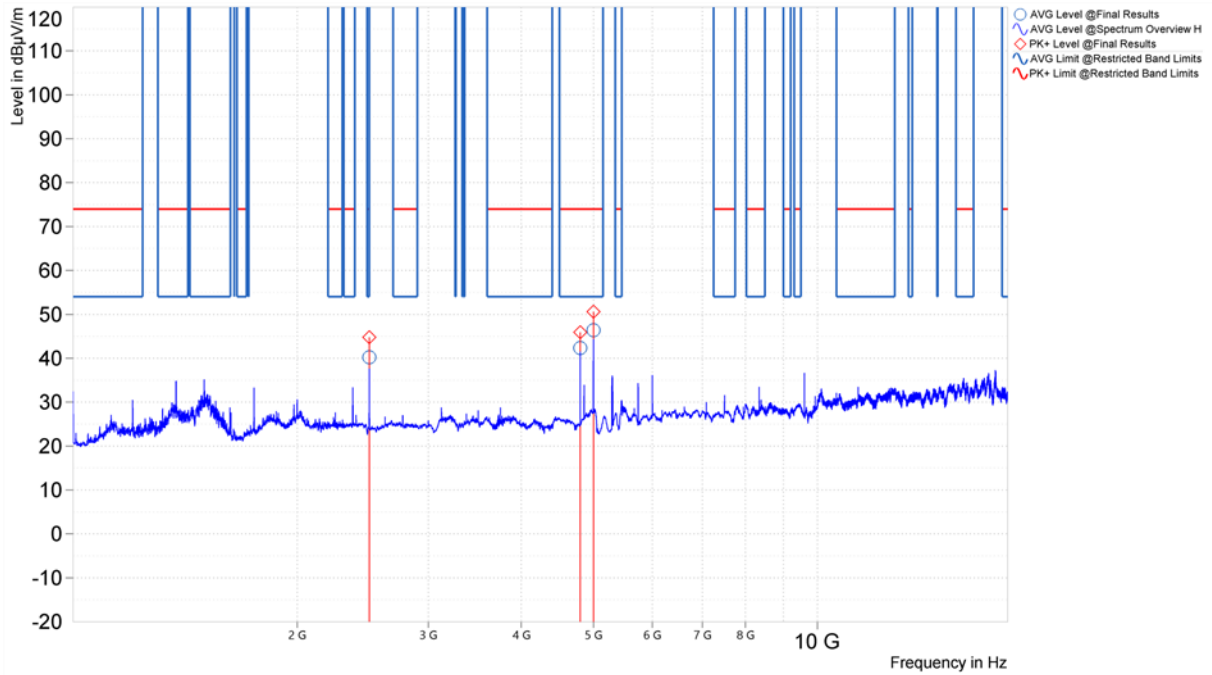
Figure 26. Worst Case Spurious Emissions, 1GHz – 18GHz, 802.11a, Horizontal (U-NII-2A, Middle Channel)
