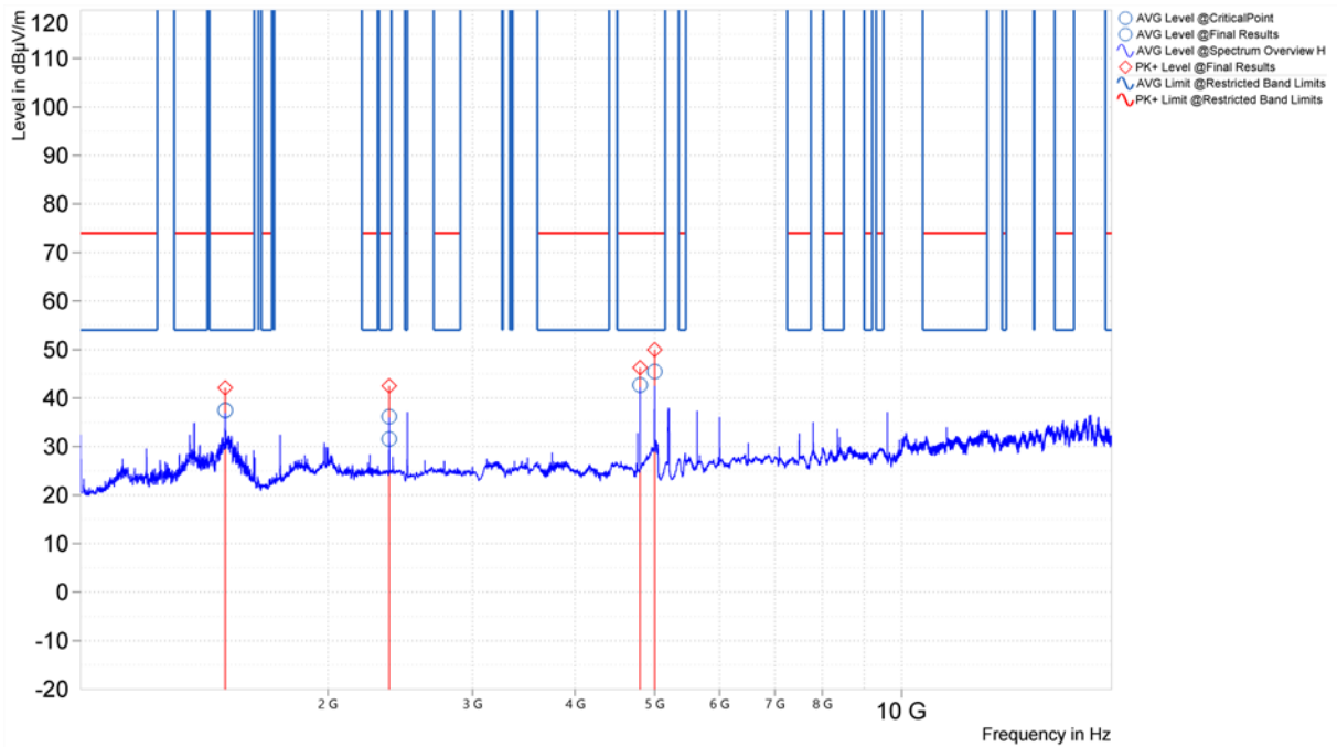
Figure 18. Worst Case Spurious Emissions, 1GHz – 18GHz, 802.11n, Horizontal (U-NII-1, Middle Channel)
