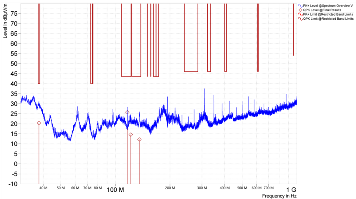
Figure 17. Worst Case Spurious Emissions, 30MHz – 1GHz, 802.11n, Vertical (U-NII-1, Middle Channel)
