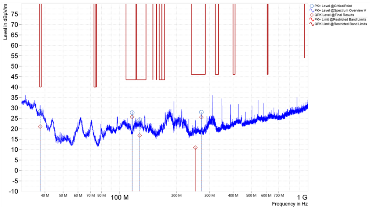
Figure 9. Worst Case Spurious Emissions, 30MHz – 1GHz, 802.11a, Vertical (U-NII-1, Middle Channel)
