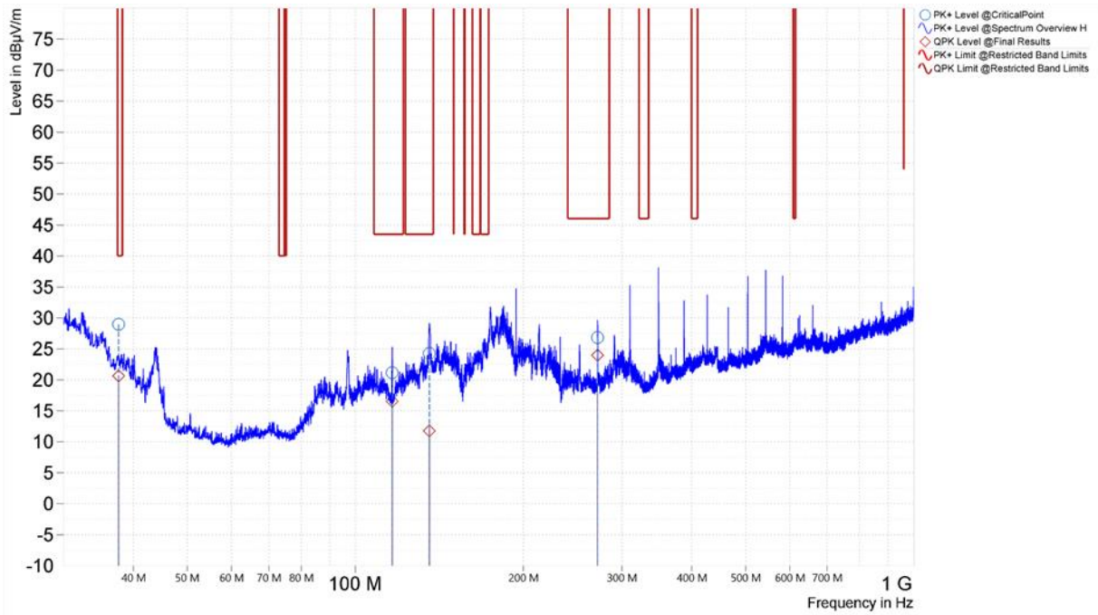
Figure 8. Worst Case Spurious Emissions, 30MHz – 1GHz, 802.11a, Horizontal (U-NII-1, Middle Channel)
