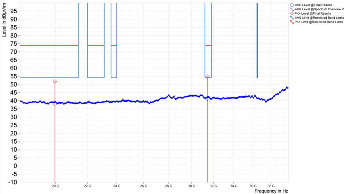
Figure 37. Worst Case Spurious Emissions, 18GHz – 40GHz, 802.11n, Vertical (U-NII-2A, Middle Channel)
