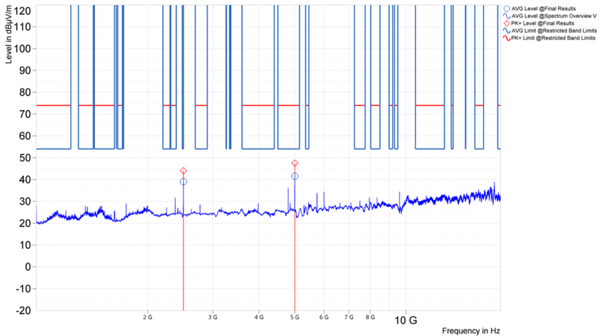
Figure 27. Worst Case Spurious Emissions, 1GHz – 18GHz, 802.11a, Vertical (U-NII-2A, Middle Channel)
