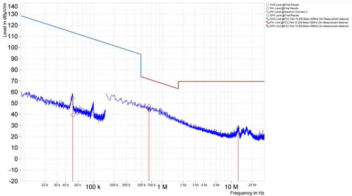
Figure 15. Worst Case Spurious Emissions, 9kHz – 30MHz, 802.11n, Coaxial Loop (U-NII-1, Middle Channel)
