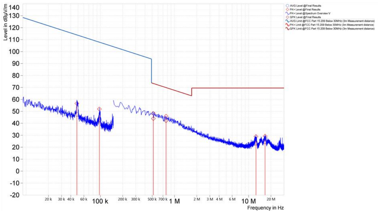
Figure 23. Worst Case Spurious Emissions, 9kHz – 30MHz, 802.11a, Coaxial Loop (U-NII-2A, Middle Channel)
