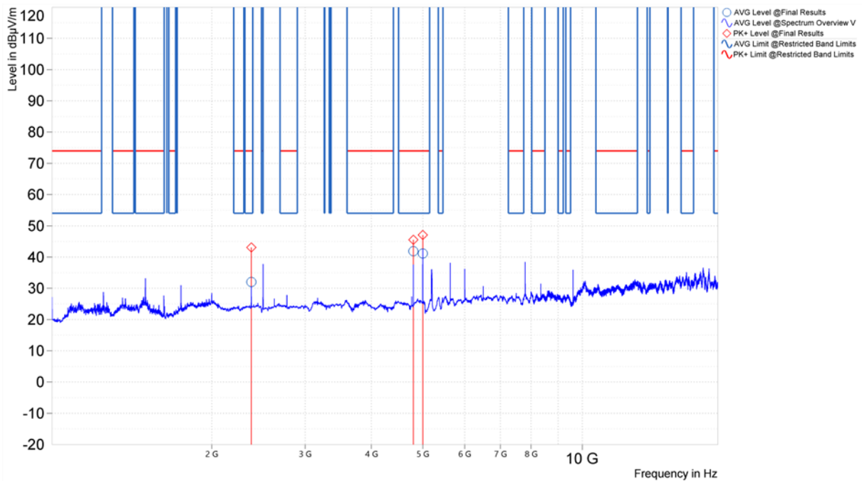
Figure 11. Worst Case Spurious Emissions, 1GHz – 18GHz, 802.11a, Vertical (U-NII-1, Middle Channel)
