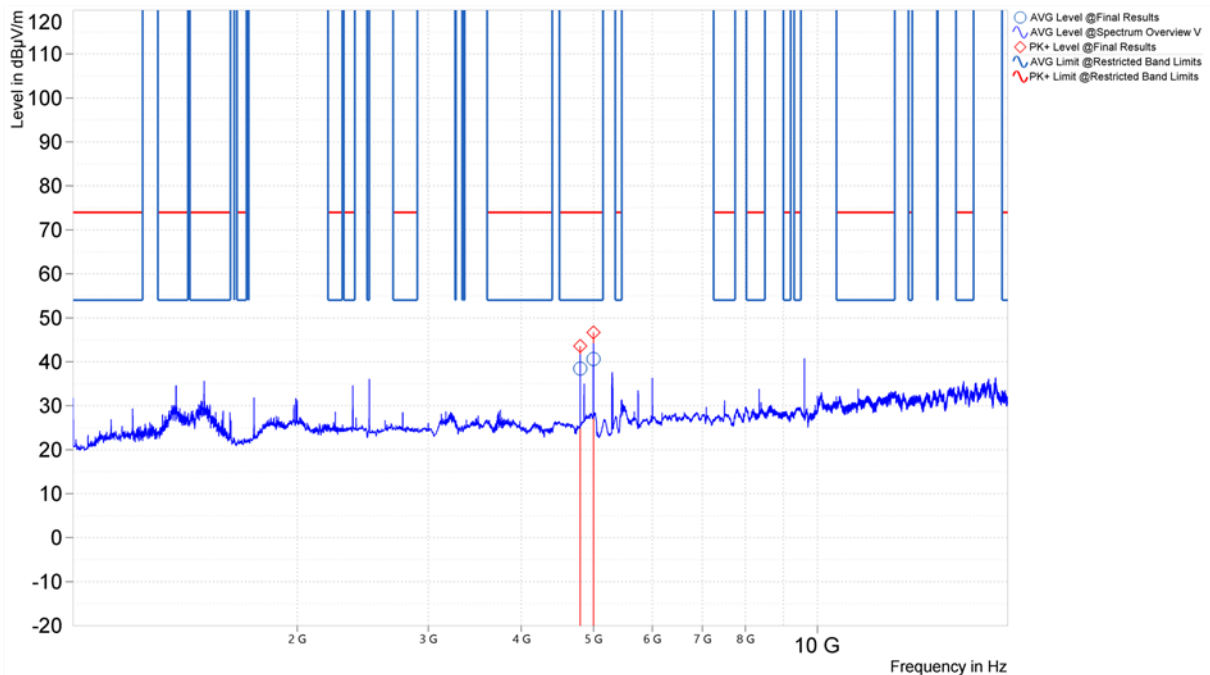
Figure 35. Worst Case Spurious Emissions, 1GHz – 18GHz, 802.11n, Vertical (U-NII-2A, Middle Channel)
