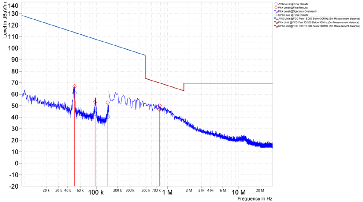
Figure 14. Worst Case Spurious Emissions, 9kHz – 30MHz, 802.11n, Coplanar Loop (U-NII-1, Middle Channel)
