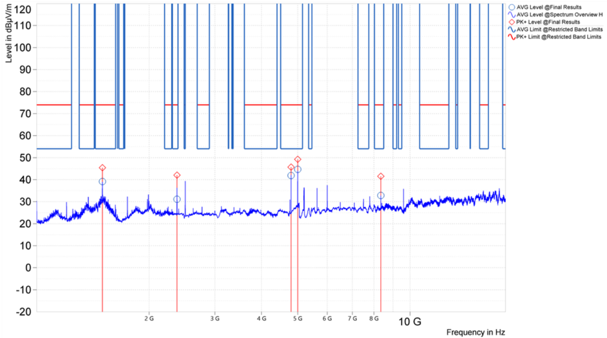
Figure 10. Worst Case Spurious Emissions, 1GHz – 18GHz, 802.11a, Horizontal (U-NII-1, Middle Channel)
