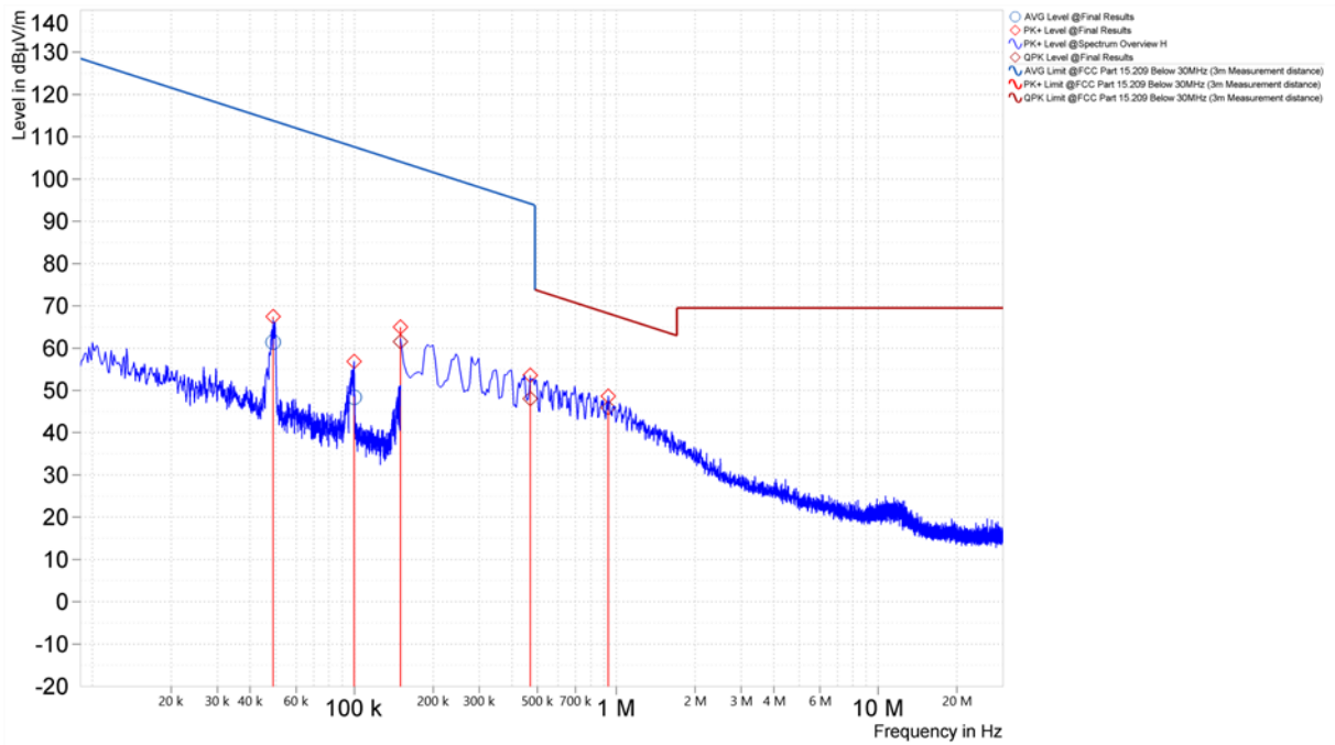
Figure 22. Worst Case Spurious Emissions, 9kHz – 30MHz, 802.11a, Coplanar Loop (U-NII-2A, Middle Channel)
