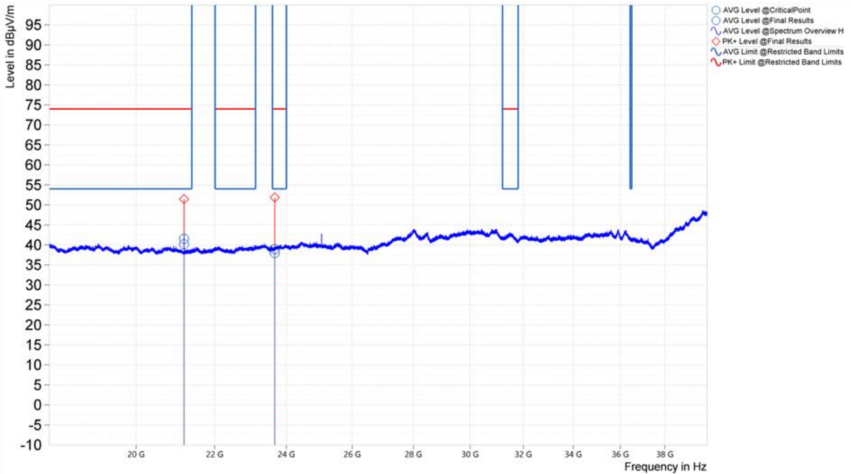
Figure 36. Worst Case Spurious Emissions, 18GHz – 40GHz, 802.11n, Horizontal (U-NII-2A, Middle Channel)
