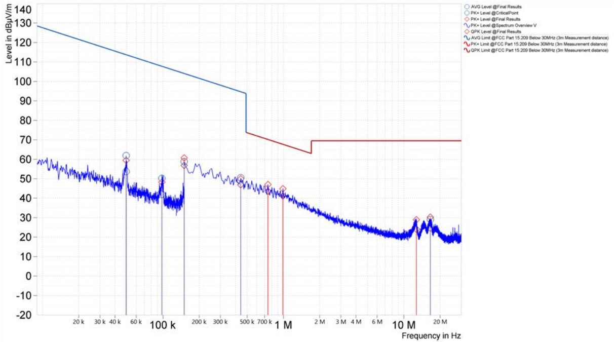
Figure 7. Worst Case Spurious Emissions, 9kHz – 30MHz, 802.11a, Coaxial Loop (U-NII-1, Middle Channel)
