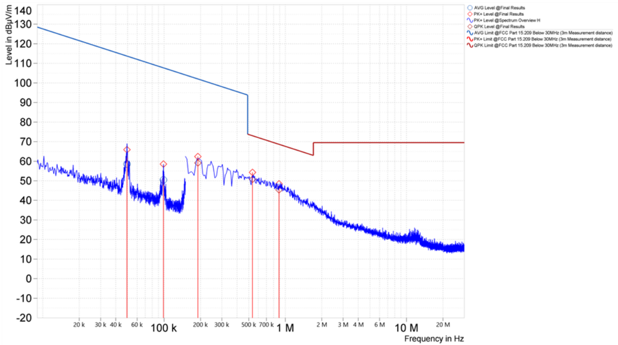
Figure 30. Worst Case Spurious Emissions, 9kHz – 30MHz, 802.11n, Coplanar Loop (U-NII-2A, Middle Channel)
