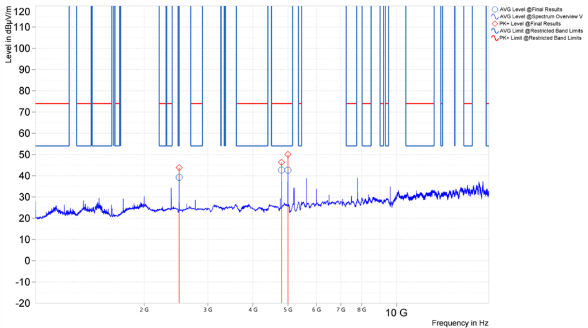
Figure 19. Worst Case Spurious Emissions, 1GHz – 18GHz, 802.11n, Vertical (U-NII-1, Middle Channel)
