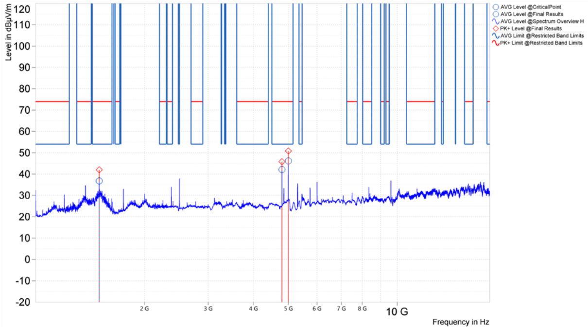
Figure 34. Worst Case Spurious Emissions, 1GHz – 18GHz, 802.11n, Horizontal (U-NII-2A, Middle Channel)
