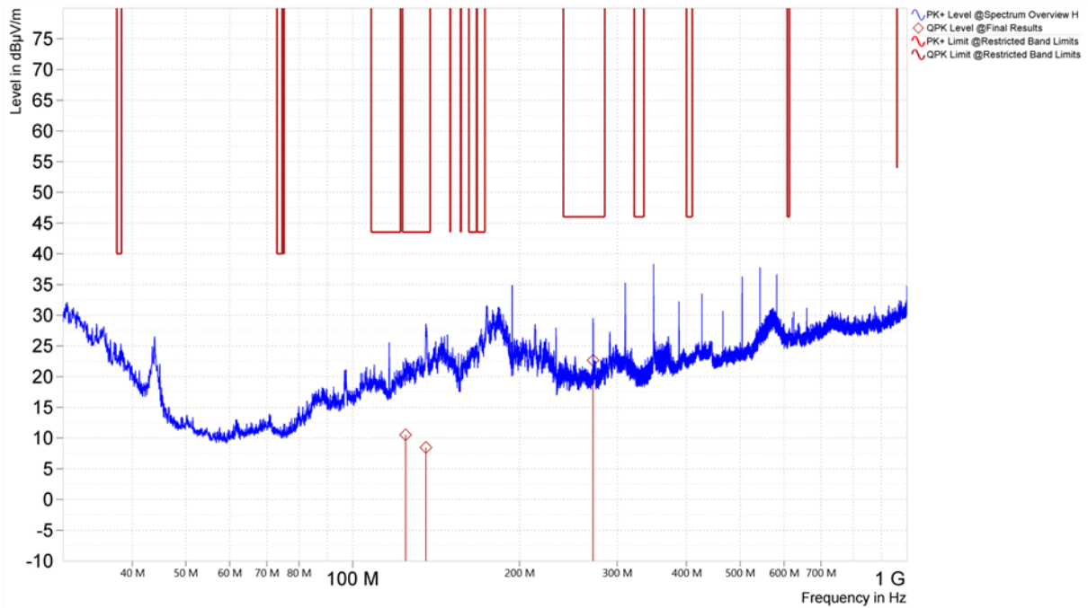
Figure 16. Worst Case Spurious Emissions, 30MHz – 1GHz, 802.11n, Horizontal (U-NII-1, Middle Channel)
