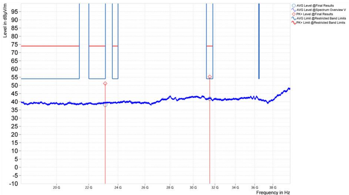
Figure 13. Worst Case Spurious Emissions, 18GHz – 40GHz, 802.11a, Vertical (U-NII-1, Middle Channel)
