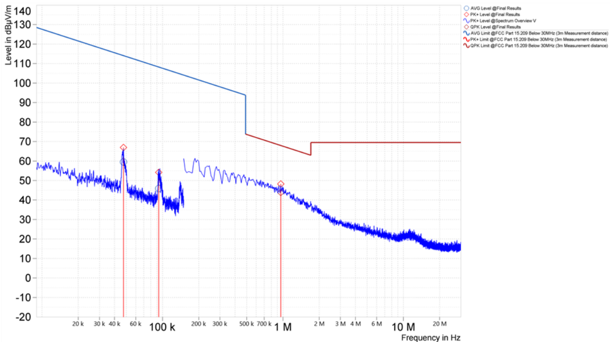
Figure 27. Worst Case Spurious Emissions, 9kHz – 30MHz, 8DPSK, Coaxial Loop (Middle Channel)
