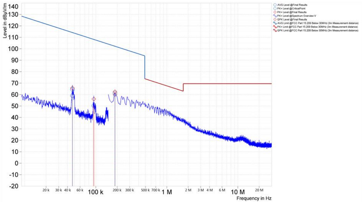
Figure 19. Worst Case Spurious Emissions, 9kHz – 30MHz, Pi/4DQPSK, Coaxial Loop (Middle Channel)
