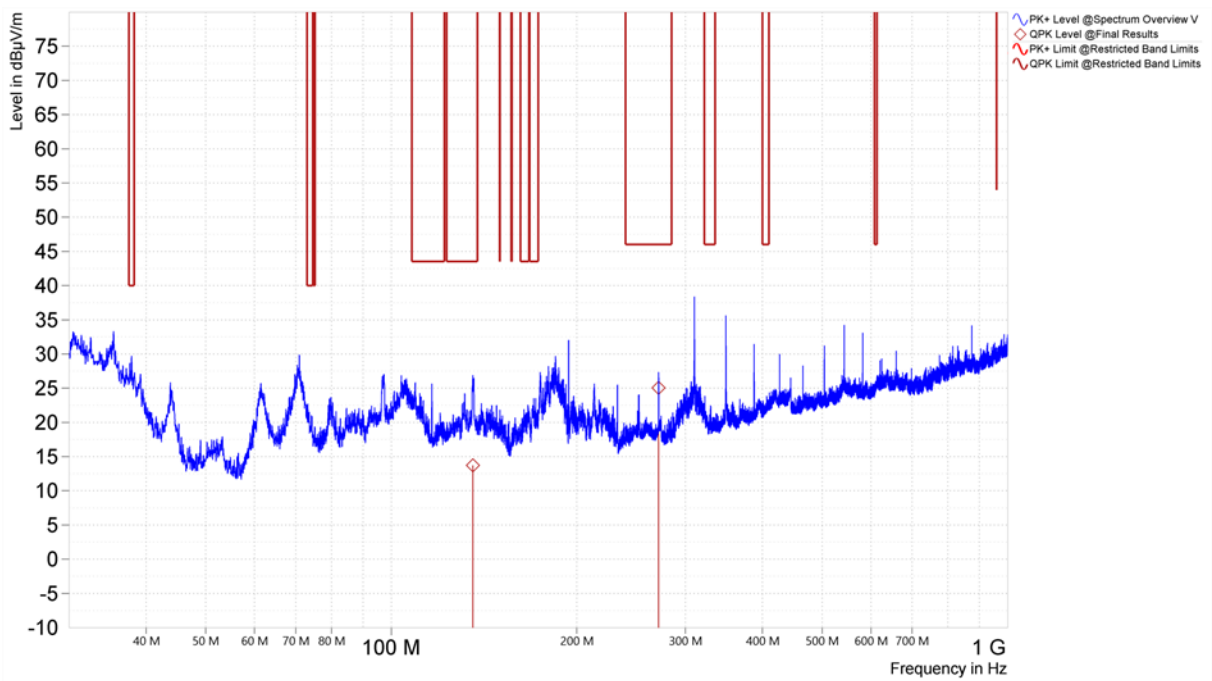
Figure 13. Worst Case Spurious Emissions, 30MHz – 1GHz, GFSK, Vertical Polarity (Middle Channel)
