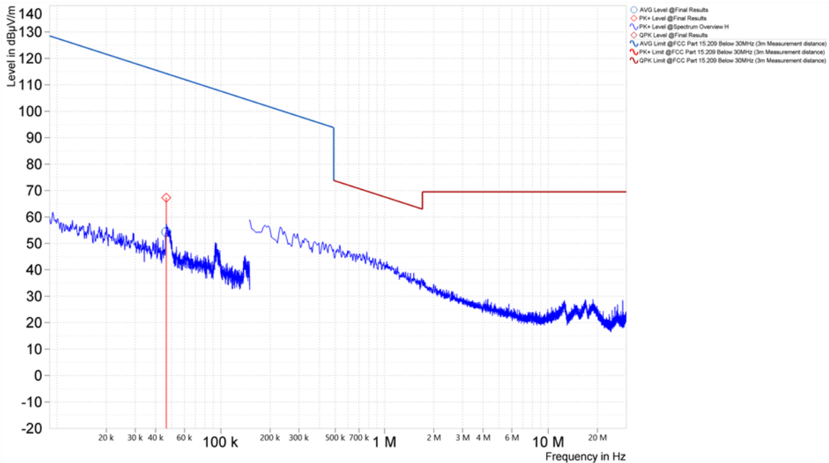
Figure 26. Worst Case Spurious Emissions, 9kHz – 30MHz, 8DPSK, Coplanar Loop (Middle Channel)
