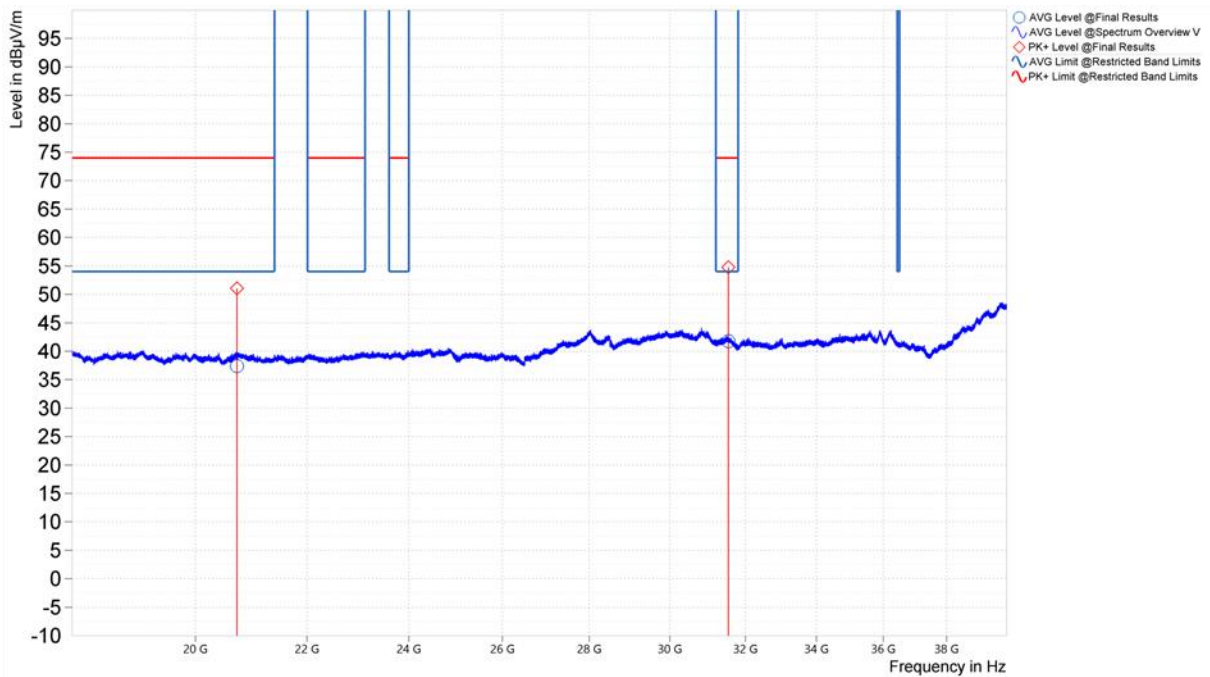
Figure 33. Worst Case Spurious Emissions, 18GHz – 40GHz, 8DPSK, Vertical Polarity (Middle Channel)
