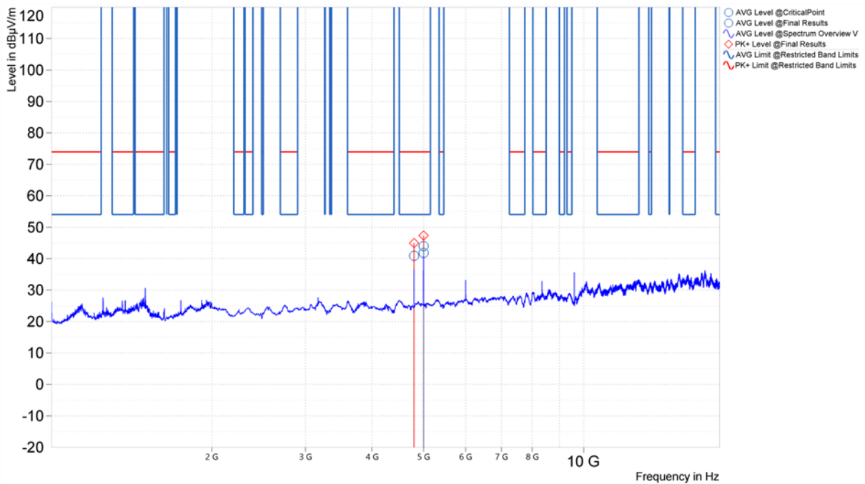
Figure 23. Worst Case Spurious Emissions, 1GHz – 18GHz, Pi/4DQPSK, Vertical Polarity (Middle Channel)
