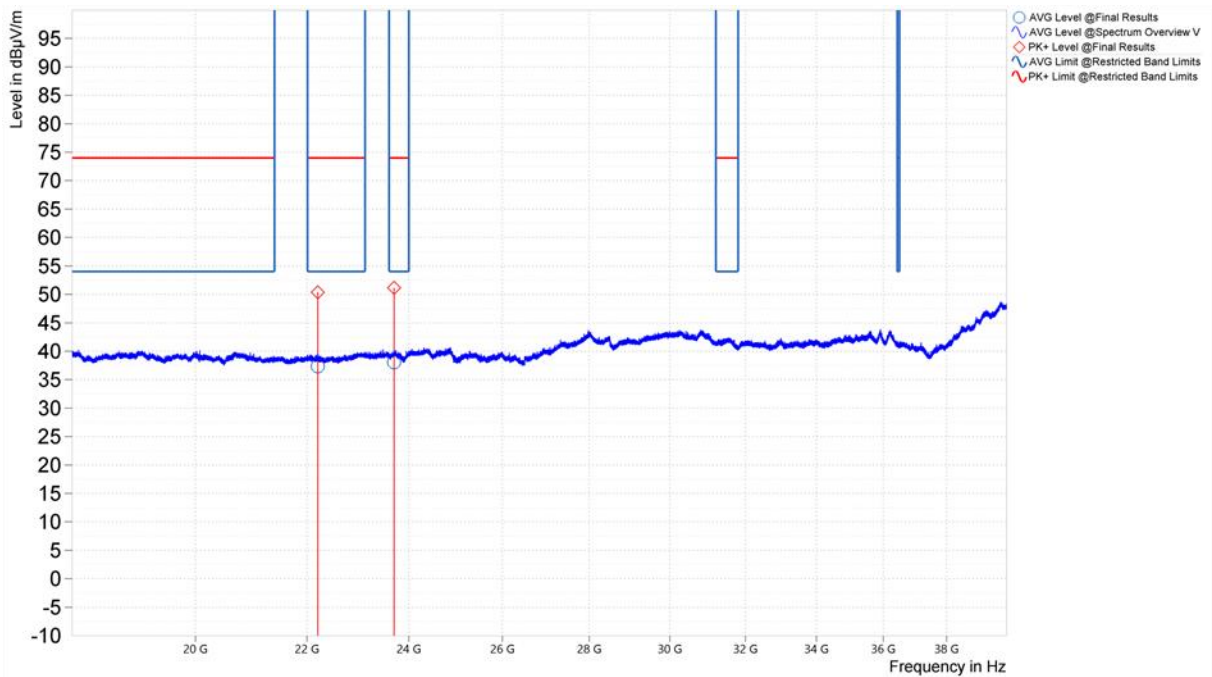
Figure 9. Worst Case Spurious Emissions, 18GHz – 40GHz, BLE, Vertical Polarity (Middle Channel)
