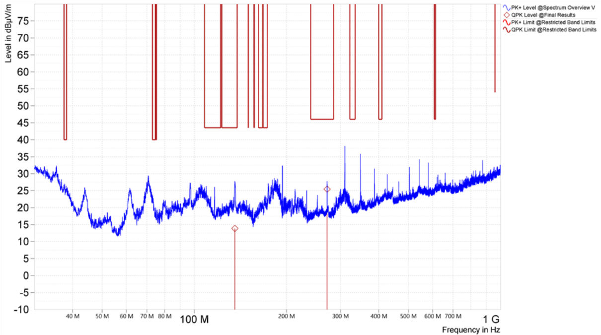
Figure 21. Worst Case Spurious Emissions, 30MHz – 1GHz, Pi/4DQPSK, Vertical Polarity (Middle Channel)
