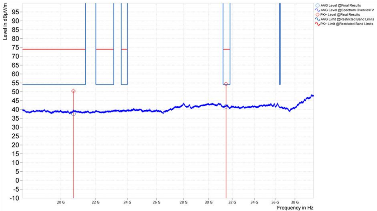
Figure 17. Worst Case Spurious Emissions, 18GHz – 40GHz, GFSK, Vertical Polarity (Middle Channel)
