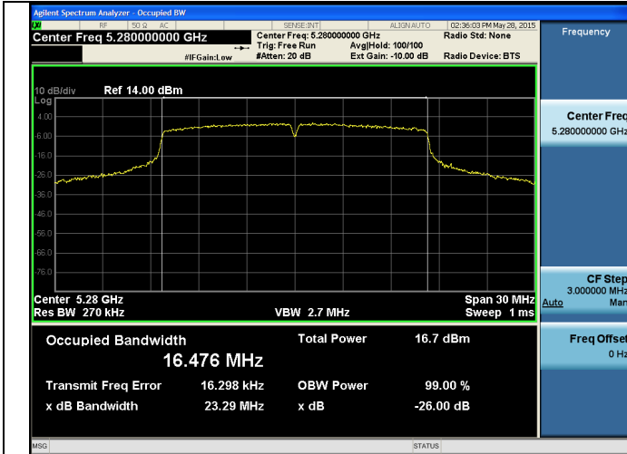
Channel 56 - 802.11a
