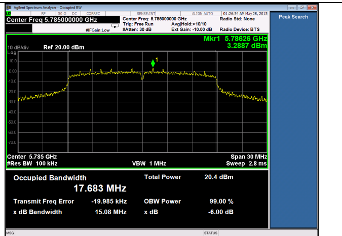
Channel 157 – 802.11n
