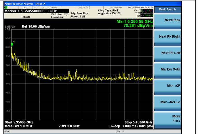
Channel 64 - 802.11n - Peak
