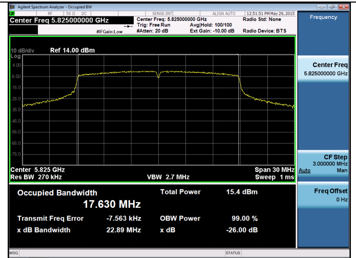
Channel 165 – 802.11n
