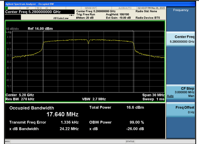
Channel 56 - 802.11n
