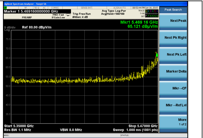
Channel 100 – 802.11a – Peak RB
