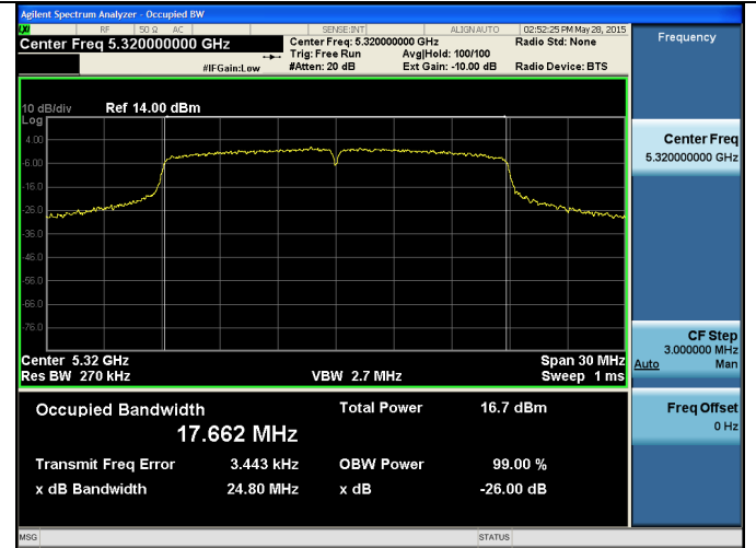
Channel 64 - 802.11n
