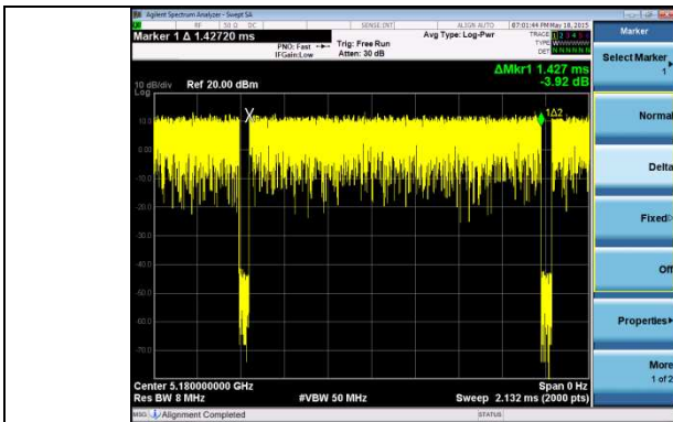
802.11a – On-time
