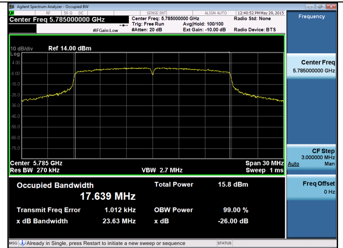
Channel 157 – 802.11n
