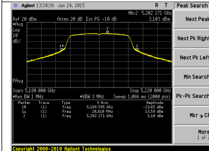
Channel 40 – 802.11a
