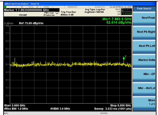
5.9-8 GHz – Channel 165
