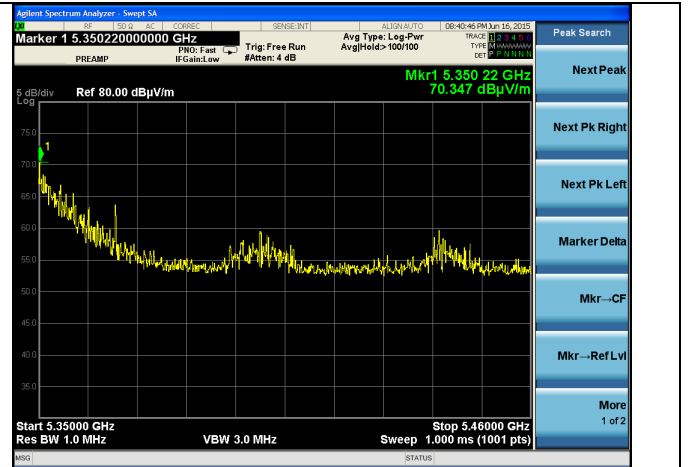
Channel 64 - 802.11a - Peak
