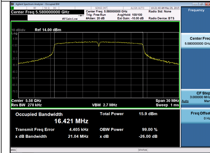
Channel 116 - 802.11a
