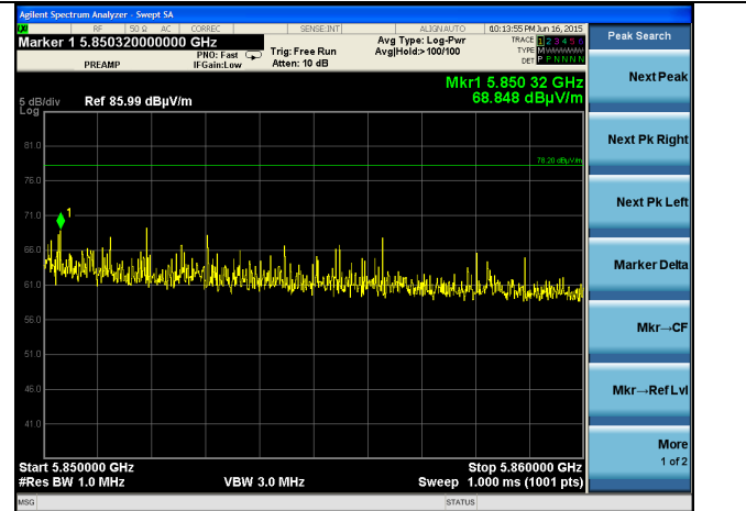
Channel 165 – 802.11n – Peak
