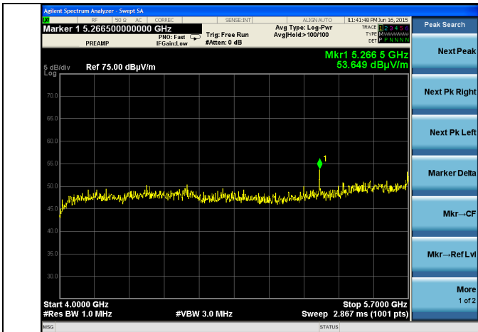
4-5.7 GHz – Channel 149
