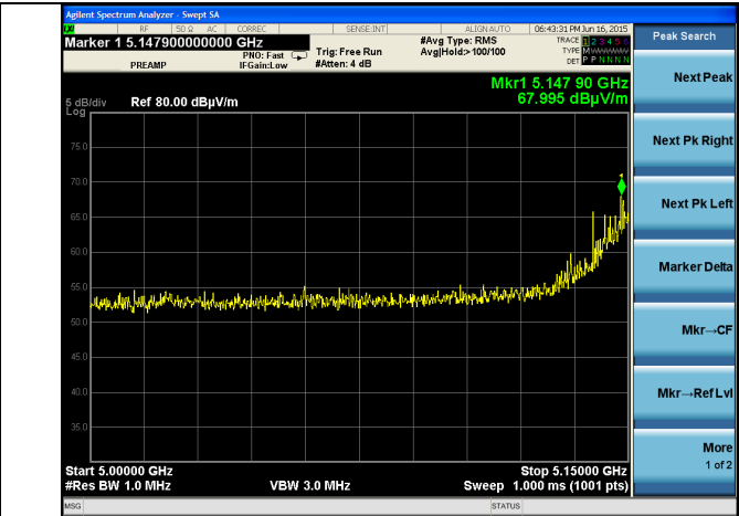
Channel 36 - 802.11a - Peak
