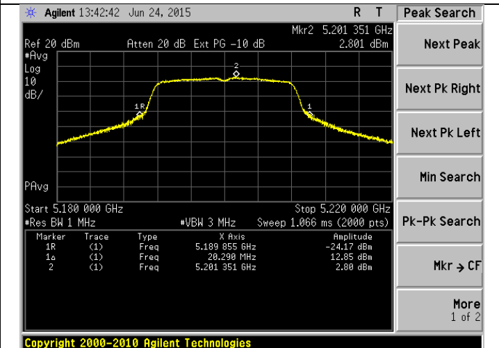
Channel 40 – 802.11n
