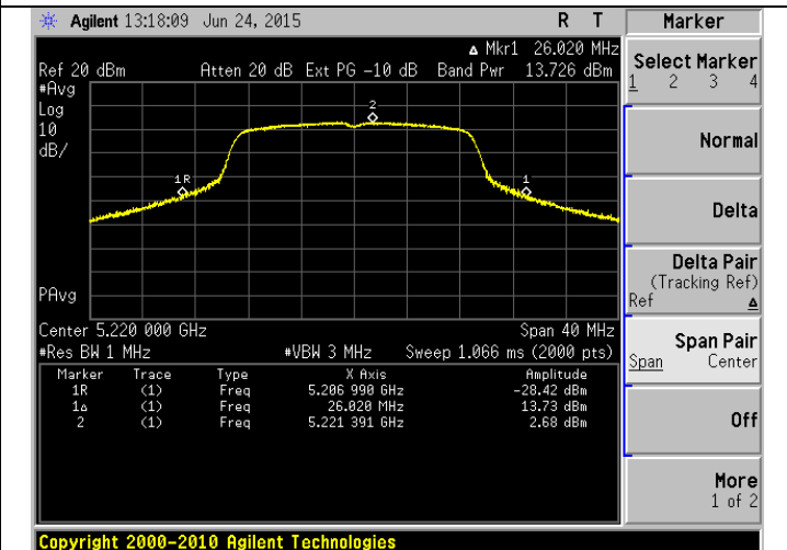
Channel 44 – 802.11n
