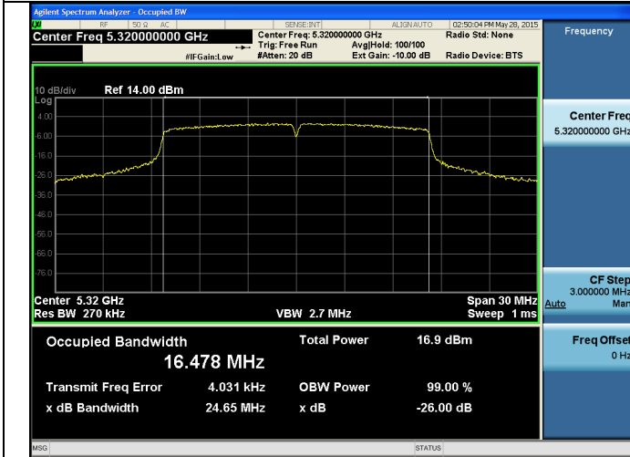
Channel 64 - 802.11a
