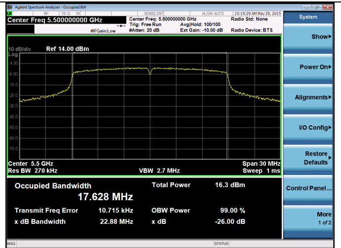
Channel 100 - 802.11n
