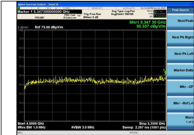
4-5.35 GHz – Channel 100
