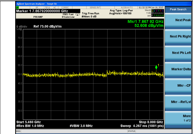
5.46-8 GHz – Channel 64
