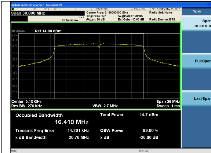
Channel 36 - 802.11a
