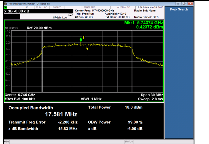
Channel 149 – 802.11n
