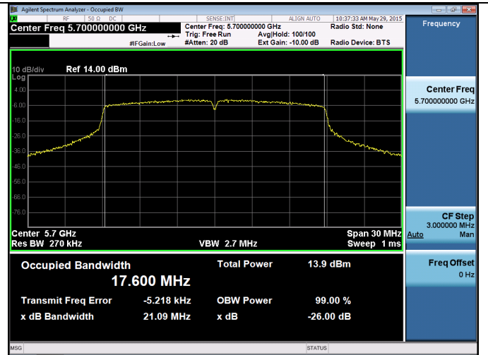
Channel 140 - 802.11n
