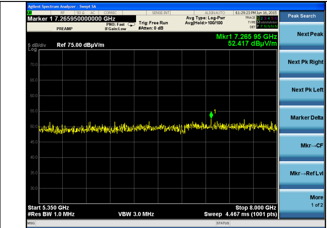
5.35-8 GHz – Channel 44
