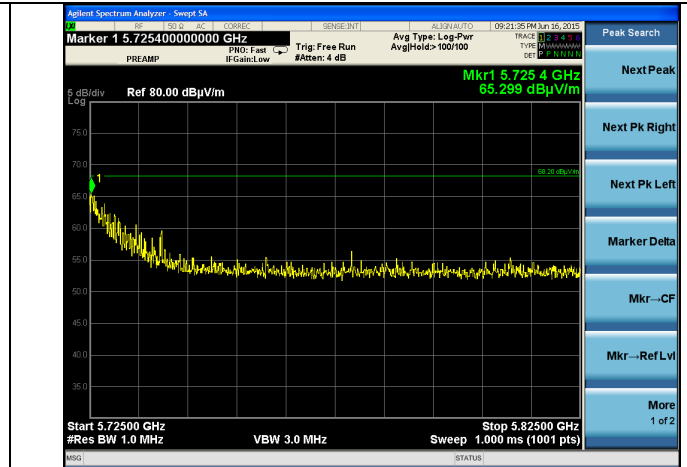
Channel 140 – 802.11n – Peak
