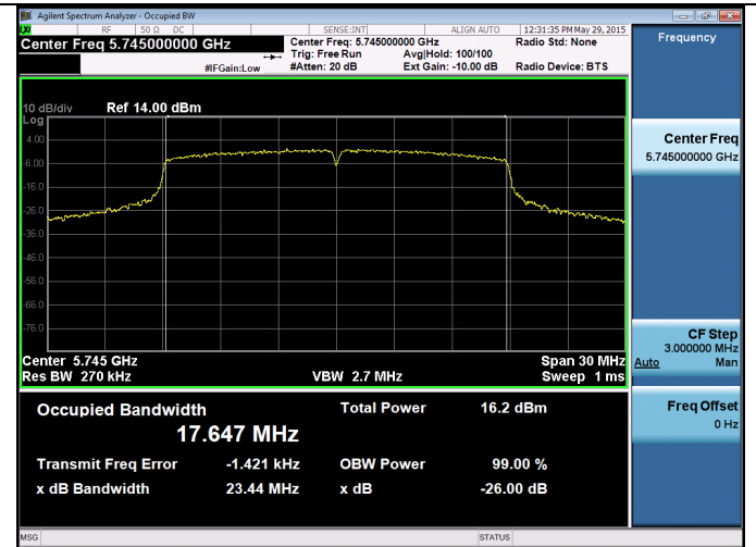
Channel 149 – 802.11n
