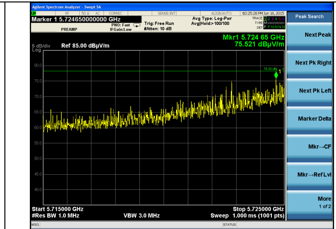
Channel 149 – 802.11n – Peak
