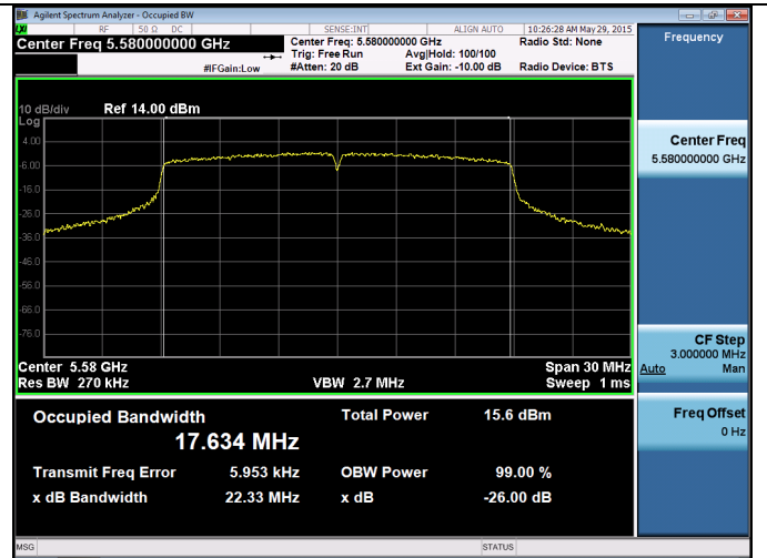
Channel 116 - 802.11n
