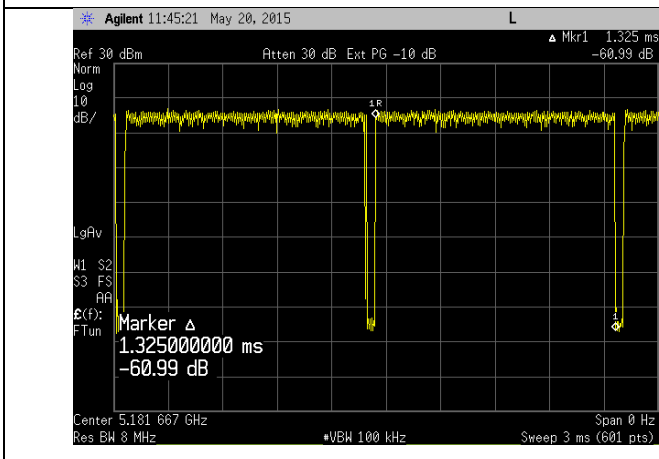
802.11n – On-time
