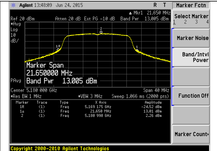
Channel 36 – 802.11n
