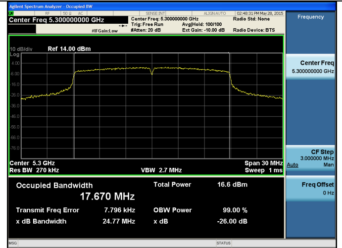
Channel 60 - 802.11n
