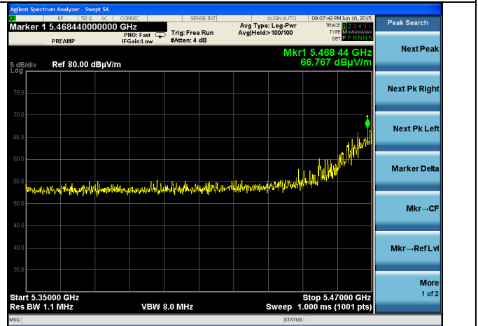
Channel 100 – 802.11n – Peak RB
