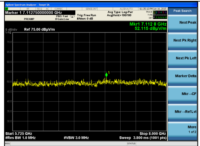
5.725-8 GHz – Channel 140
