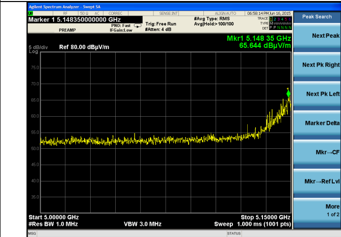
Channel 36 - 802.11n - Peak
