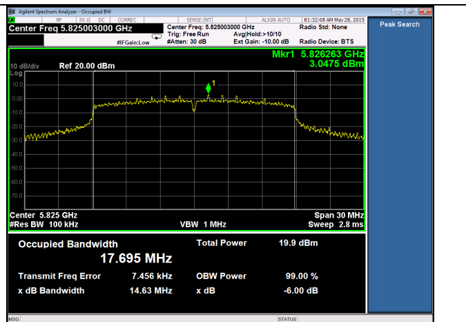
Channel 165 – 802.11n
