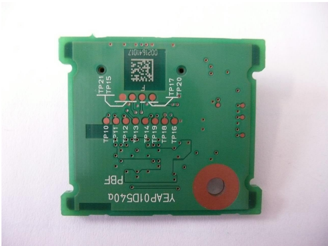
Memory-PCB-02
