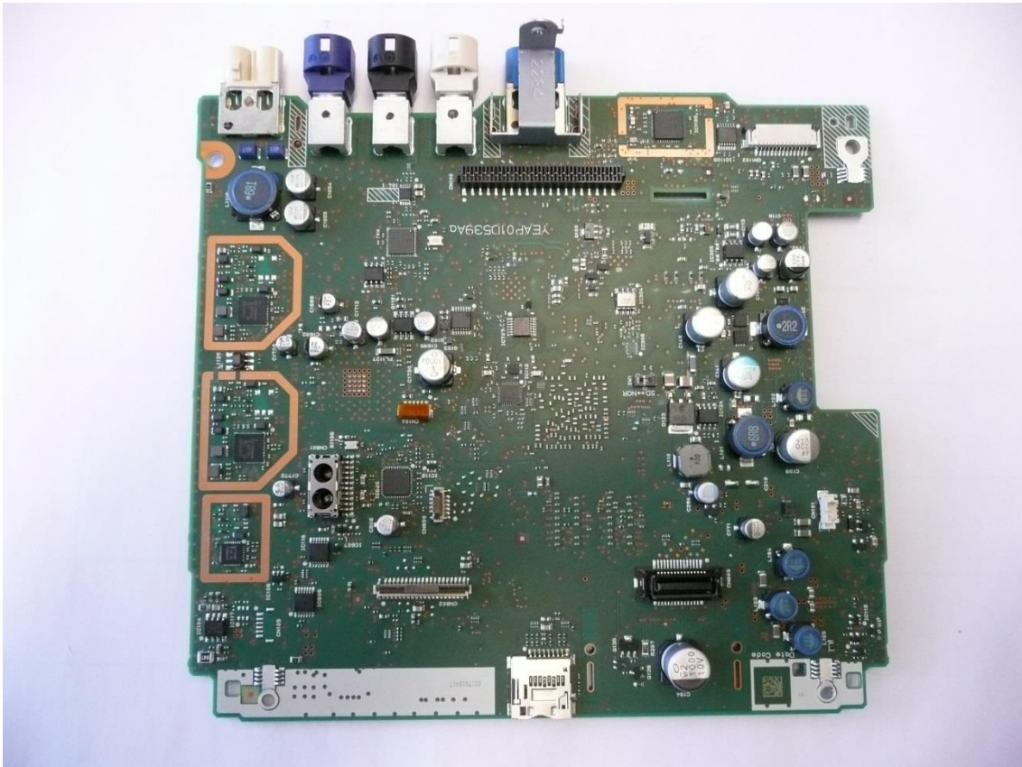
Main-PCB-03
