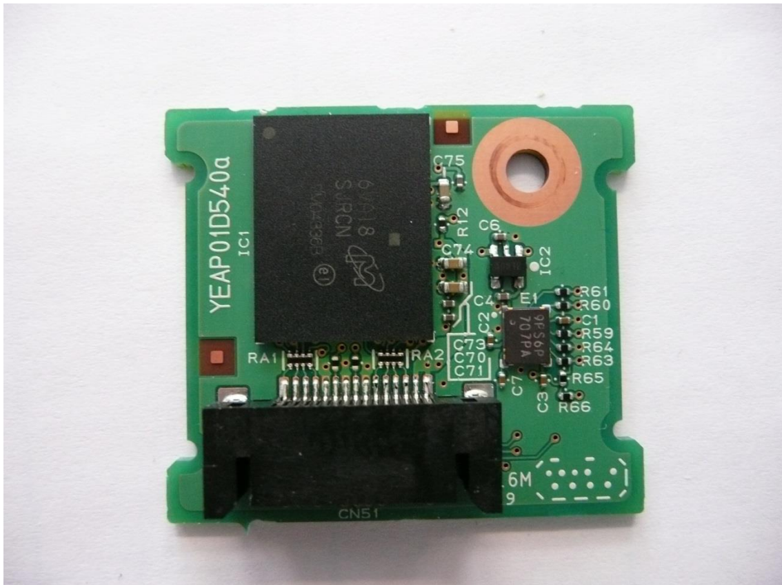
Memory-PCB-02
