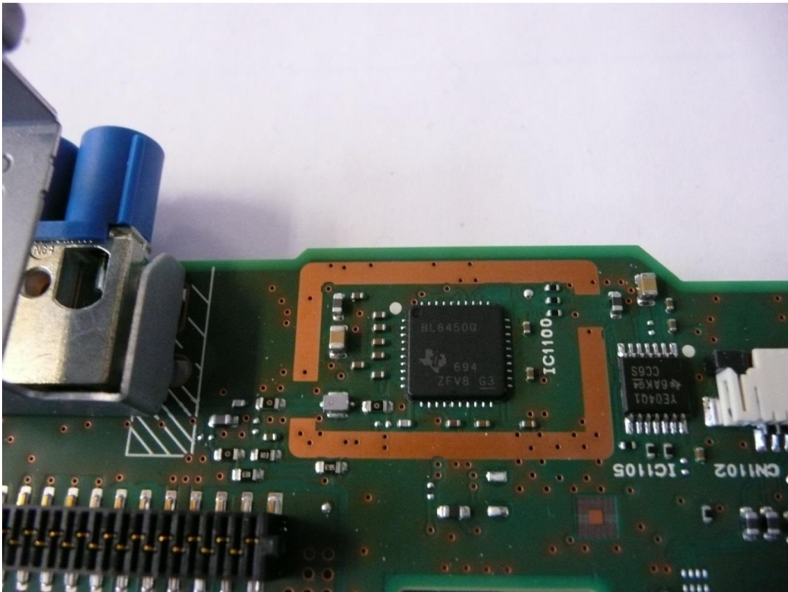
Main-PCB-04
