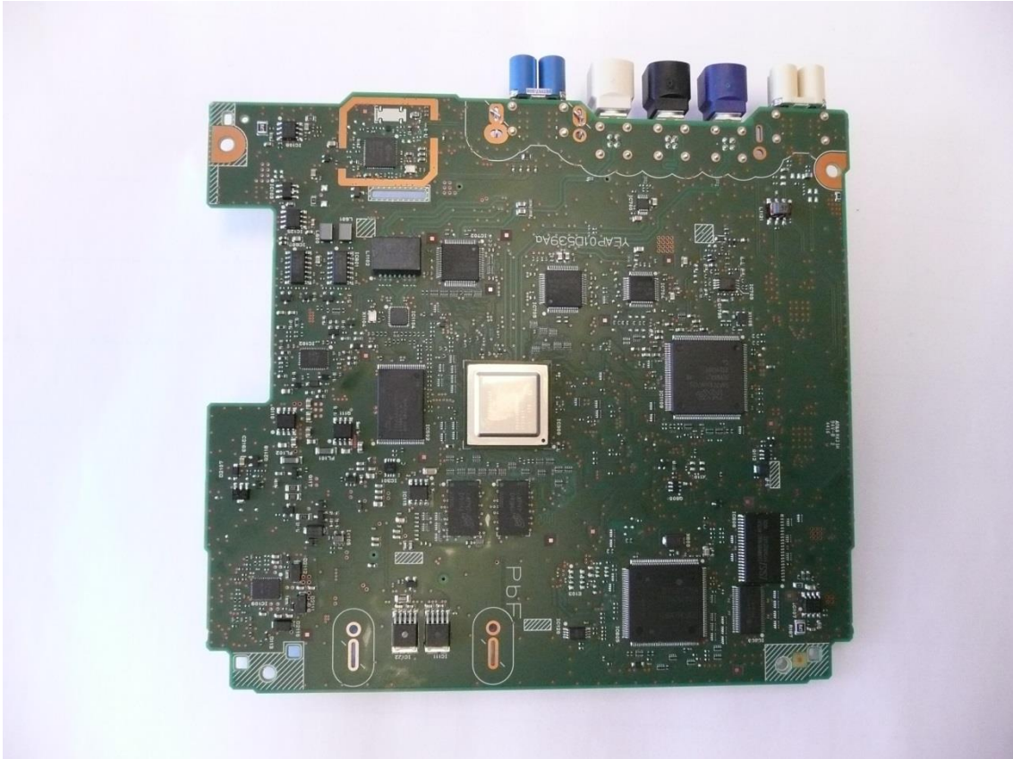
Main-PCB-04
