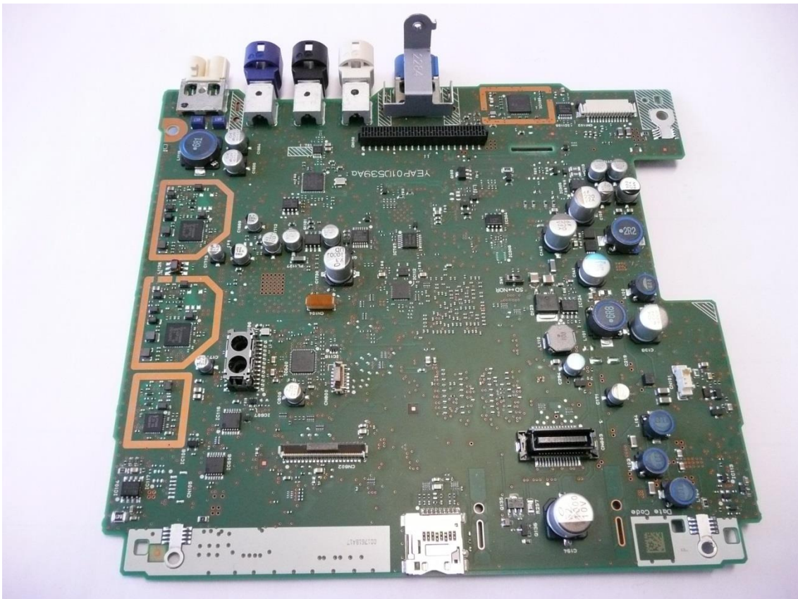
Main-PCB-02
