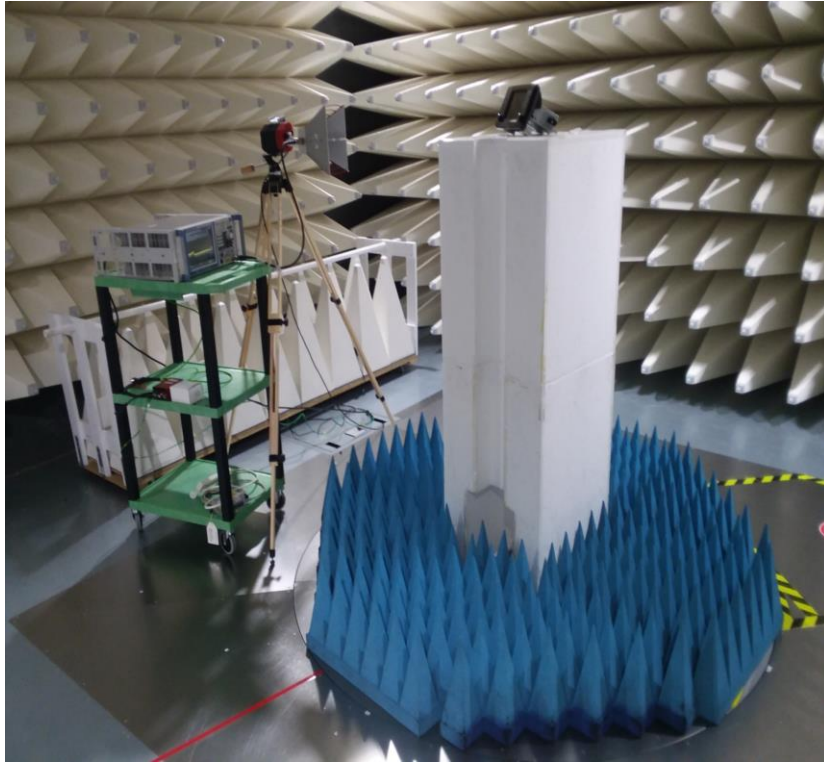
Figure B5. Radiated Setup
