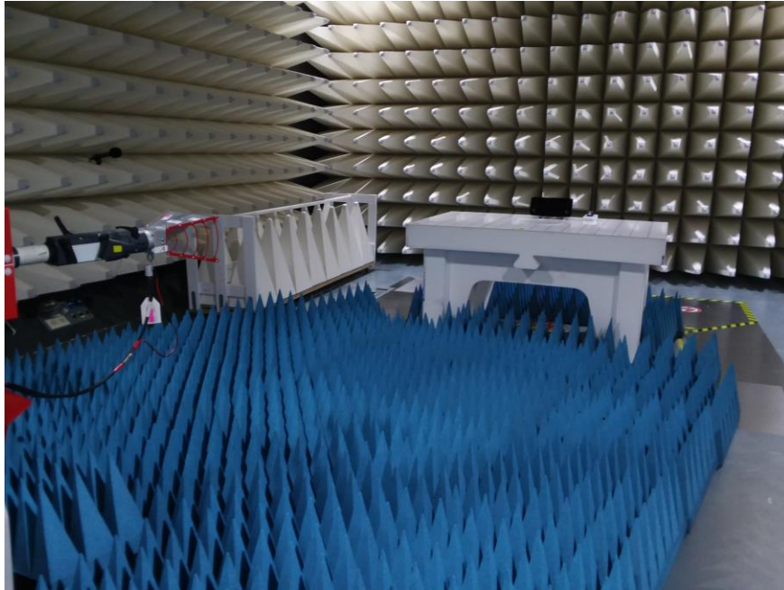
Figure B5. Radiated Setup – High Range
