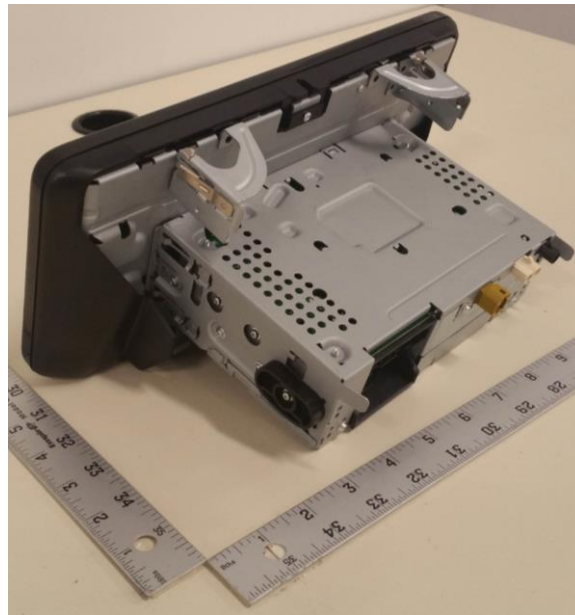
Figure B3. DUT Side Rear view2
