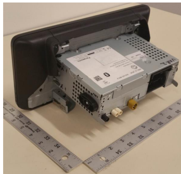
Figure B2. DUT Side Rear view1
