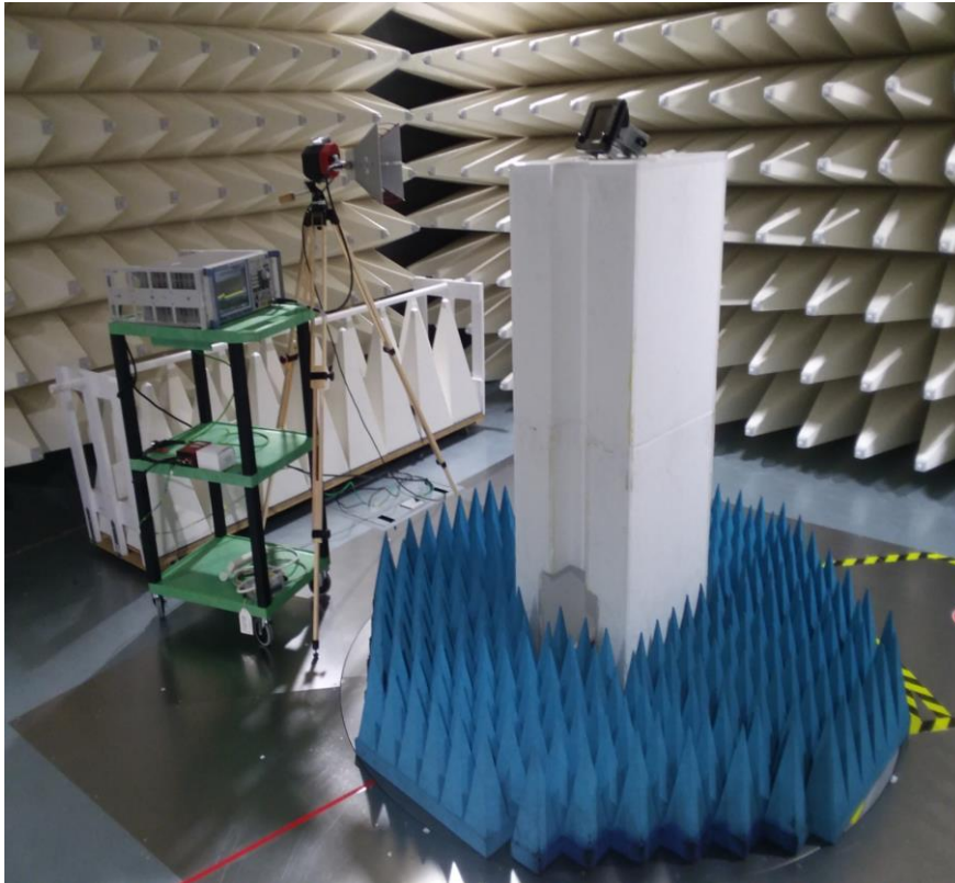
Figure B5. Radiated Setup
