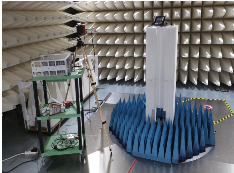
Figure B4. Radiated Test Setup
