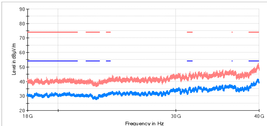
RF_FCC_15.407_E Field_18GHz_40GHz
