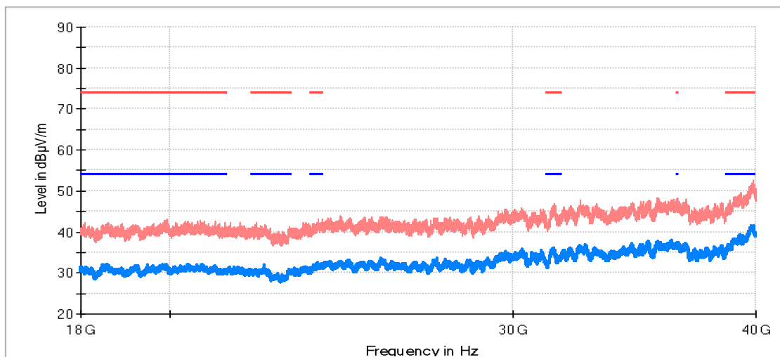
RF_FCC_15.407_E Field_18GHz_40GHz
