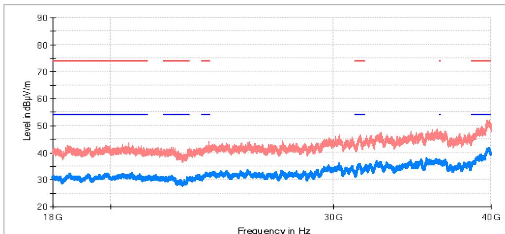
RF_FCC_15.407_E Field_18GHz_40GHz
