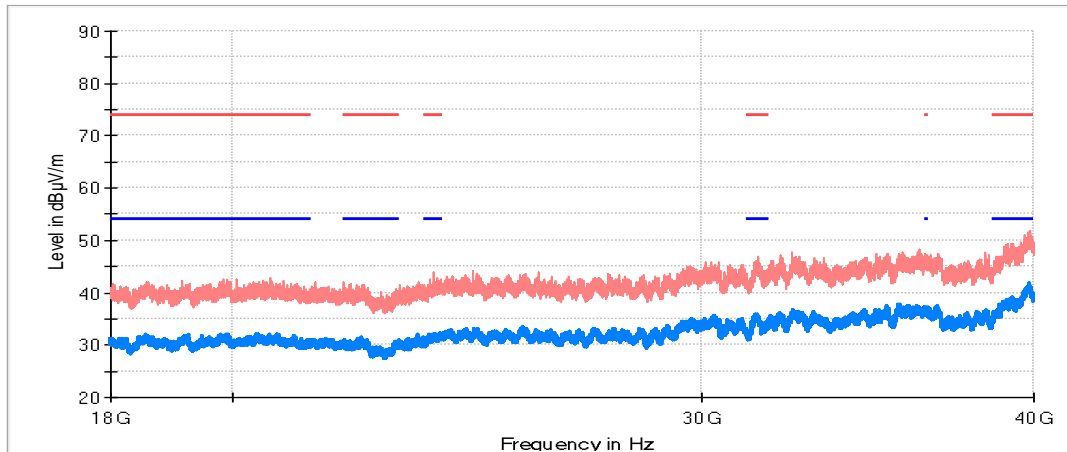
RF_FCC_15.407_E Field_18GHz_40GHz
