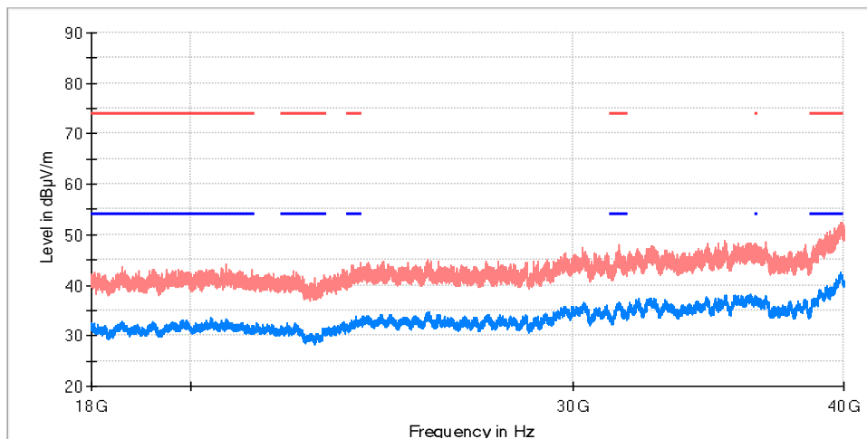
RF_FCC_15.407_E Field_18GHz_40GHz
