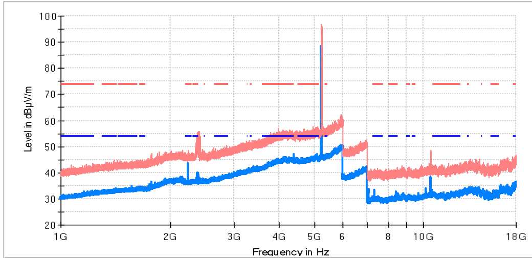
RF_FCC_15.407_E Field_1GHz_18GHz
