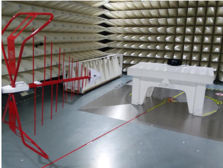
Figure B3. Radiated Setup – Low Range
