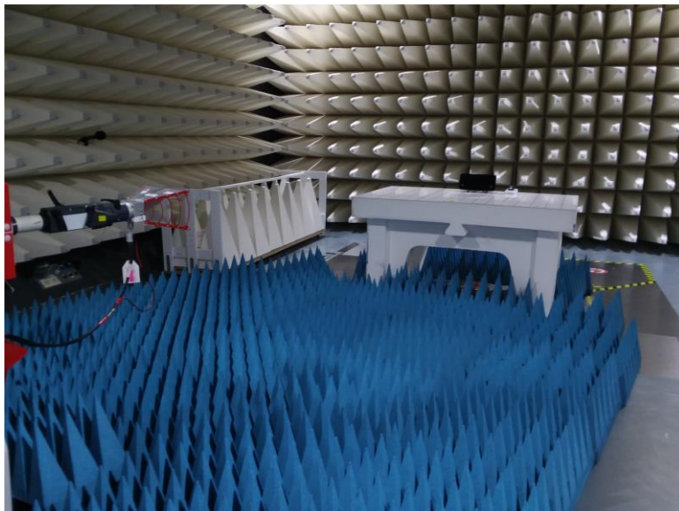
Figure B4. Radiated Setup – High Range
