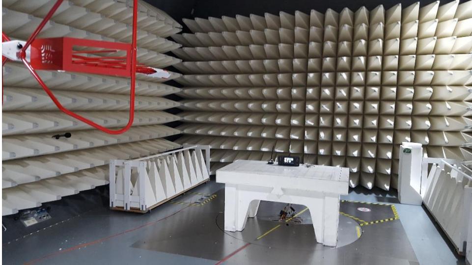
Figure B6. Radiated Emission test setup LR (0.03 – 1GHz)
