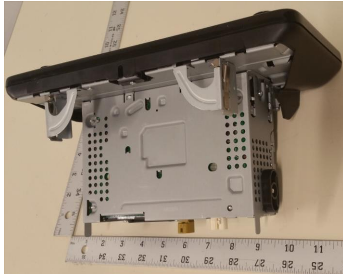
Figure B3. DUT Side Rear view2
