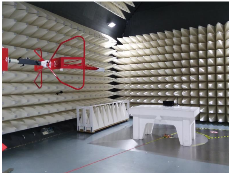
Figure B4. Radiated Setup – Low Range
