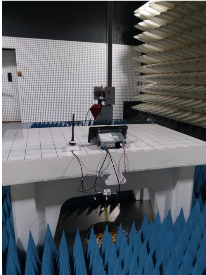
Figure B5. Radiated Setup – High Range
