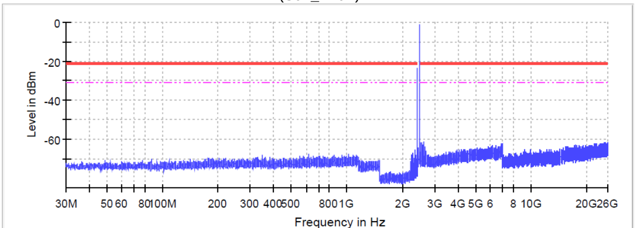
Radio Technology = Bluetooth EDR 2, Operating Frequency = high (S01_AA01)
