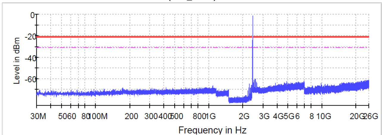
Radio Technology = Bluetooth EDR 2, Operating Frequency = mid (S01_AA01)
