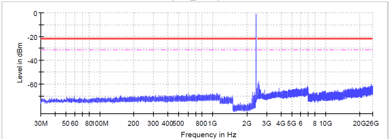
Radio Technology = Bluetooth EDR 2, Operating Frequency = low (S01_AA01)
