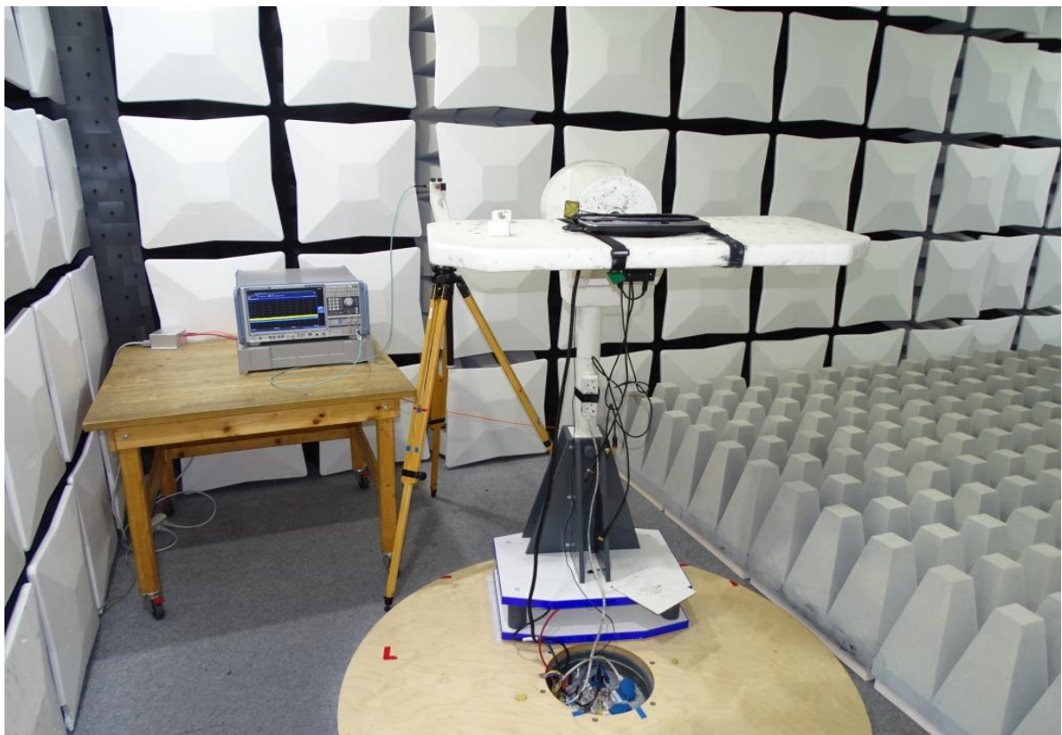
Photo 4: Test setup for radiated measurements above 26 GHz
