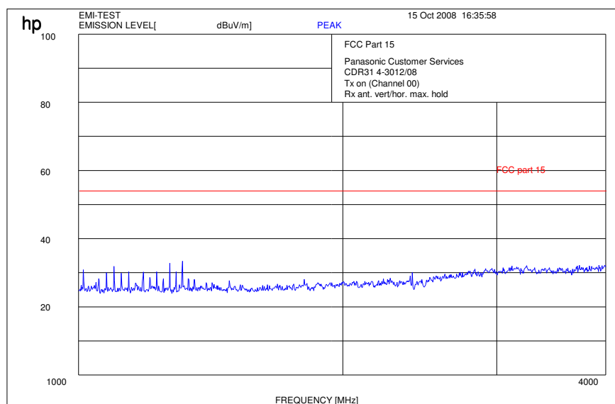
Plot 2: 1 - 4 GHz vertical worst case (lowest channel)
