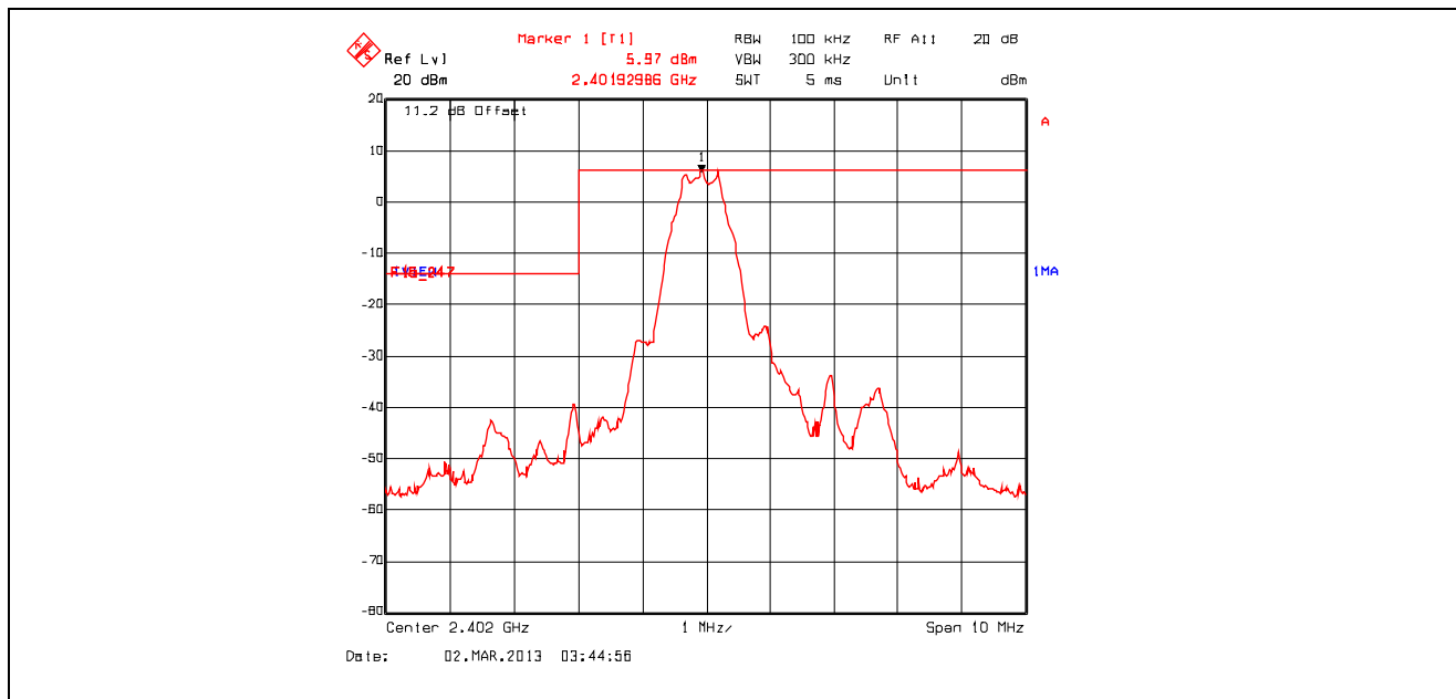
Plot 5.4.4.1.1. Band-Edge RF Conducted Emissions, Length 37 bytes, Bit pattern 0 (Pseudo-random bit sequence 9) Low End of Frequency Band, 2402 MHz
