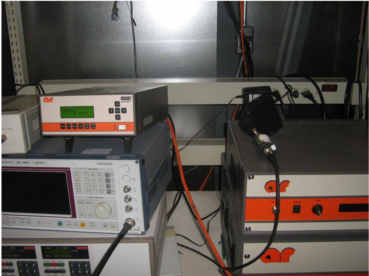
Figure 3: RF Power conducted tests
