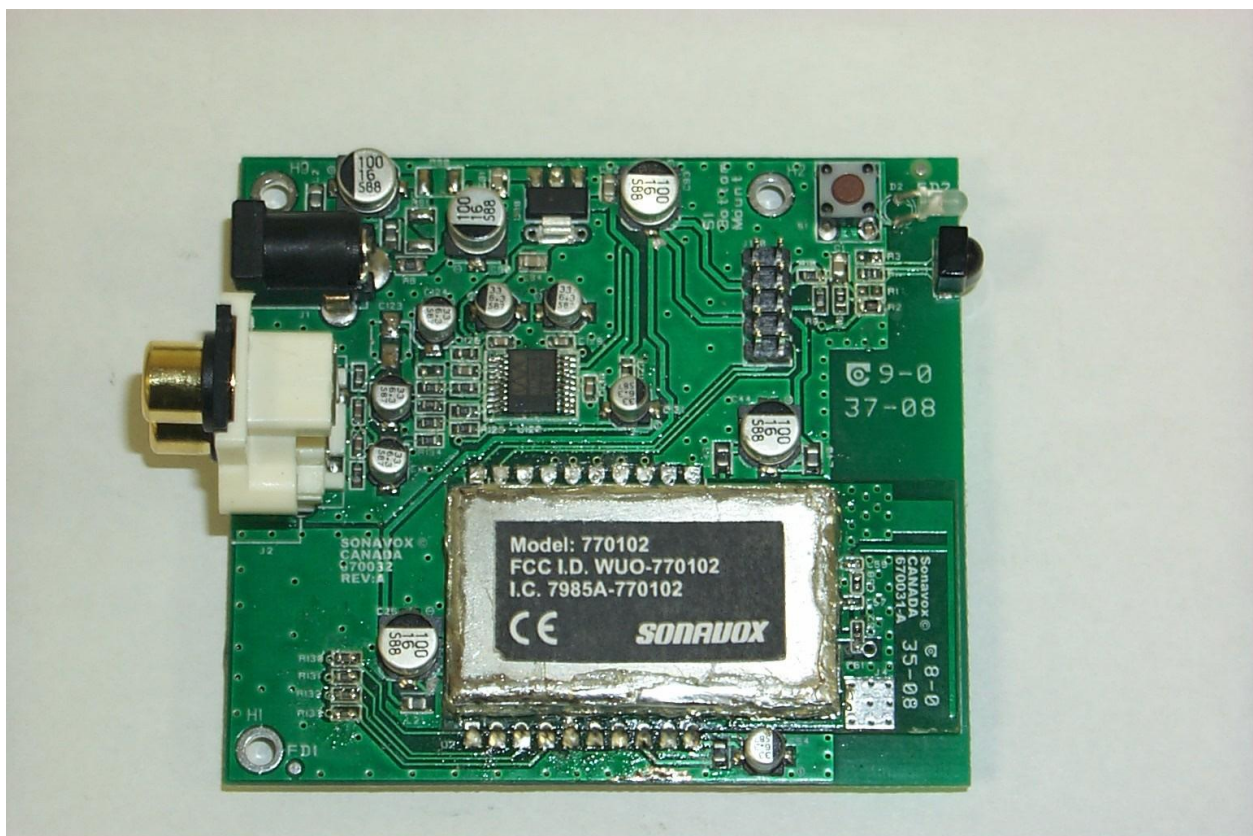
Figure 3: Audio module
