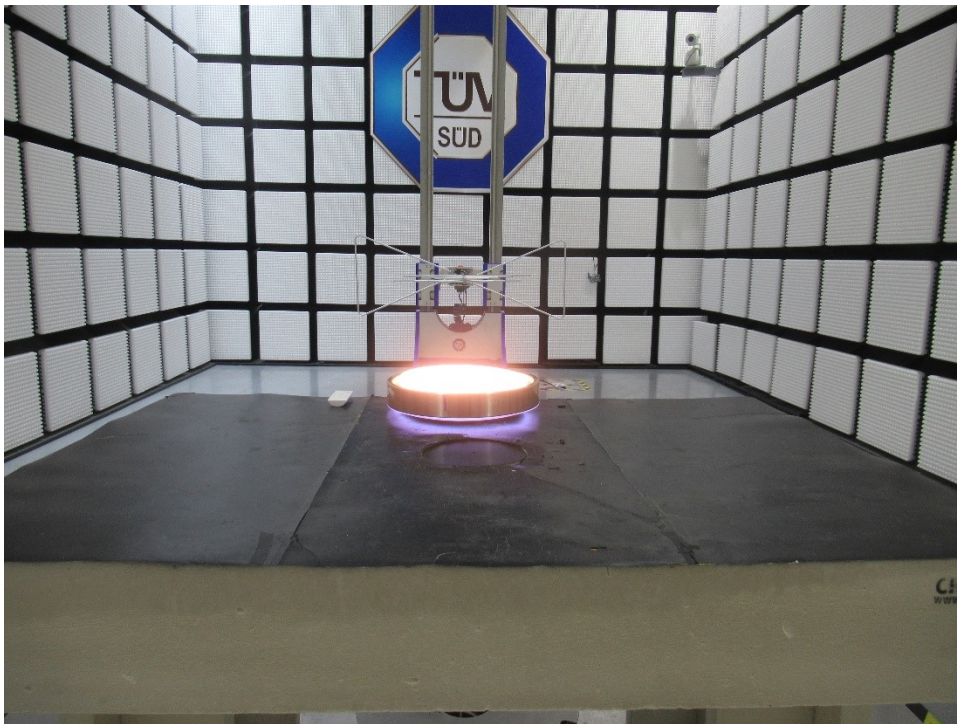
Radiated Emission test (1# Test Site) Below 1GHz
