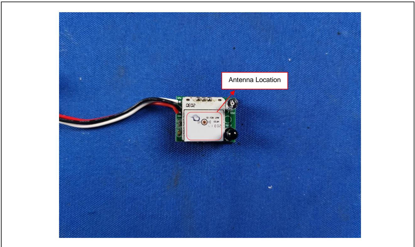
Details of: Inside view of sensor
