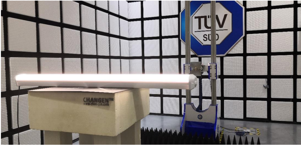
Radiated Emission test 1-18GHz
