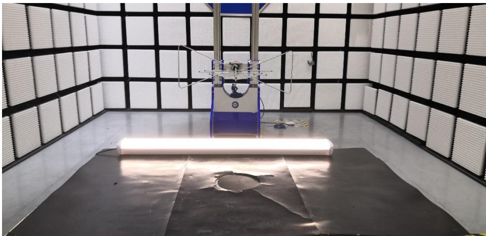
Radiated Emission test Below 1GHz
