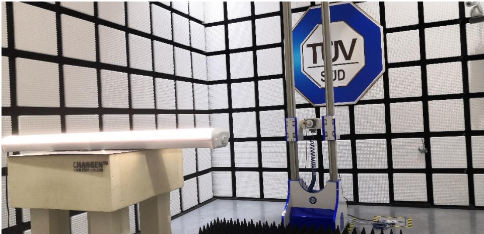
Radiated Emission test 18-40GHz
