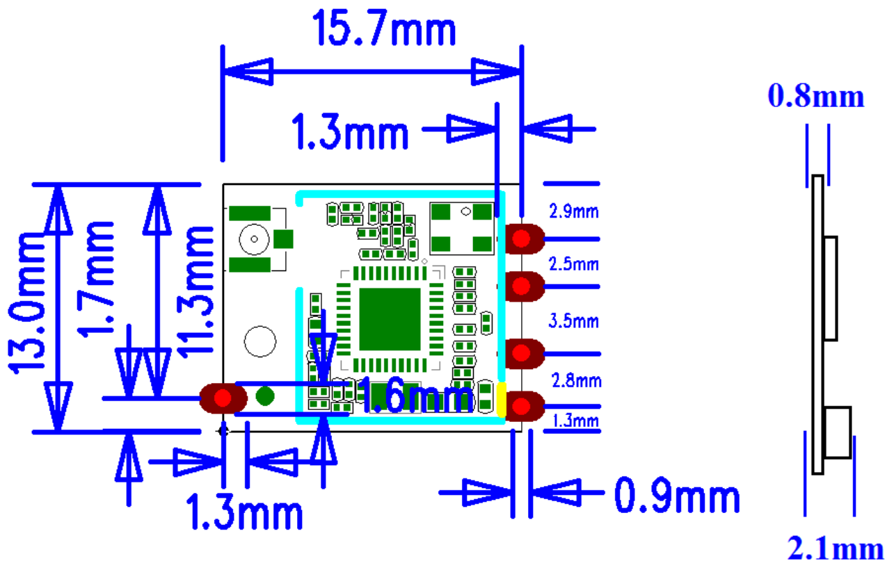
Figure 6 Module dimension
