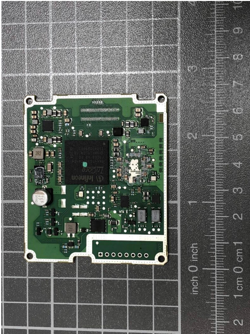
Variant 4, PCB, top view
