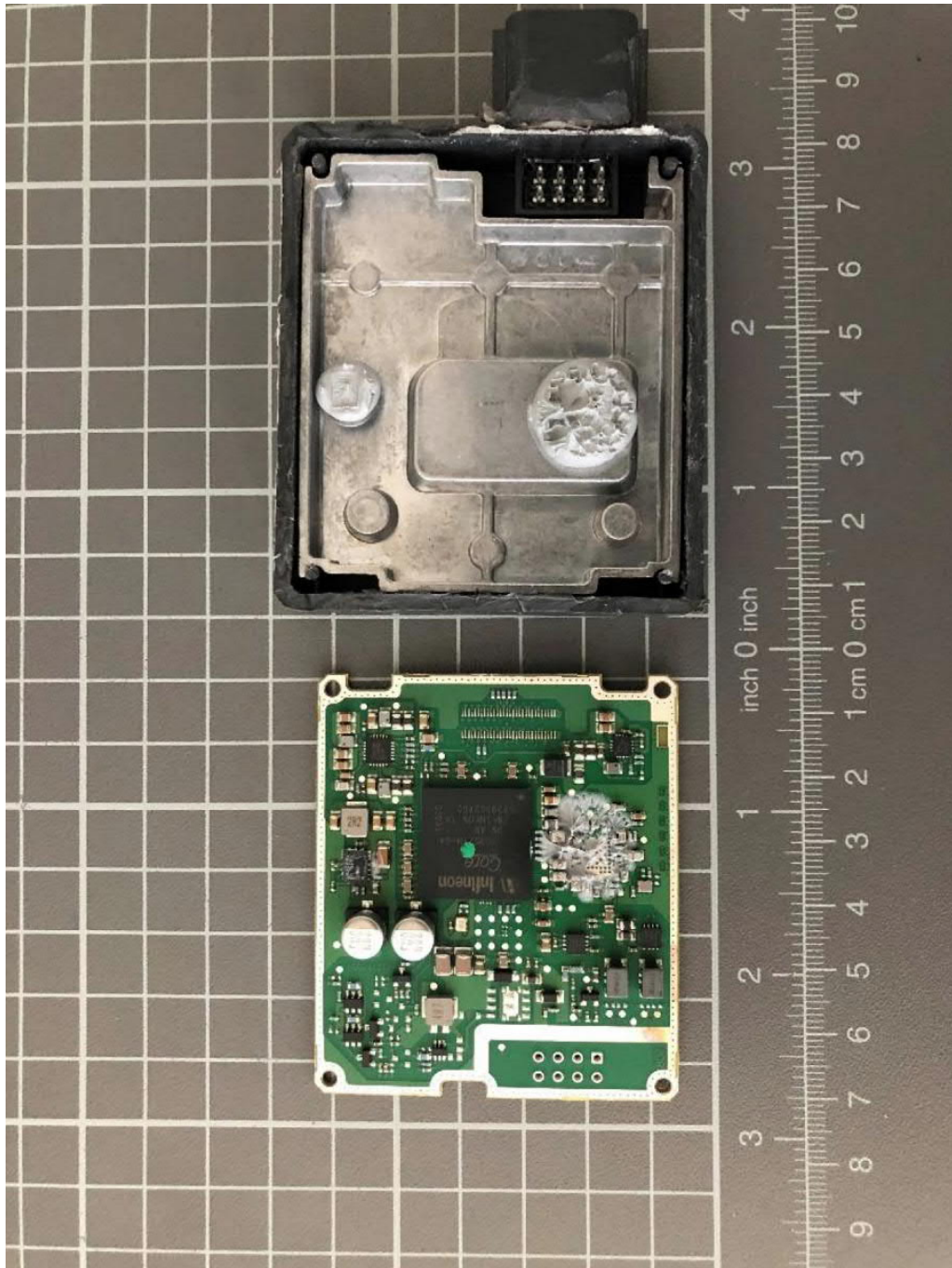
Variant 1, internal view 3
