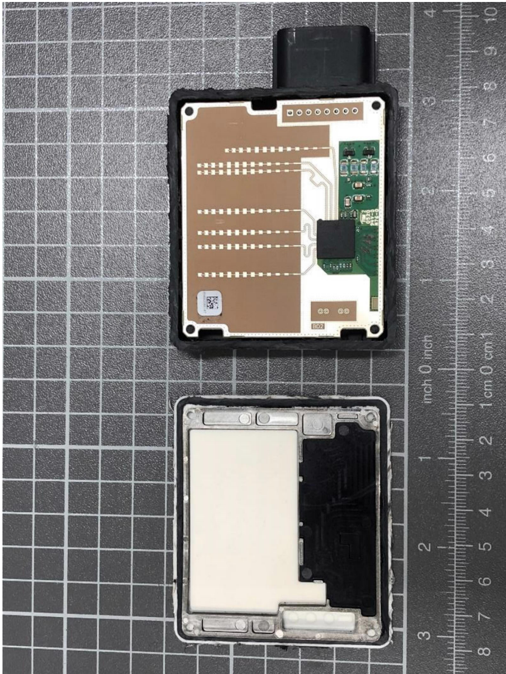
Variant 4, internal view 2
