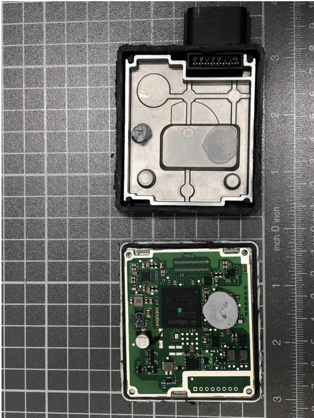
Variant 4, internal view 3
