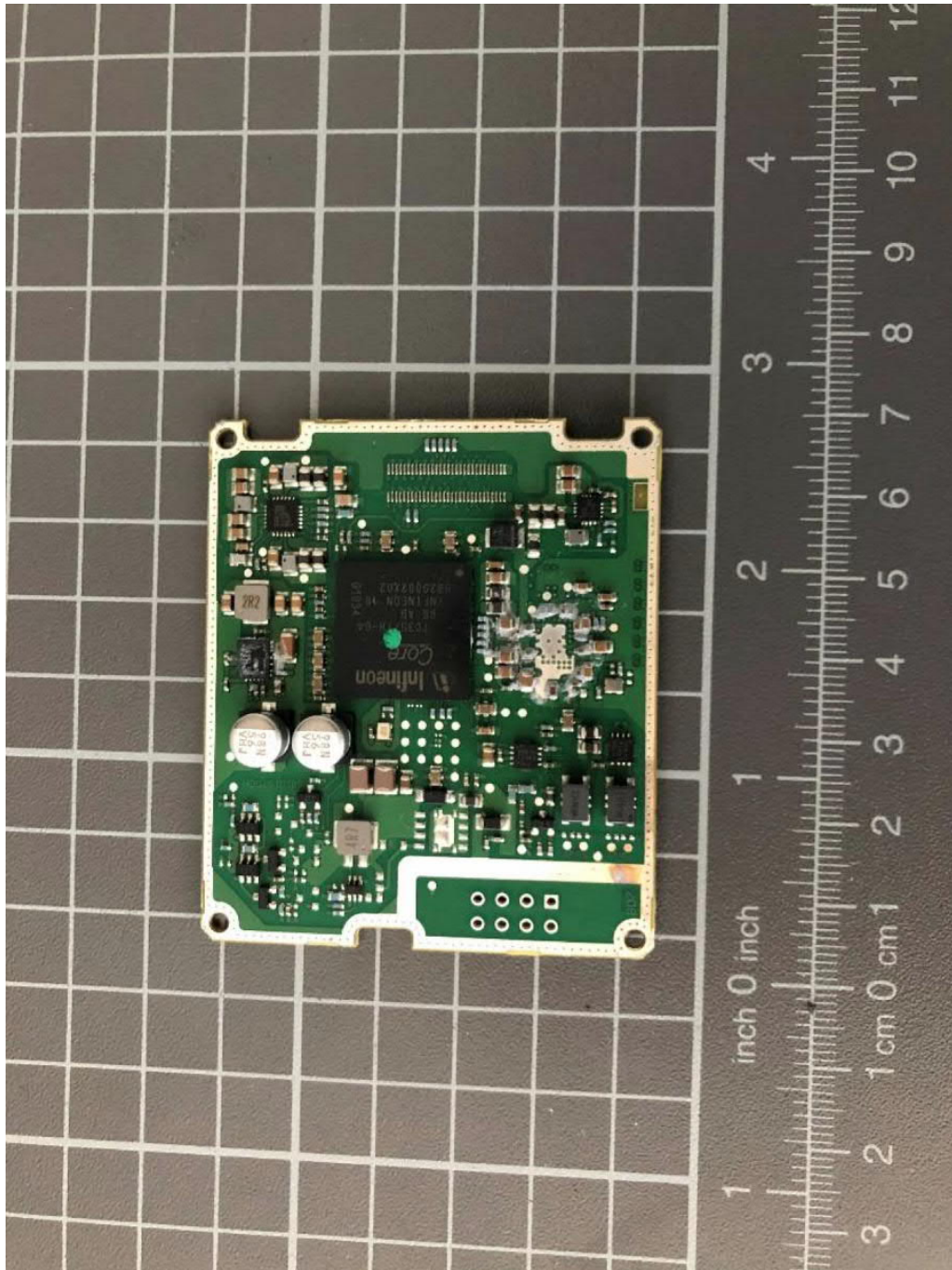
Variant 1, PCB, top view
