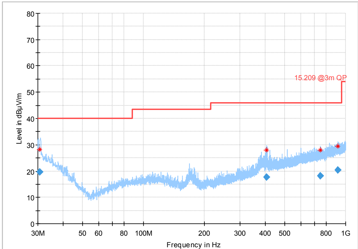
Plot no. 5: radiated emissions 30 MHz – 1 GHz, polarization vertical / horizontal
