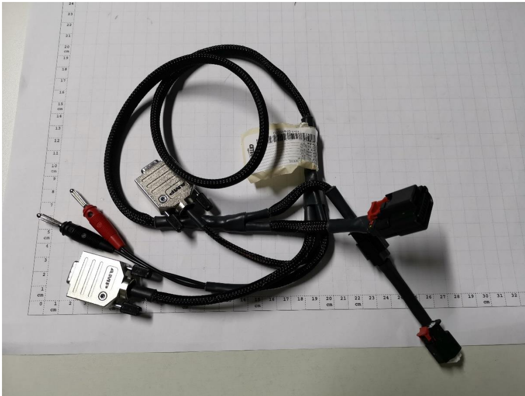
Photograph 7: Cables for power supply and CAN communication
