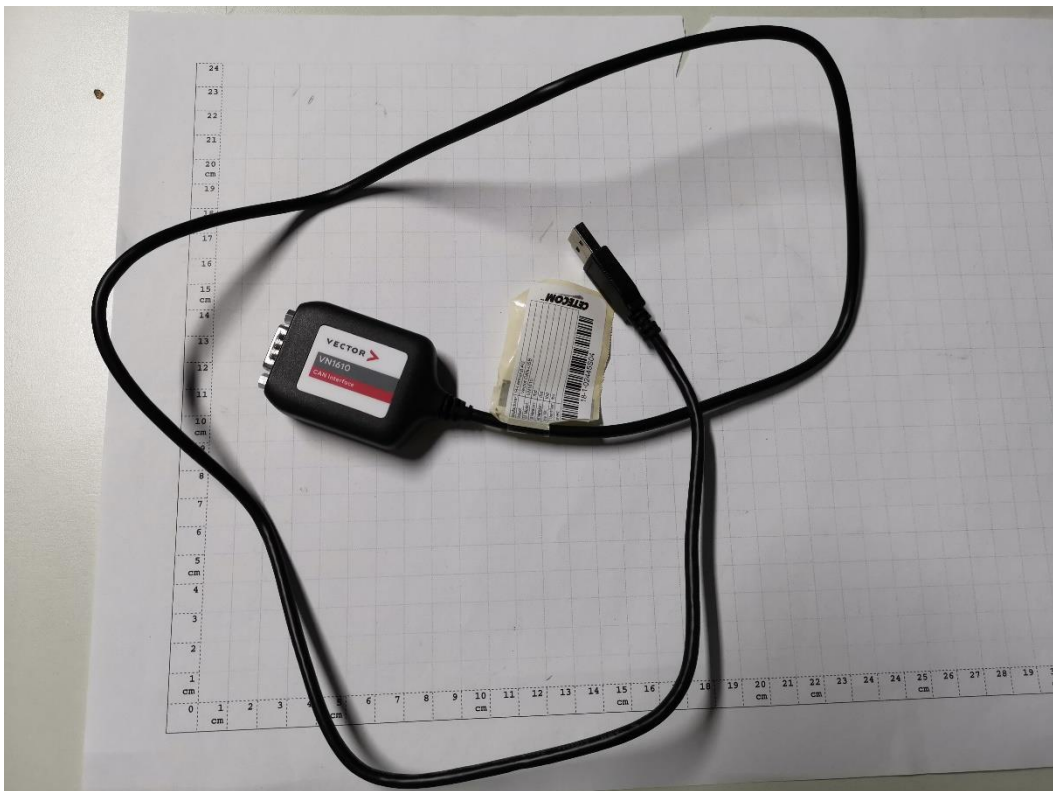
Photograph 8: CAN-USB converter
