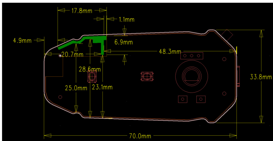
EUT Front View
