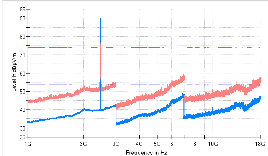
1GHz_18GHz_HP & VP_CH High
