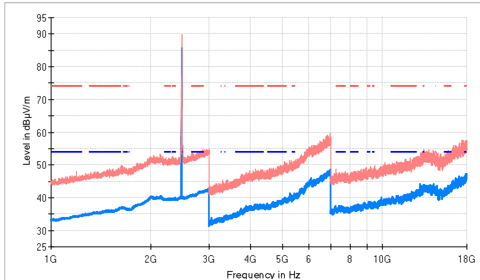
1GHz_18GHz_HP & VP_CH High
