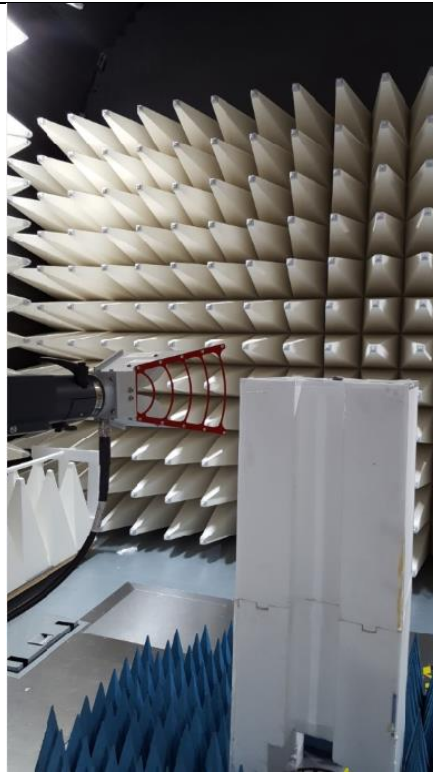
Figure B5. Radiated Setup HR
