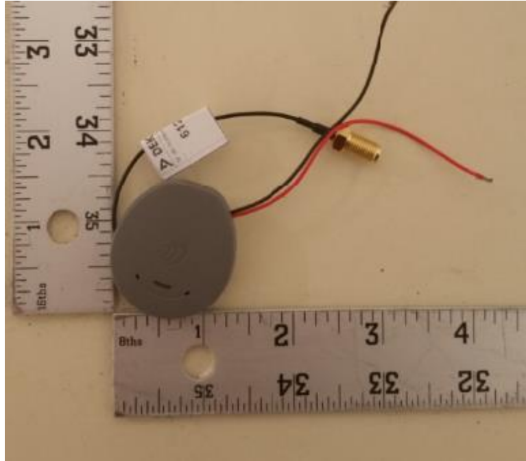
Figure B1. Conducted DUT Top View
