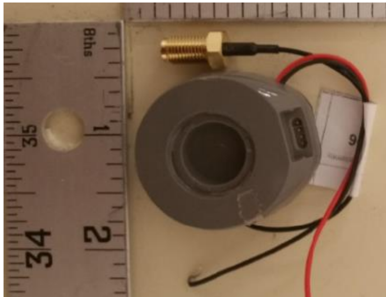
Figure B2. Conducted DUT Bottom View
