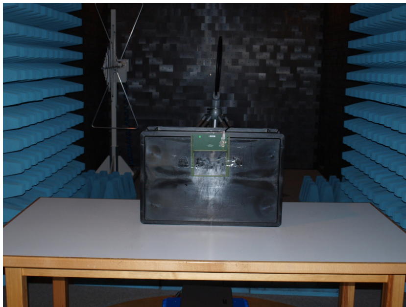
Picture 1-4: Occupied bandwidth test setup
