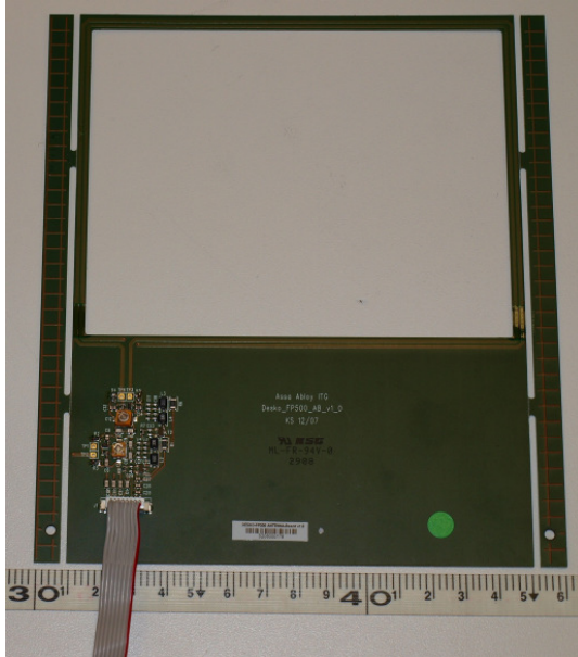
Picture 1-3: antenna board top side
