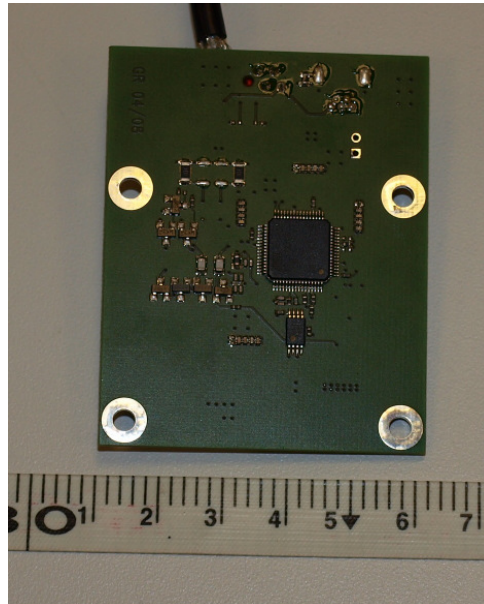
Picture 1-2: RFID 500 module bottom side
