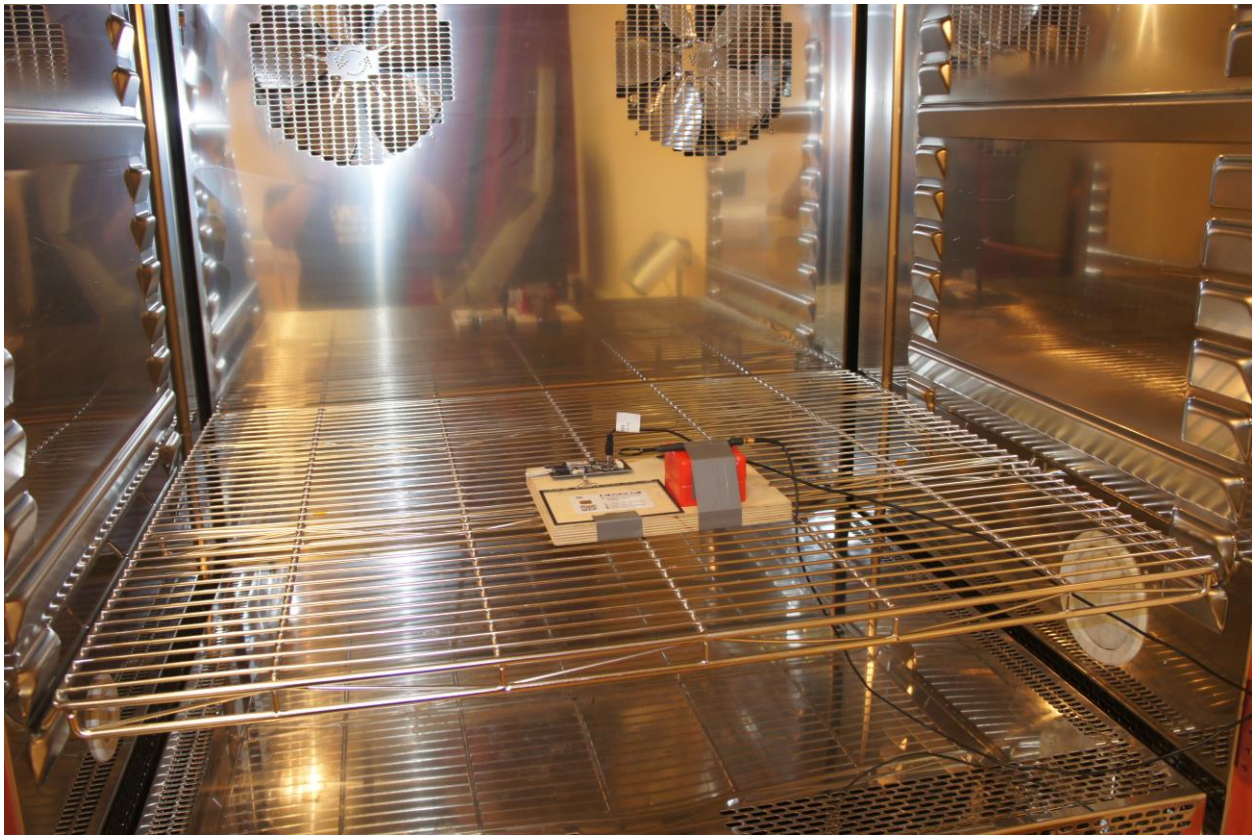
Picture 9: EUT test setup extreme conditions test
