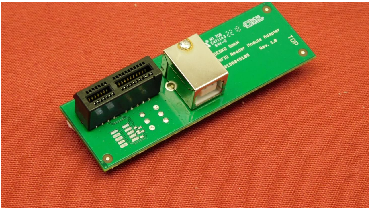
Picture 5: RFID reader module adapter top view
